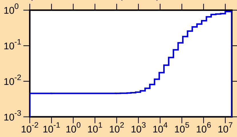
\mu vs. E for ^{150}\text{Nd}(\text{mt251})
