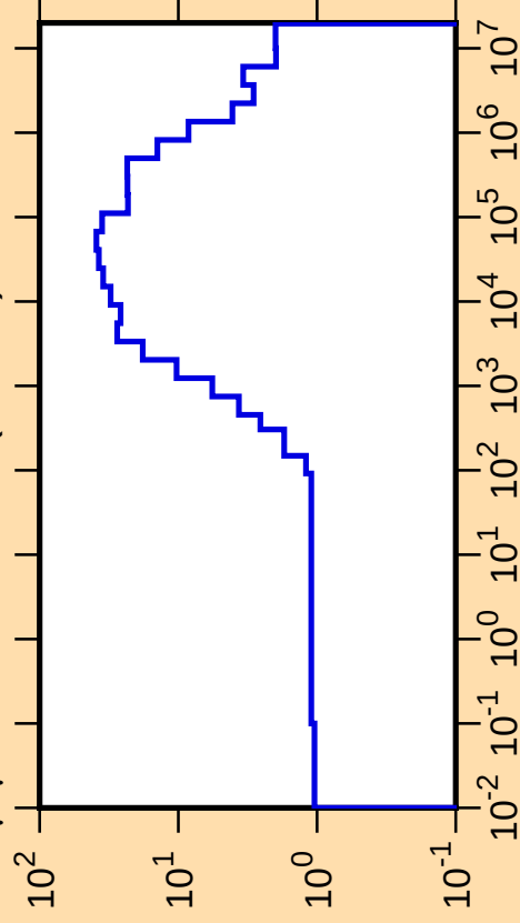
\Delta\mu/\mu vs. E for ^{150}\text{Nd}(\text{mt251})
