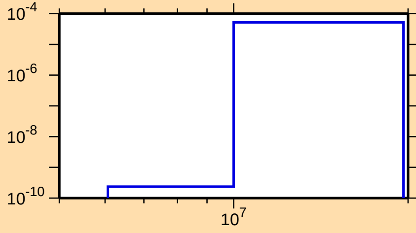
\sigma vs. E for ^{150}\text{Nd}(n,n\alpha)
