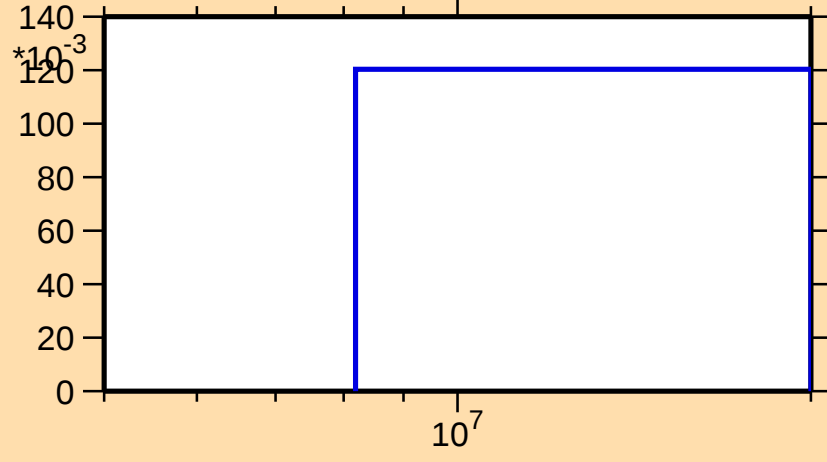
\sigma vs. E for ^{150}\text{Nd}(n,3n)
