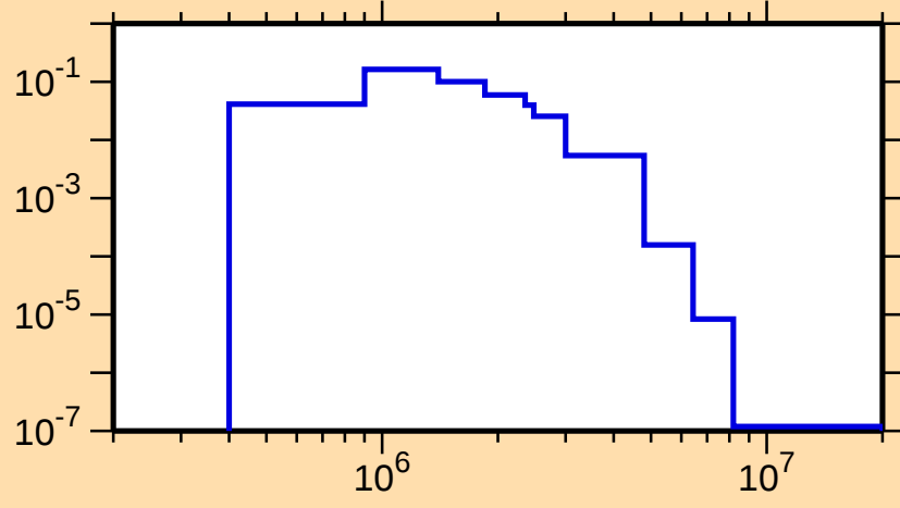
\sigma vs. E for ^{150}\text{Nd}(n,n_3)
