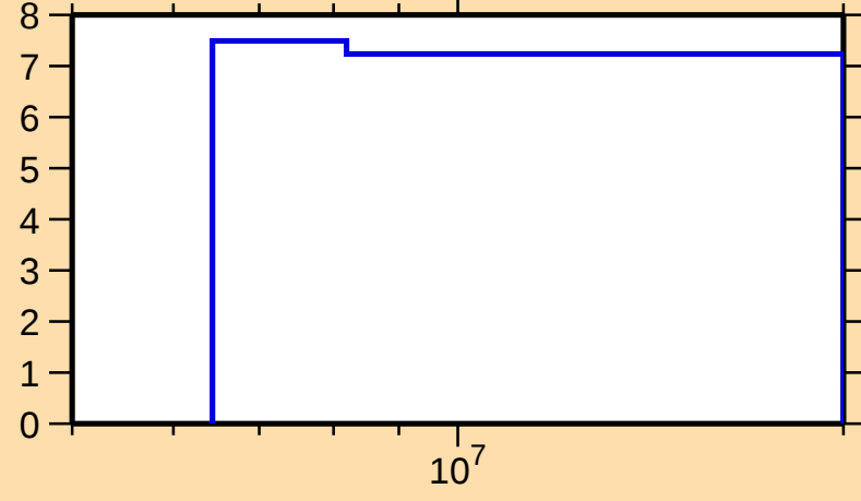
\Delta\sigma/\sigma vs. E for ^{150}\text{Nd}(n,2n)
