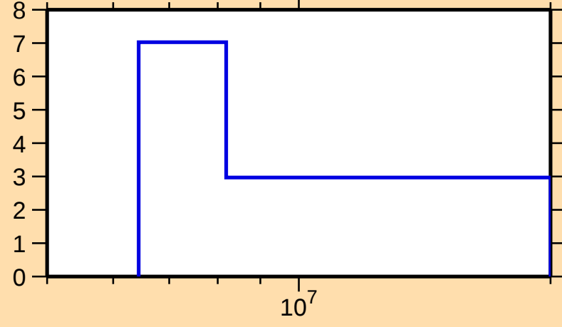
\Delta\sigma/\sigma vs. E for ^{150}\text{Nd}(n,\text{el.})
