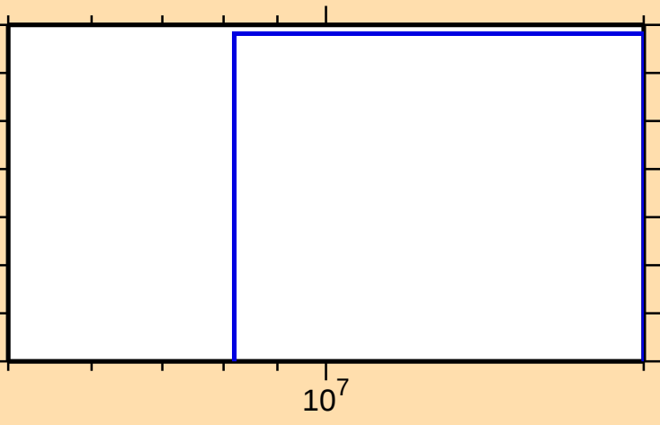
\sigma vs. E for ^{150}\text{Nd}(n,2n\alpha)
