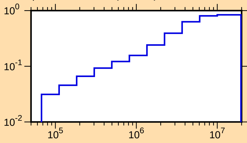
\mu vs. E for ^{66}\text{Ni}(\text{mt251})
