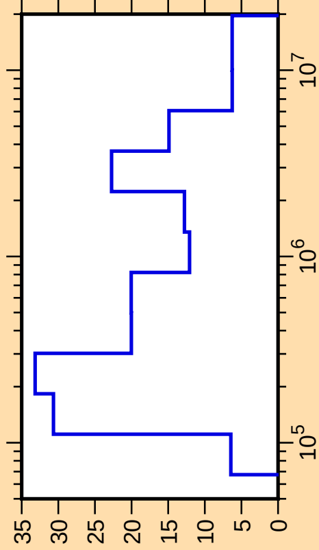
\Delta\mu/\mu vs. E for ^{66}\text{Ni}(\text{mt251})
