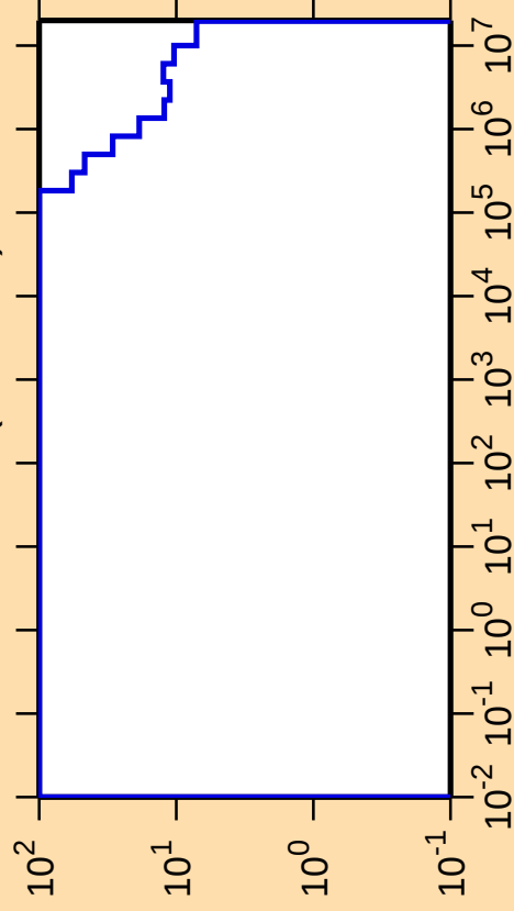
\Delta\sigma/\sigma vs. E for ^{251}\text{No}(n,\text{nonel.})
