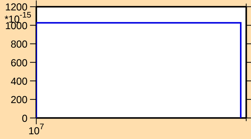
\sigma vs. E for ^{251}\text{No}(n,\text{pd})
