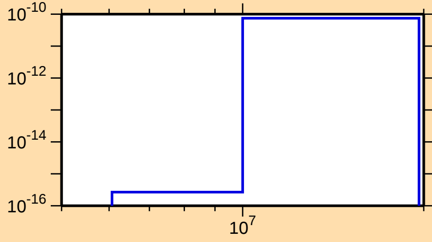
\sigma vs. E for ^{251}\text{No}(\text{mt117})
