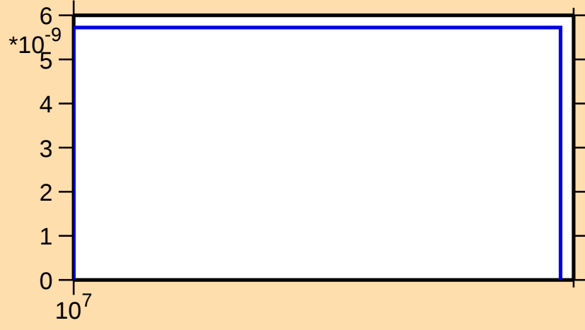
\sigma vs. E for ^{251}\text{No}(n,nt)
