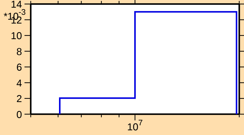
\sigma vs. E for ^{251}\text{No}(n,2n\alpha)
