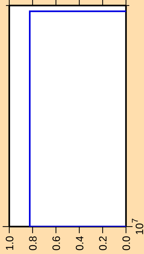
\Delta\sigma/\sigma vs. E for ^{251}\text{No}(n,\text{pd})
