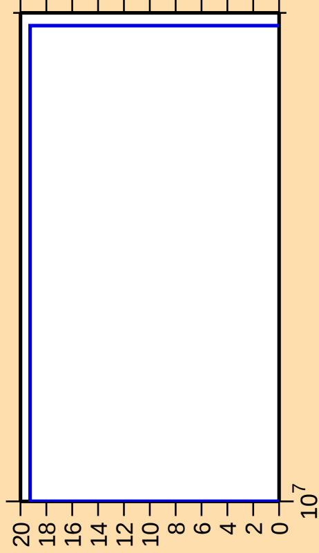
\Delta\sigma/\sigma vs. E for ^{251}\text{No}(n,\text{pt})
