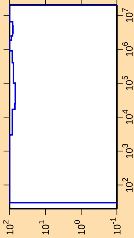
\Delta\sigma/\sigma vs. E for ^{251}\text{No}(n,\text{inel.})
