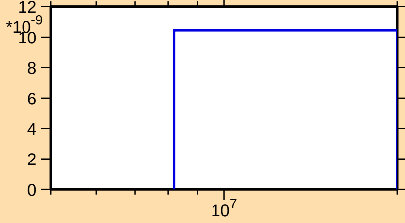
\sigma vs. E for ^{251}\text{No}(n,\text{He}3)
