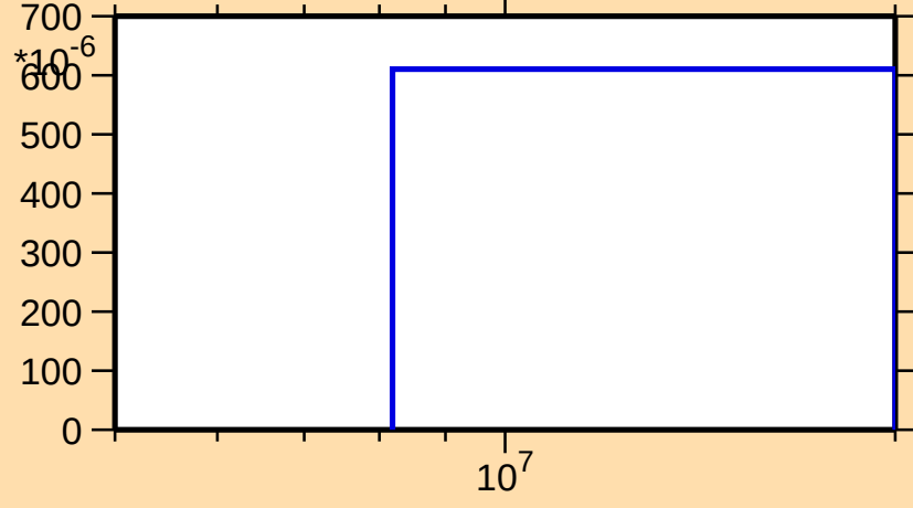
\sigma vs. E for ^{251}\text{No}(n,3n)
