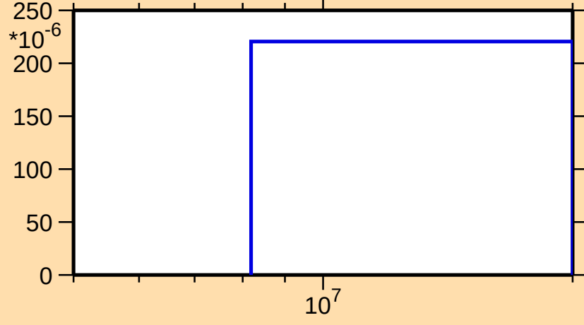
\sigma vs. E for ^{251}\text{No}(n,3n\alpha)
