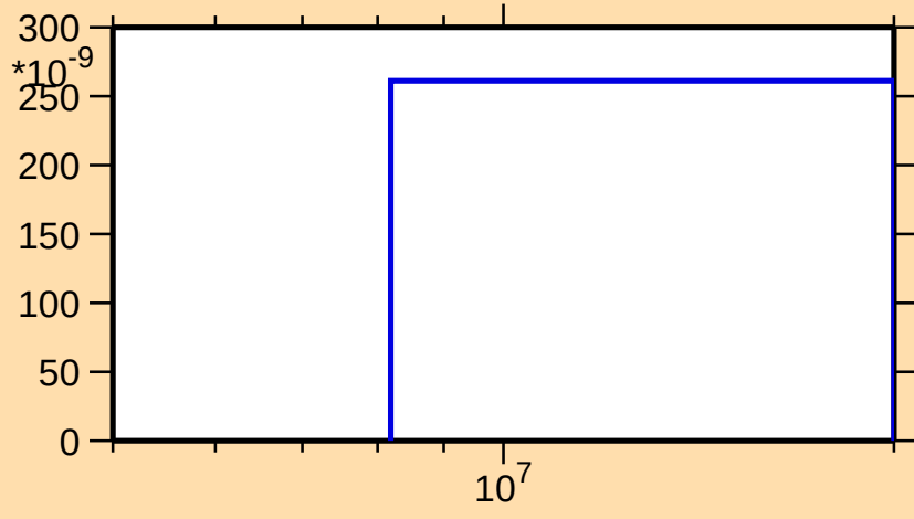
\sigma vs. E for ^{251}\text{No}(n,\text{nd})
