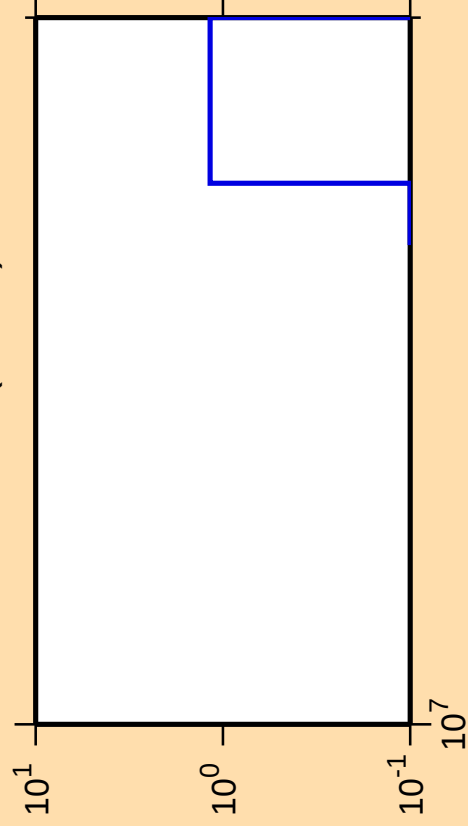
\Delta\sigma/\sigma vs. E for ^{264}\text{No}(n,\text{He3})
