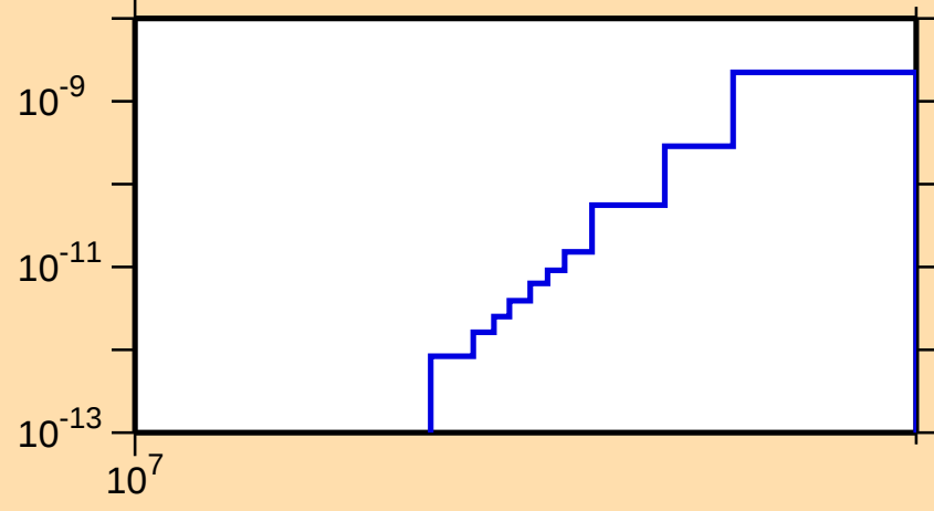
\sigma vs. E for ^{264}\text{No}(n,2n\alpha)
