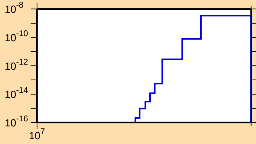
\sigma vs. E for ^{264}\text{No}(n,\text{nd})
