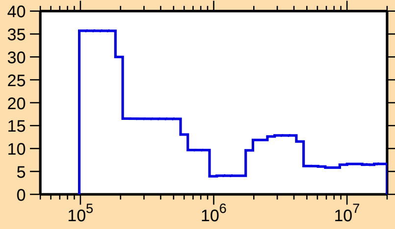
\Delta\sigma/\sigma vs. E for ^{264}\text{No}(n,\text{nonel.})
