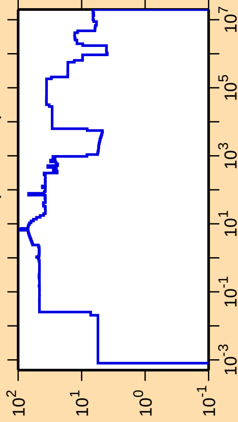
\Delta\sigma/\sigma vs. E for ^{264}\text{No}(n,\text{nonel.})
