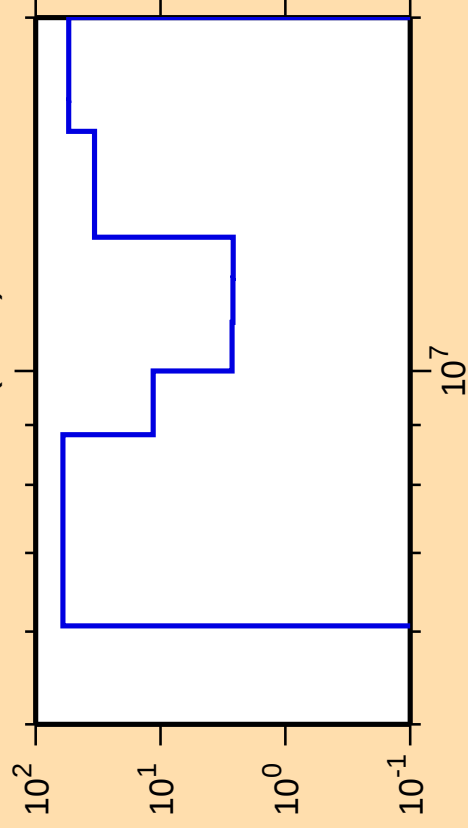
\Delta\sigma/\sigma vs. E for ^{264}\text{No}(n,2n)
