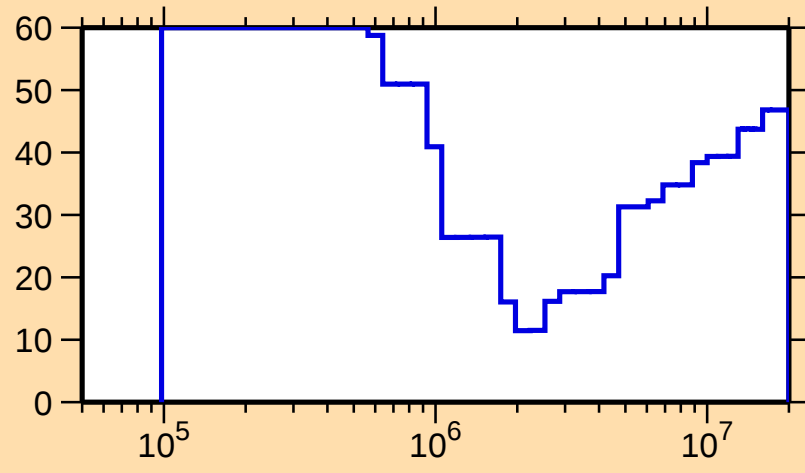
\Delta\sigma/\sigma vs. E for ^{264}\text{No}(n,n_1)
