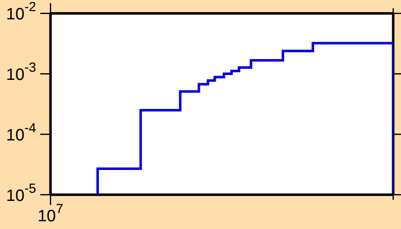
\sigma vs. E for ^{264}\text{No}(n,3n)
