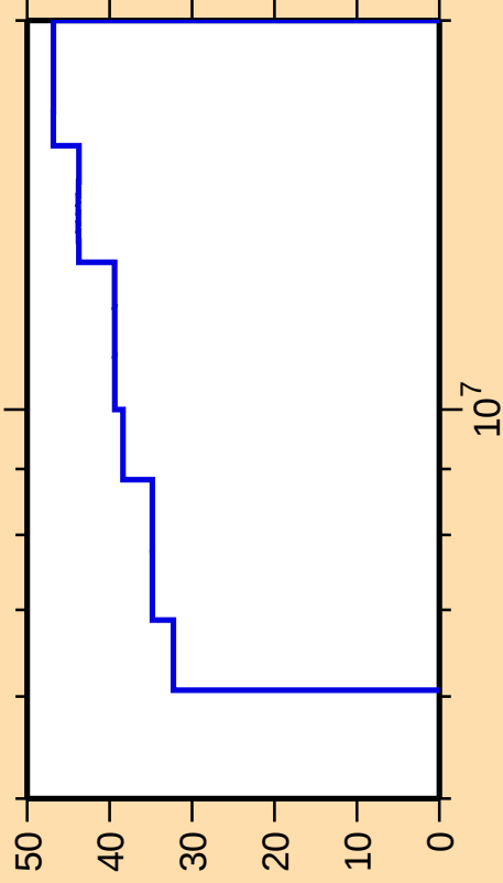
\Delta\sigma/\sigma vs. E for ^{264}\text{No}(n,n_1)
