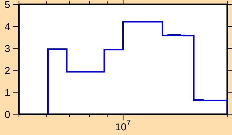
\Delta\sigma/\sigma vs. E for ^{264}\text{No}(n,\text{tot.})
