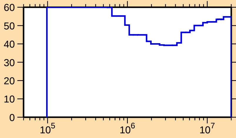
\Delta\sigma/\sigma vs. E for ^{264}\text{No}(n,\text{inel.})
