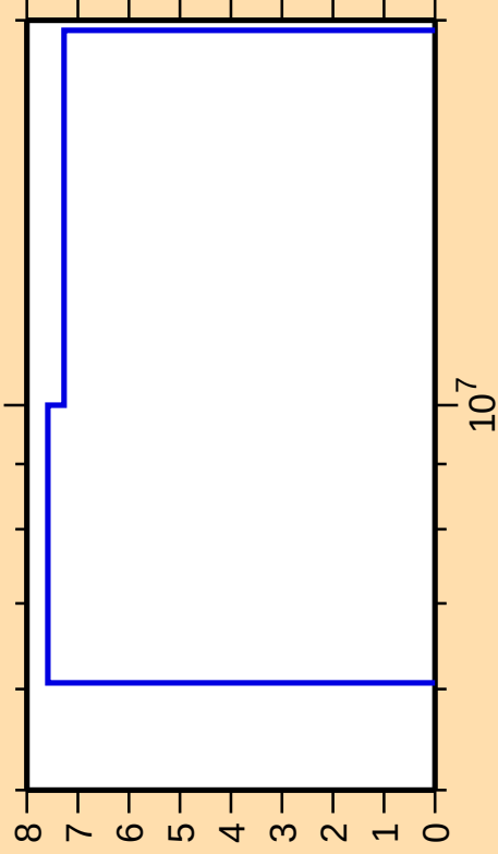
\Delta\sigma/\sigma vs. E for ^{264}\text{No}(n,f)
