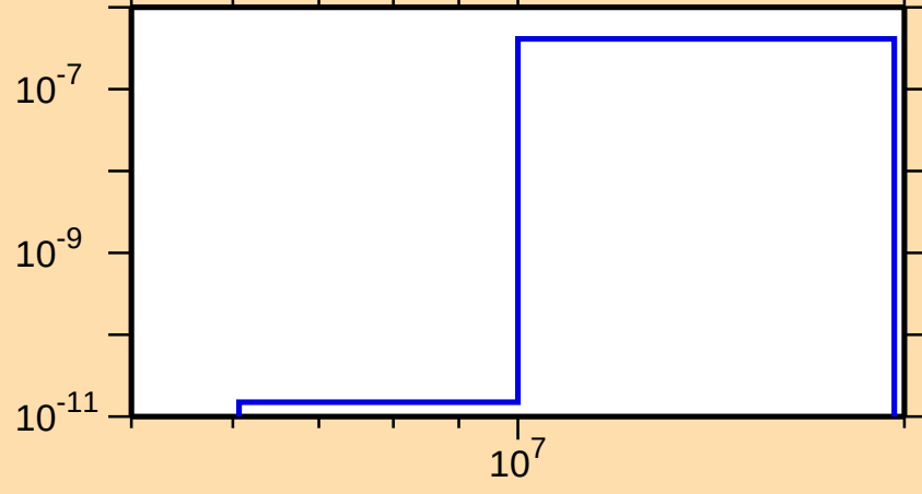
\sigma vs. E for ^{264}\text{No}(n,n\alpha)
