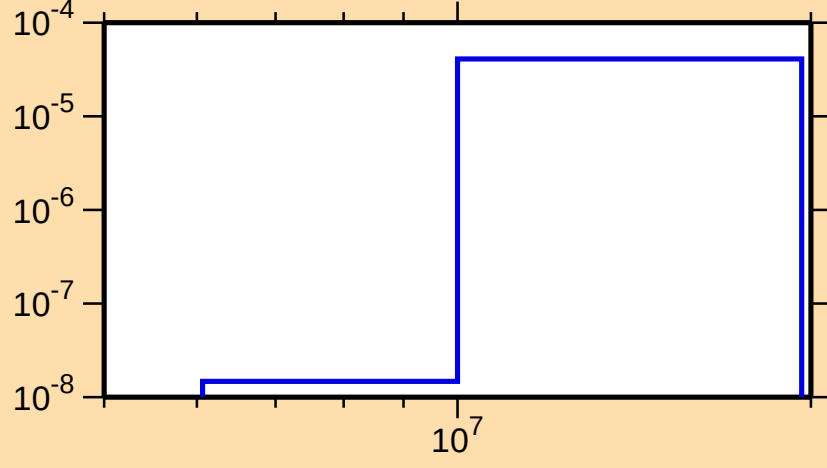
\sigma vs. E for ^{264}\text{No}(n,p)
