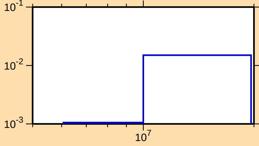
\sigma vs. E for ^{264}\text{No}(n,2n)
