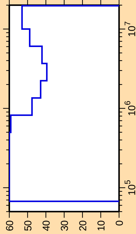
\Delta\sigma/\sigma vs. E for ^{264}\text{No}(n,\text{inel.})
