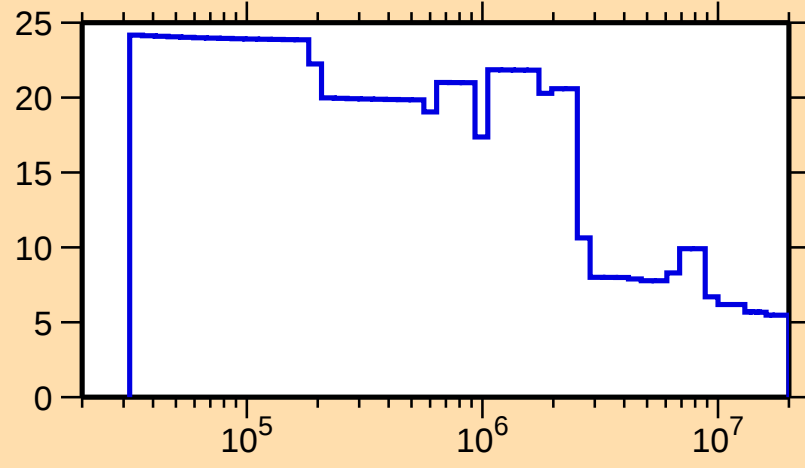
\Delta\sigma/\sigma vs. E for ^{235}\text{Np}(n,\text{nonel.})
