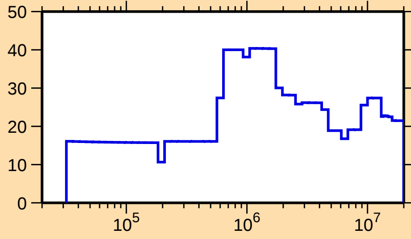
\Delta\sigma/\sigma vs. E for ^{235}\text{Np}(n,\text{el.})
