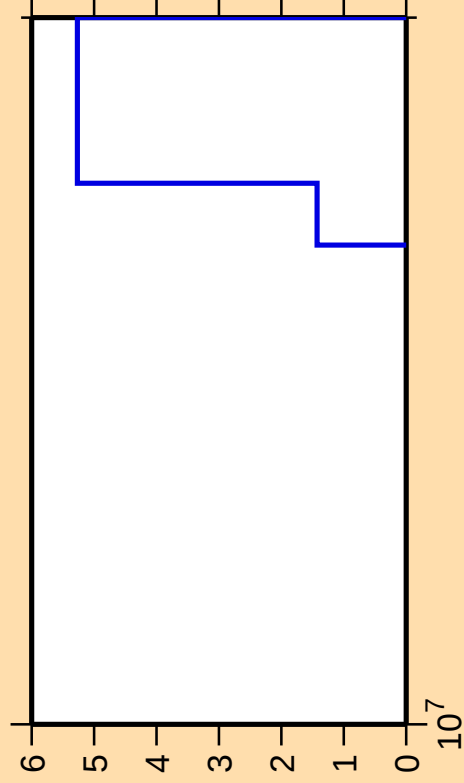
\Delta\sigma/\sigma vs. E for ^{235}\text{Np}(n,p\alpha)
