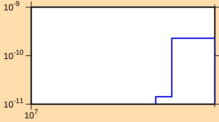
\sigma vs. E for ^{235}\text{Np}(n,\text{He3})
