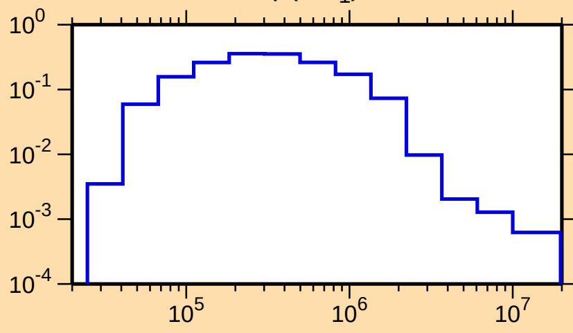
\sigma vs. E for ^{235}\text{Np}(n,n_1)
