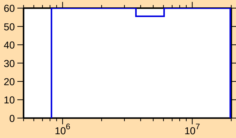
\Delta\sigma/\sigma vs. E for ^{235}\text{Np}(n,\text{inel.})
