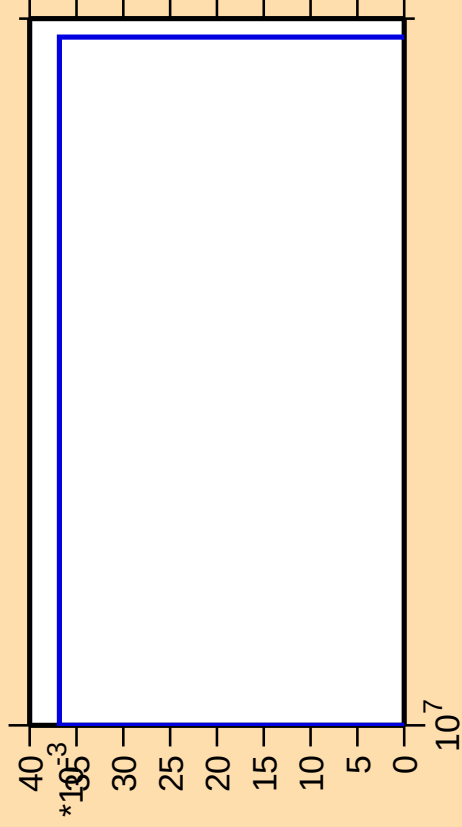
\Delta\sigma/\sigma vs. E for ^{235}\text{Np}(n,3n\alpha)
