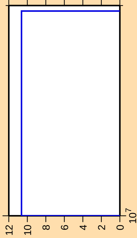
\Delta\sigma/\sigma vs. E for ^{235}\text{Np}(n,\text{He3})
