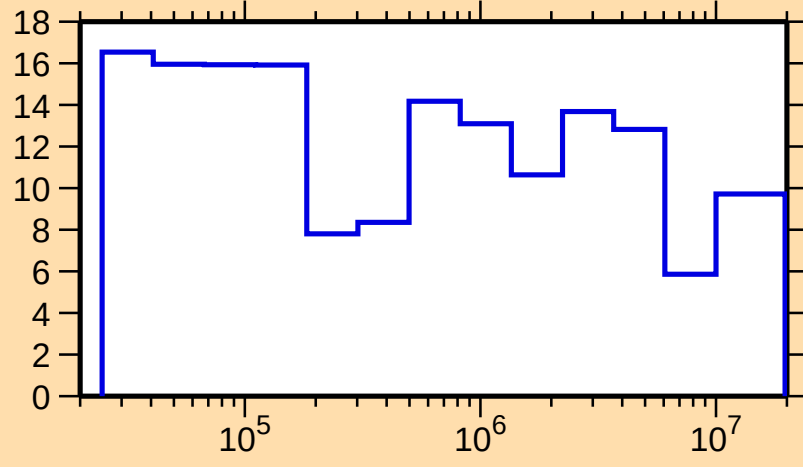
\Delta\sigma/\sigma vs. E for ^{235}\text{Np}(n,\text{tot.})
