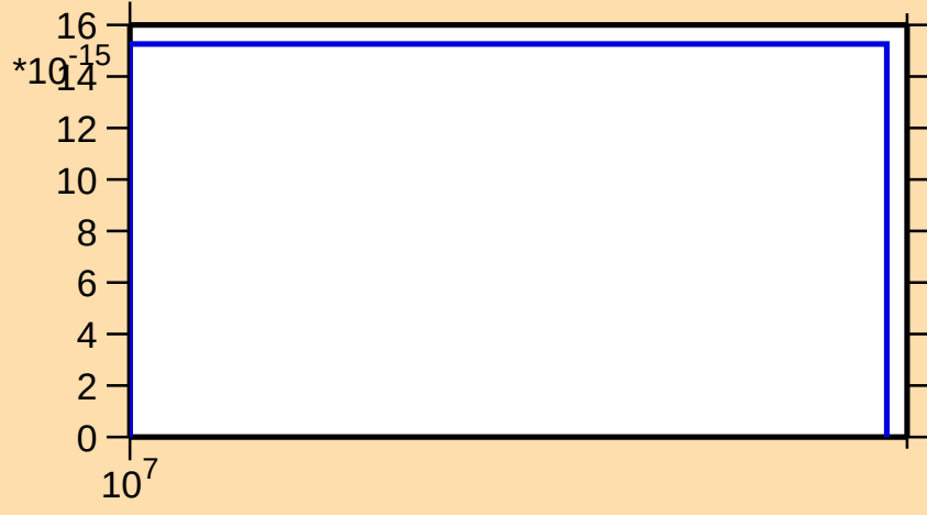
\sigma vs. E for ^{235}\text{Np}(n,3n\alpha)
