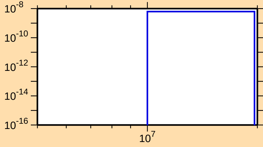
\sigma vs. E for ^{235}\text{Np}(n,2n\alpha)
