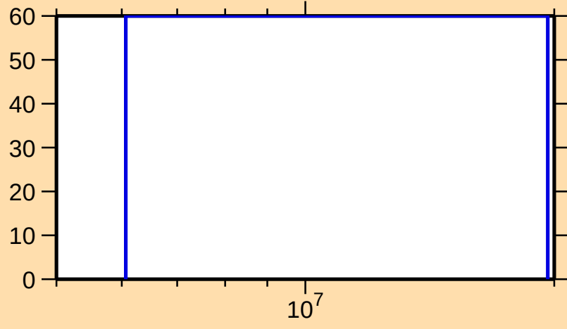
\Delta\sigma/\sigma vs. E for ^{235}\text{Np}(n,\text{inel.})
