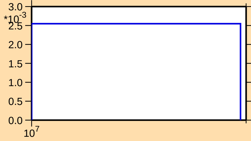
\sigma vs. E for ^{235}\text{Np}(n,3n)
