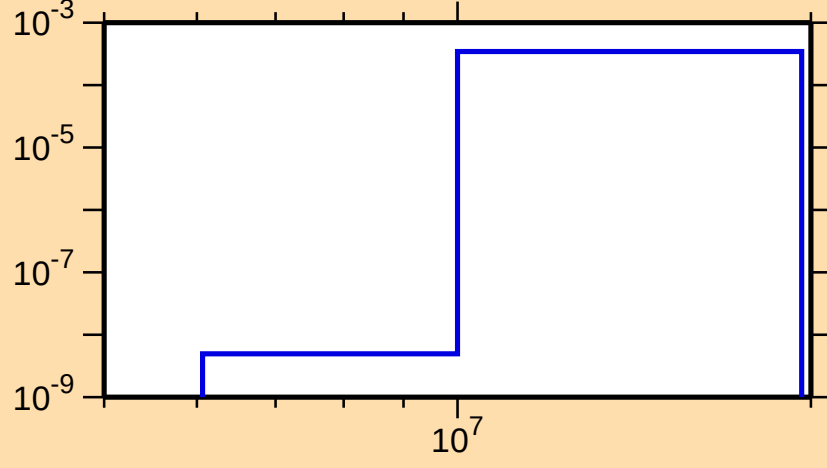
\sigma vs. E for ^{235}\text{Np}(n,d)
