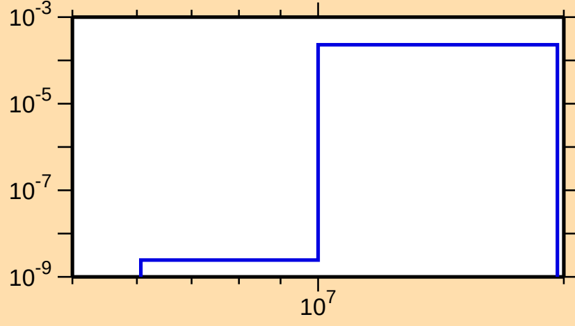
\sigma vs. E for ^{235}\text{Np}(n,np)
