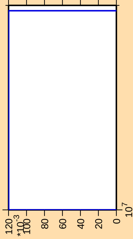
\Delta\sigma/\sigma vs. E for ^{235}\text{Np}(n,p\alpha)
