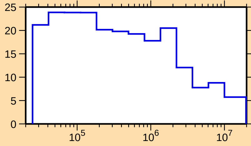
\Delta\sigma/\sigma vs. E for ^{235}\text{Np}(n,\text{nonel.})
