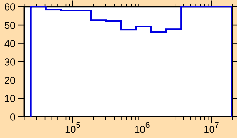
\Delta\sigma/\sigma vs. E for ^{235}\text{Np}(n,n_1)
