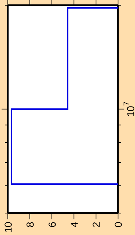
\Delta\sigma/\sigma vs. E for ^{235}\text{Np}(n,f)
