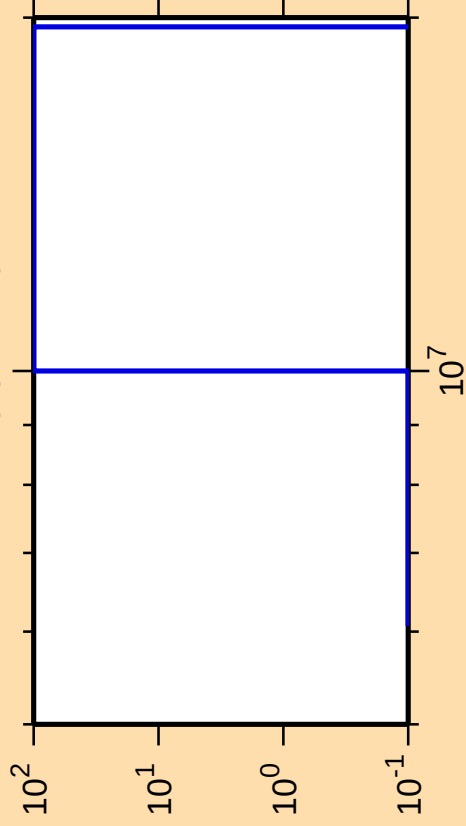
\Delta\sigma/\sigma vs. E for ^{235}\text{Np}(n,2n\alpha)
