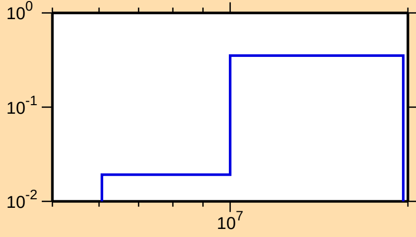
\sigma vs. E for ^{235}\text{Np}(n,2n)
