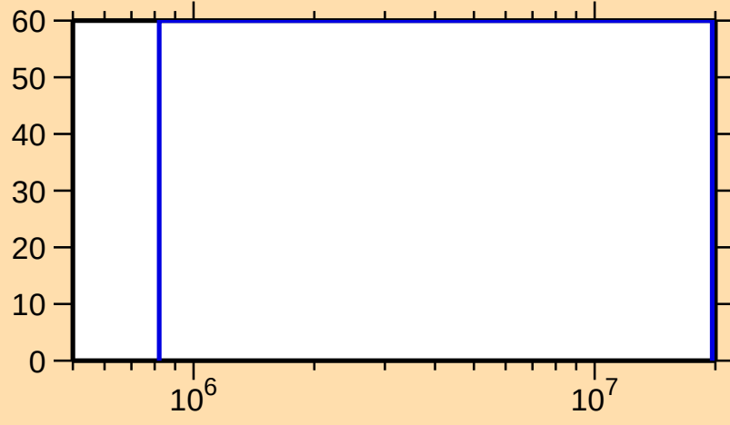
\Delta\sigma/\sigma vs. E for ^{235}\text{Np}(n,n\text{cont.})
