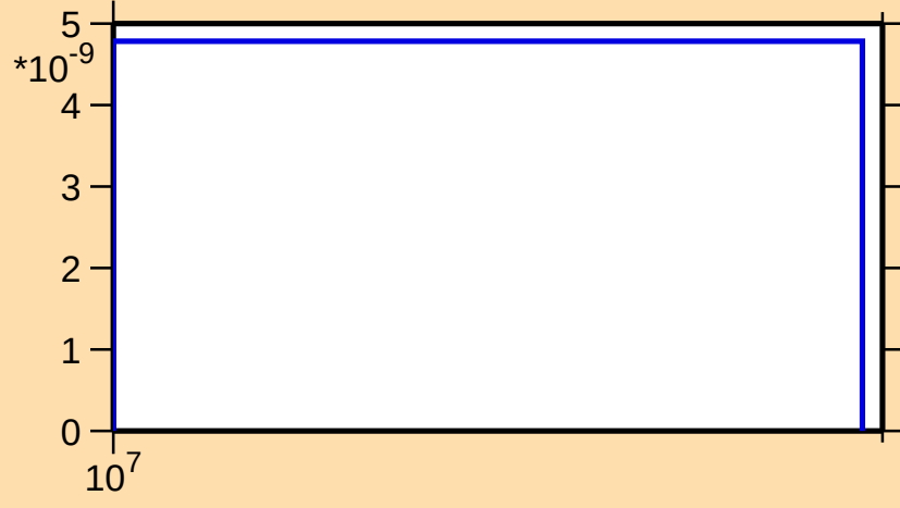
\sigma vs. E for ^{235}\text{Np}(n,nt)
