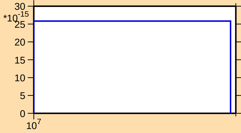
\sigma vs. E for ^{235}\text{Np}(n,p\alpha)
