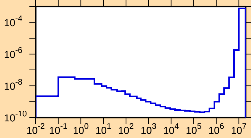
\sigma vs. E for ^{235}\text{Np}(n,\alpha)
