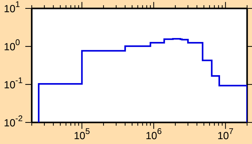
\sigma vs. E for ^{235}\text{Np}(n,\text{inel.})
