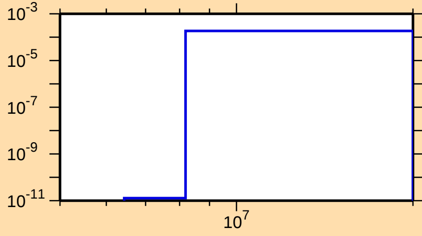
\sigma vs. E for ^{235}\text{Np}(n,np)
