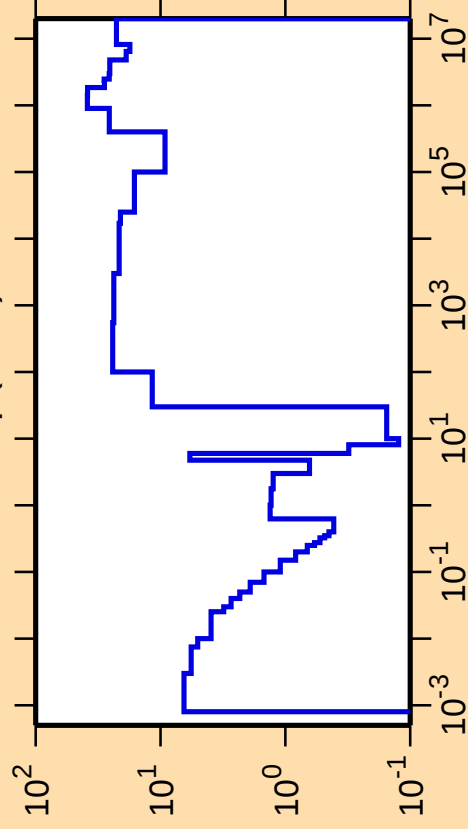
\Delta\sigma/\sigma vs. E for ^{235}\text{Np}(n,\text{el.})
