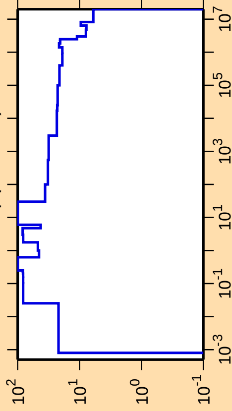
\Delta\sigma/\sigma vs. E for ^{235}\text{Np}(n,\text{nonel.})
