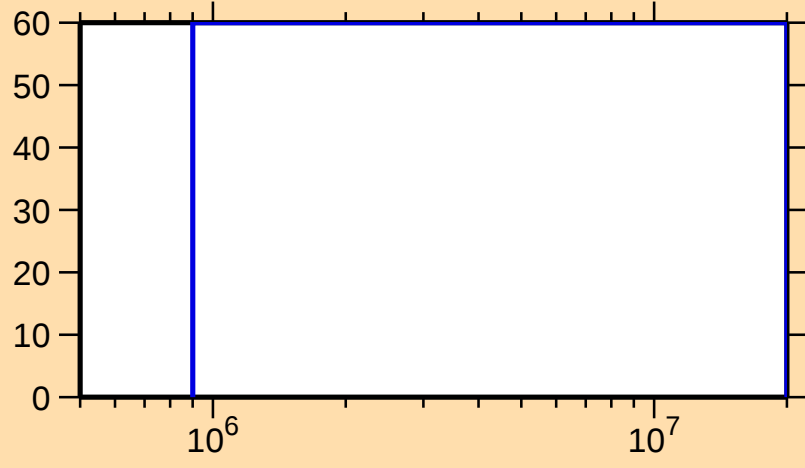
\Delta\sigma/\sigma vs. E for ^{235}\text{Np}(n,n\text{cont.})
