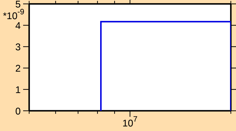
\sigma vs. E for ^{235}\text{Np}(n,nt)
