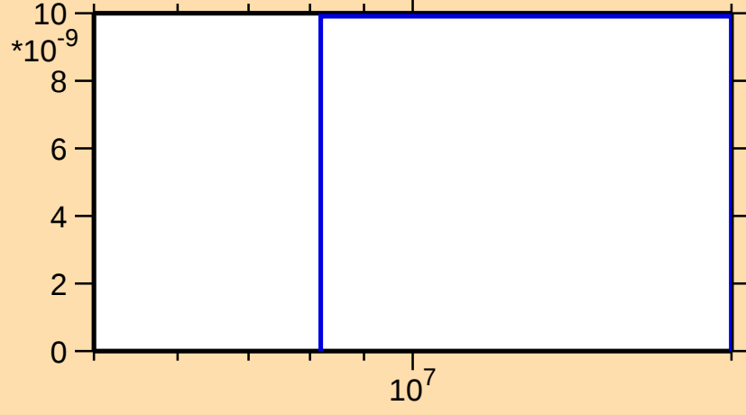
\sigma vs. E for ^{235}\text{Np}(n,\text{nd})
