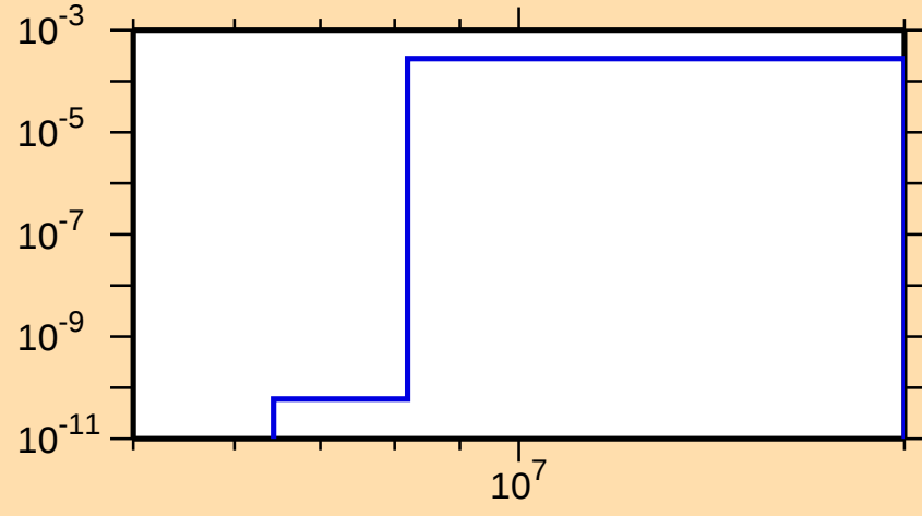
\sigma vs. E for ^{235}\text{Np}(n,d)
