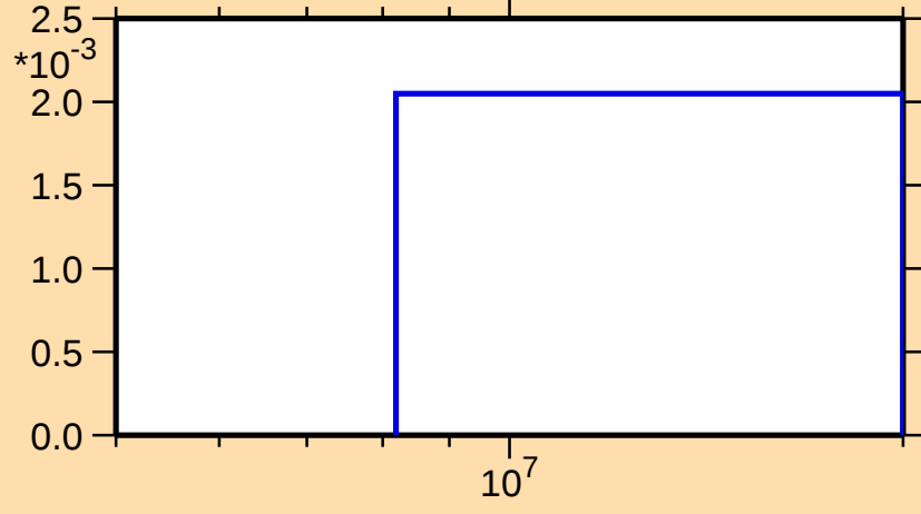
\sigma vs. E for ^{235}\text{Np}(n,3n)
