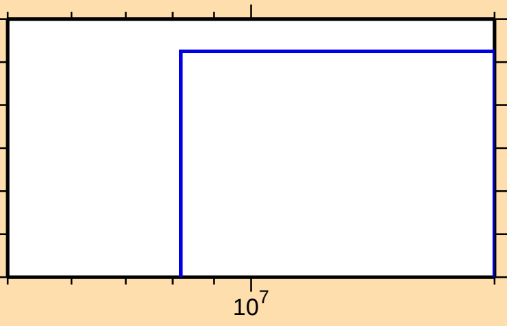
\sigma vs. E for ^{235}\text{Np}(n,2n\alpha)
