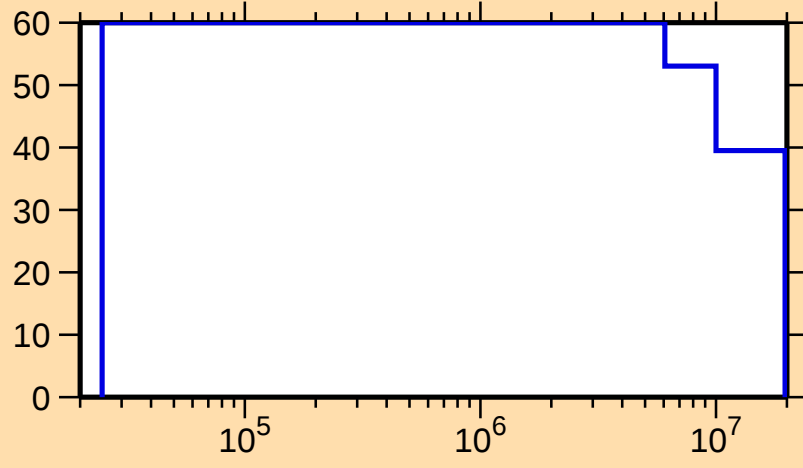
\Delta\sigma/\sigma vs. E for ^{239}\text{Np}(n,\text{inel.})
