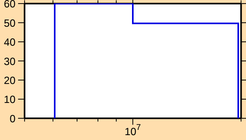
\Delta\sigma/\sigma vs. E for ^{239}\text{Np}(n,2n)
