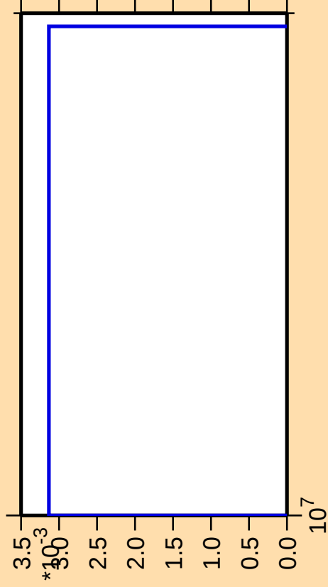
\Delta\sigma/\sigma vs. E for ^{239}\text{Np} (mt 11)
