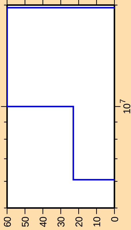
\Delta\sigma/\sigma vs. E for ^{239}\text{Np}(n,np)
