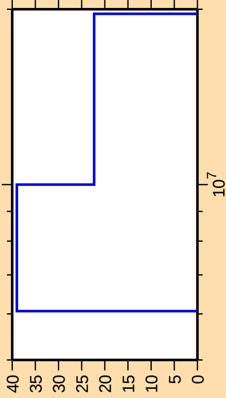
\Delta\sigma/\sigma vs. E for ^{239}\text{Np}(n,f)
