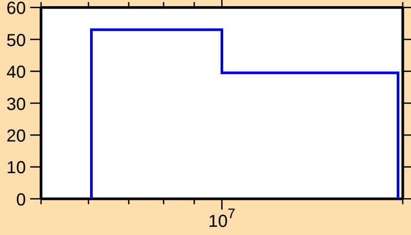
\Delta\sigma/\sigma vs. E for ^{239}\text{Np}(n,\text{inel.})
