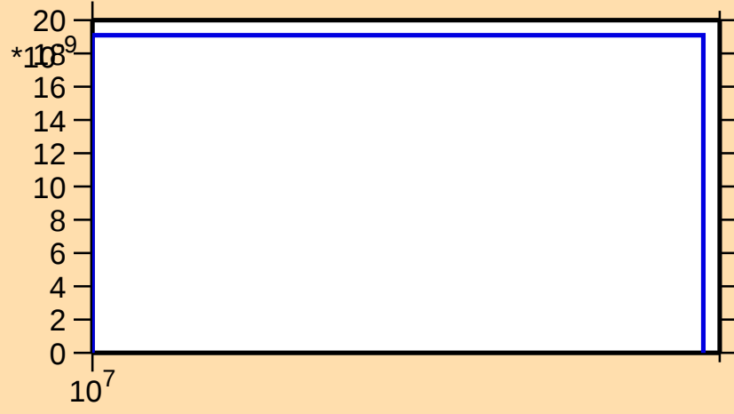
\sigma vs. E for ^{239}\text{Np}(n,\text{nd})
