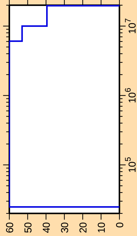
\Delta\sigma/\sigma vs. E for ^{239}\text{Np}(n,\text{inel.})
