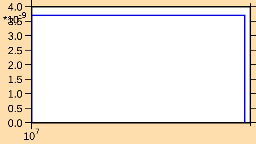
\sigma vs. E for ^{239}\text{Np}(n,2np)
