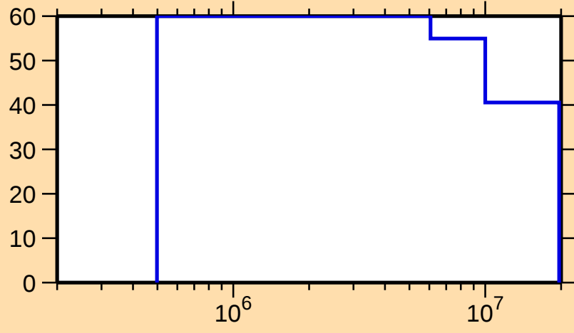
\Delta\sigma/\sigma vs. E for ^{239}\text{Np}(n,n\text{cont.})
