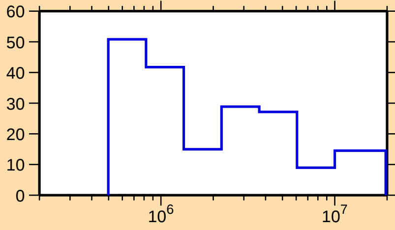
\Delta\sigma/\sigma vs. E for ^{239}\text{Np}(n,\text{el.})
