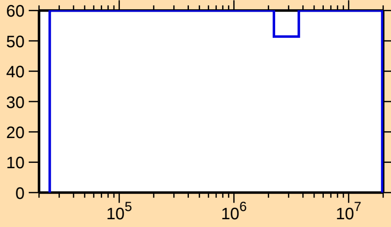
\Delta\sigma/\sigma vs. E for ^{239}\text{Np}(n,n_1)
