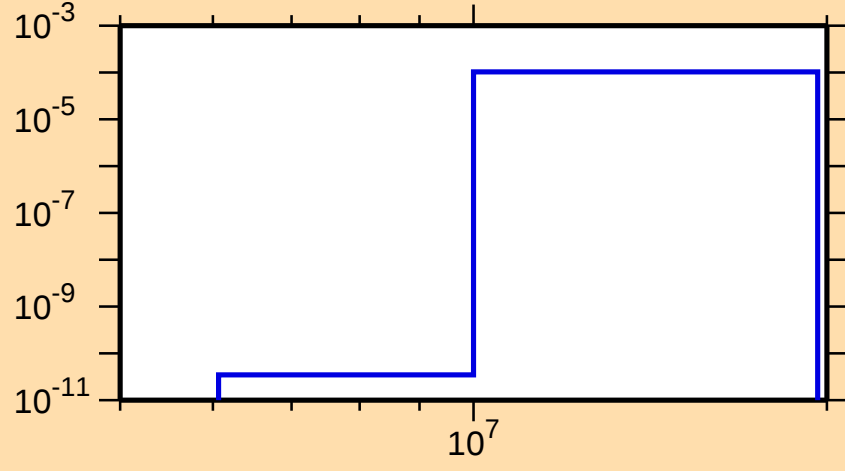
\sigma vs. E for ^{239}\text{Np}(n,np)
