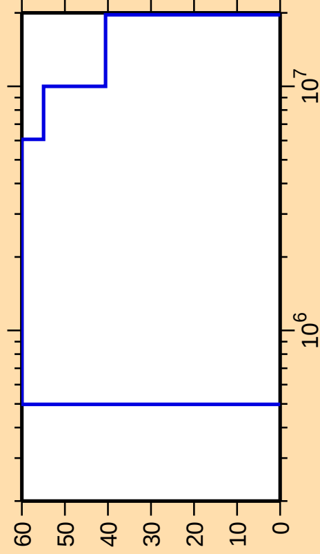
\Delta\sigma/\sigma vs. E for ^{239}\text{Np}(n,\text{ncont.})
