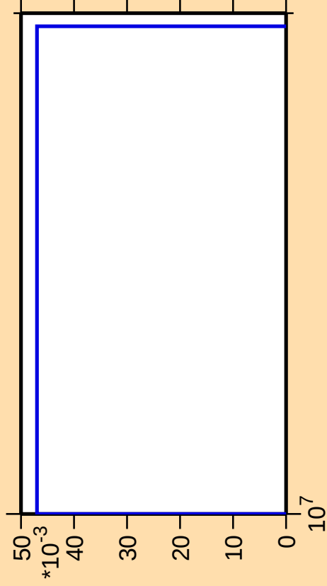
\Delta\sigma/\sigma vs. E for ^{239}\text{Np}(n,3n\alpha)
