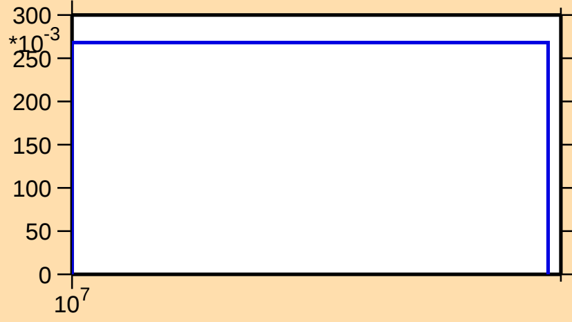
\sigma vs. E for ^{239}\text{Np}(n,3n)
