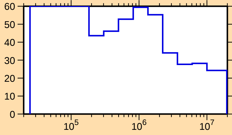
\Delta\sigma/\sigma vs. E for ^{239}\text{Np}(n,\text{nonel.})
