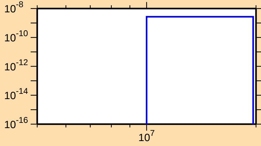
\sigma vs. E for ^{239}\text{Np}(n,2n\alpha)
