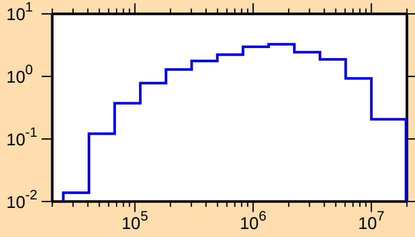
\sigma vs. E for ^{239}\text{Np}(n,\text{inel.})
