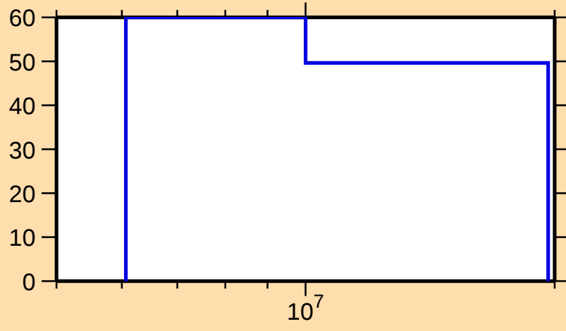
\Delta\sigma/\sigma vs. E for ^{239}\text{Np}(n,2n)
