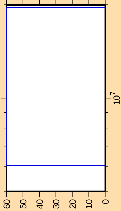
\Delta\sigma/\sigma vs. E for ^{239}\text{Np}(n,p)
