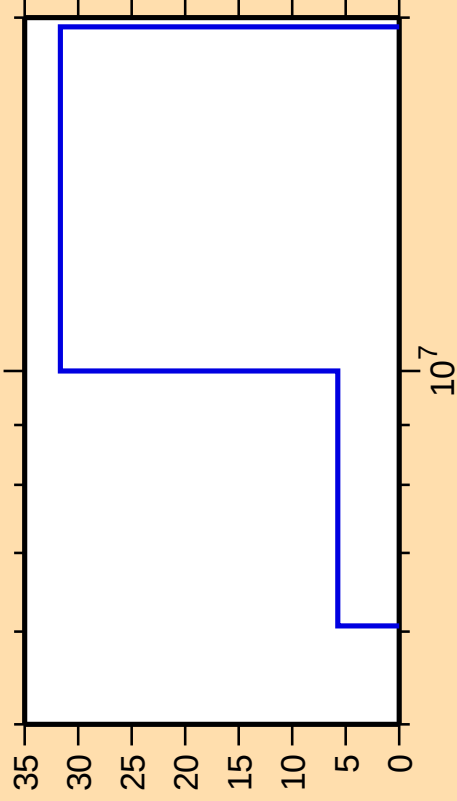
\Delta\sigma/\sigma vs. E for ^{239}\text{Np}(n,t)
