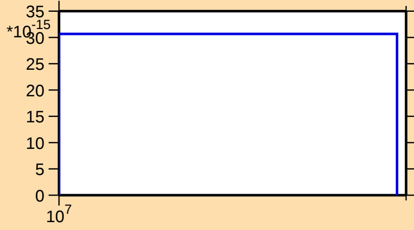
\sigma vs. E for ^{239}\text{Np}(n,\text{He3})
