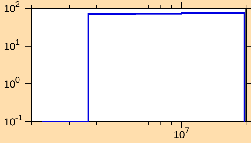
\Delta\sigma/\sigma vs. E for ^{239}\text{Np}(n,p)
