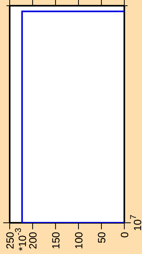
\Delta\sigma/\sigma vs. E for ^{239}\text{Np}(n,\text{He3})
