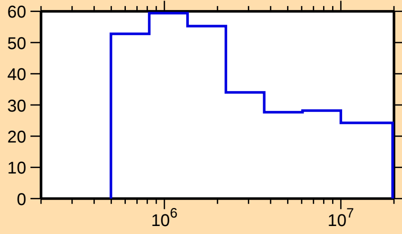
\Delta\sigma/\sigma vs. E for ^{239}\text{Np}(n,n\text{nonel.})
