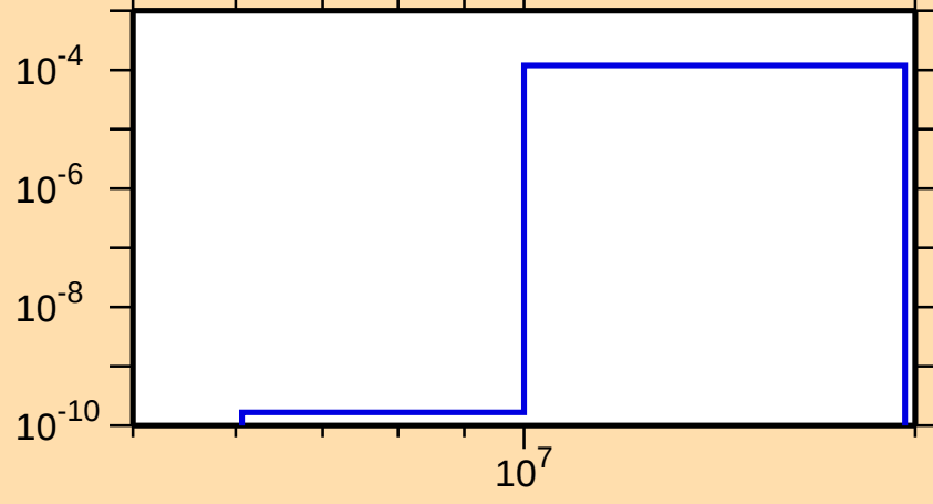
\sigma vs. E for ^{239}\text{Np}(n,d)
