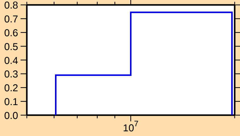
\sigma vs. E for ^{239}\text{Np}(n,2n)
