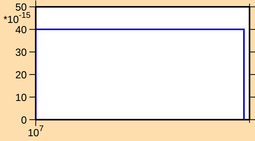
\sigma vs. E for ^{239}\text{Np}(n,3n\alpha)
