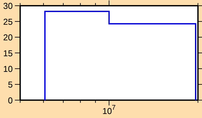
\Delta\sigma/\sigma vs. E for ^{239}\text{Np}(n,\text{nonel.})
