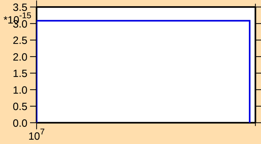
\sigma vs. E for ^{239}\text{Np} (mt 11)
