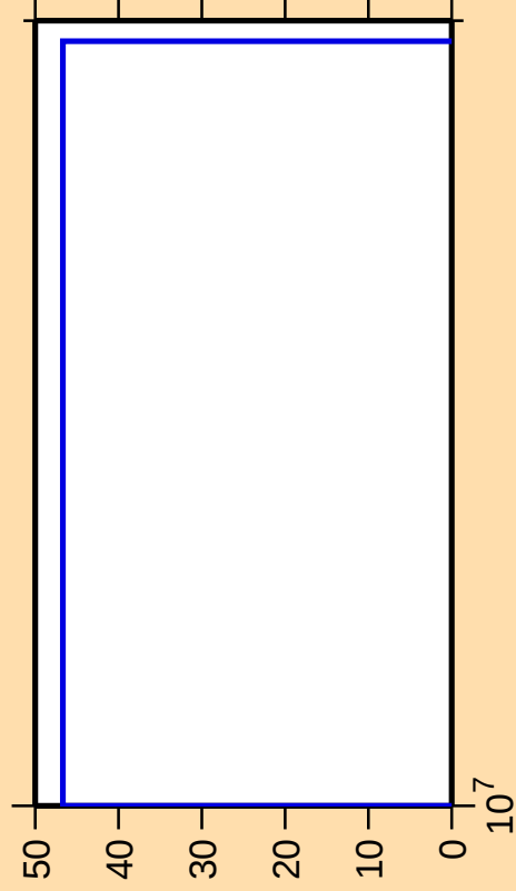
\Delta\sigma/\sigma vs. E for ^{239}\text{Np}(n,\text{nd})
