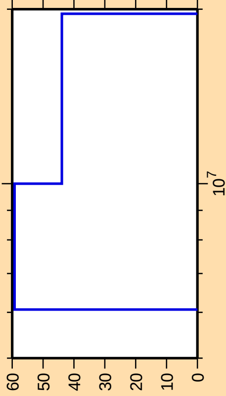
\Delta\sigma/\sigma vs. E for ^{239}\text{Np}(n,d)
