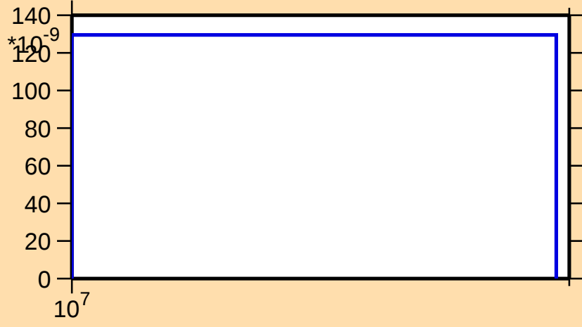
\sigma vs. E for ^{239}\text{Np}(n,nt)
