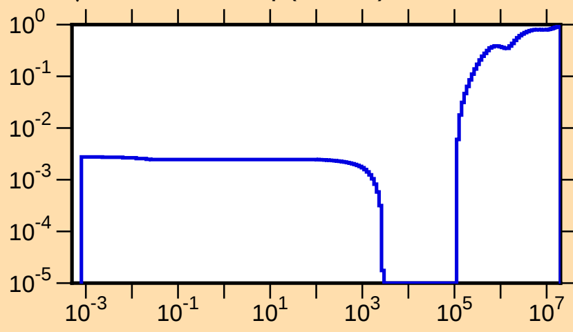
\mu vs. E for ^{242}\text{Np}(\text{mt251})
