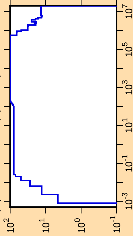
\Delta\mu/\mu vs. E for ^{242}\text{Np}(\text{mt251})
