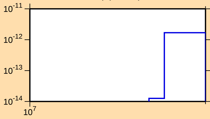
\sigma vs. E for ^{242}\text{Np}(n,3n\alpha)
