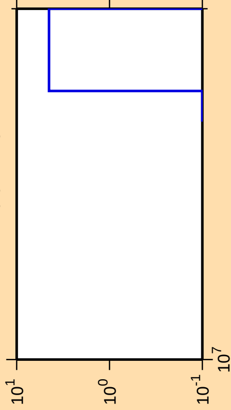
\Delta\sigma/\sigma vs. E for ^{242}\text{Np}(\text{mt 11})
