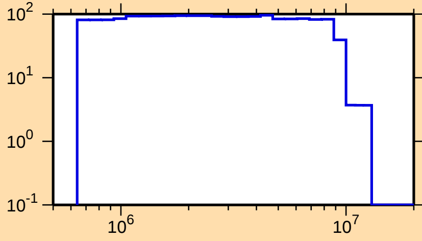
\Delta\sigma/\sigma vs. E for ^{242}\text{Np}(n,n_1)
