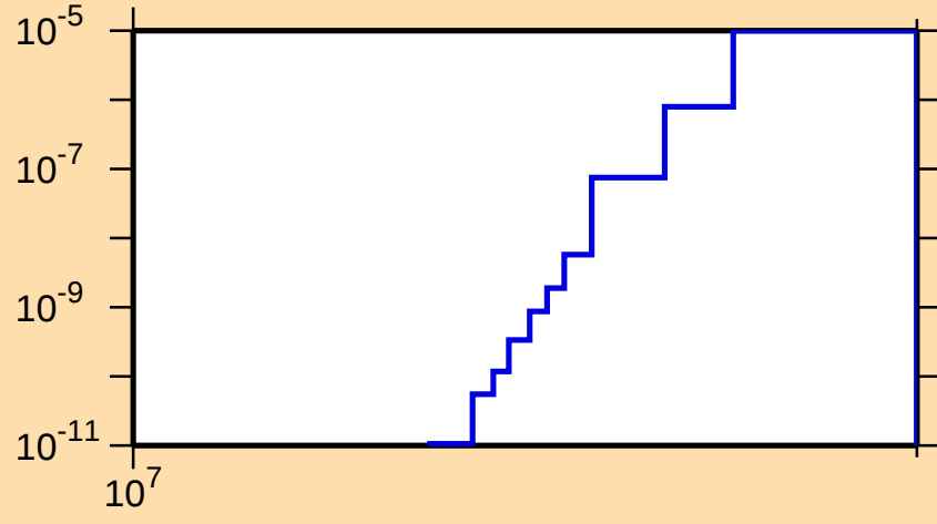
\sigma vs. E for ^{242}\text{Np}(n,nt)
