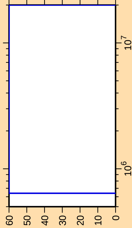
\Delta\sigma/\sigma vs. E for ^{242}\text{Np}(n,n\text{cont.})
