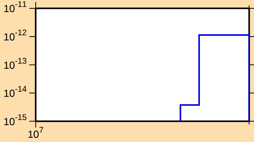
\sigma vs. E for ^{242}\text{Np}(\text{mt 11})
