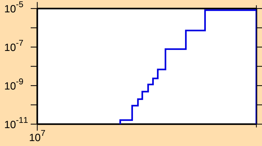
\sigma vs. E for ^{242}\text{Np}(n,\text{nd})
