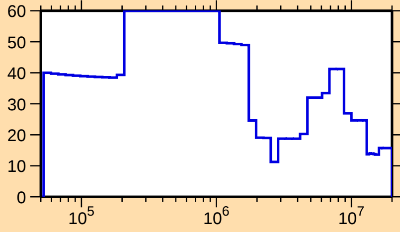
\Delta\sigma/\sigma vs. E for ^{242}\text{Np}(n,\text{el.})
