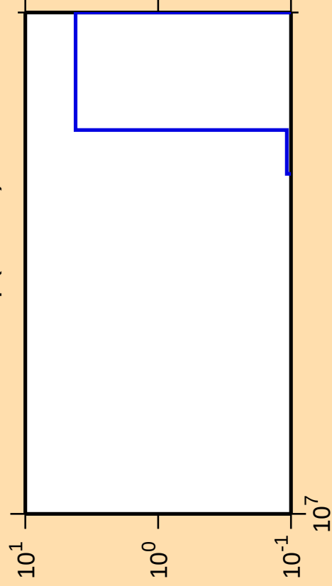
\Delta\sigma/\sigma vs. E for ^{242}\text{Np}(n,\text{He3})
