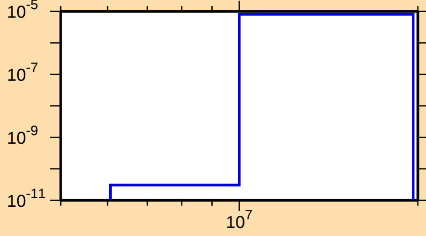
\sigma vs. E for ^{242}\text{Np}(n,n\alpha)
