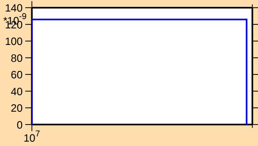
\sigma vs. E for ^{242}\text{Np}(n,\text{nd})
