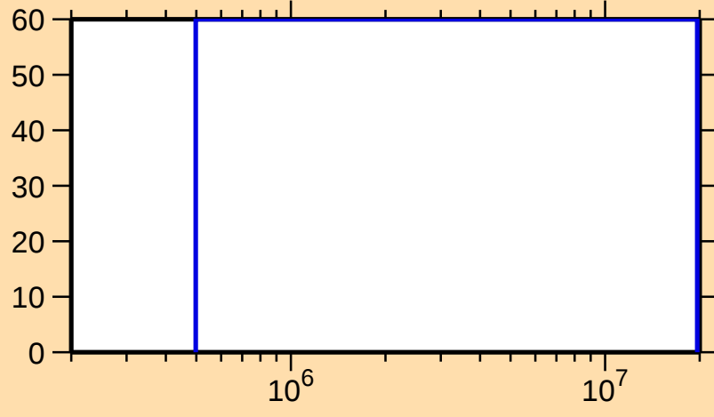
\Delta\sigma/\sigma vs. E for ^{242}\text{Np}(n,n\text{cont.})
