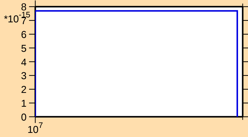
\sigma vs. E for ^{242}\text{Np}(\text{mt 11})
