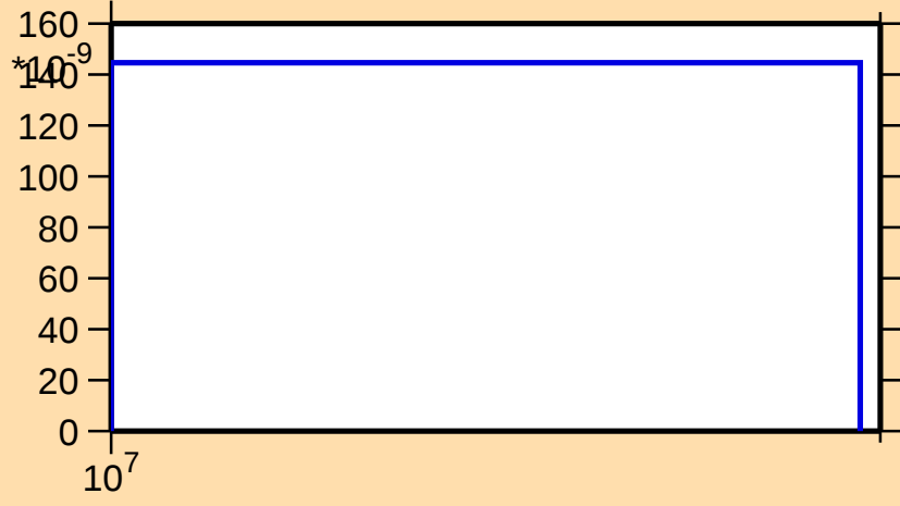
\sigma vs. E for ^{242}\text{Np}(n,nt)
