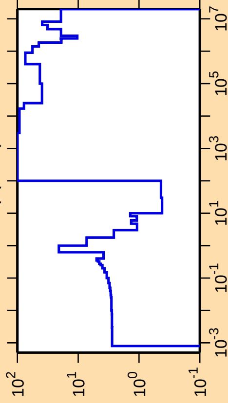
\Delta\sigma/\sigma vs. E for ^{242}\text{Np}(n,\text{el.})
