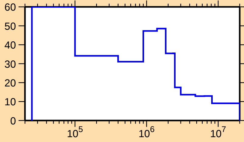
\Delta\sigma/\sigma vs. E for ^{242}\text{Np}(n,\text{nonel.})
