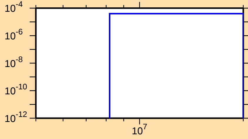
\sigma vs. E for ^{242}\text{Np}(n,t)
