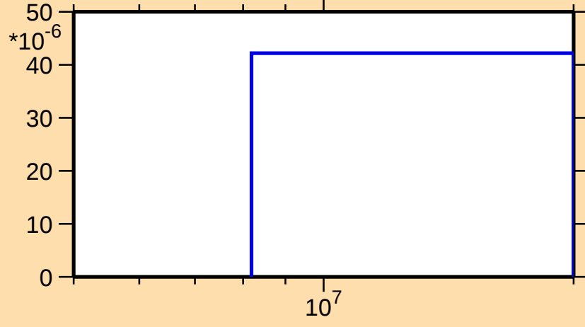
\sigma vs. E for ^{242}\text{Np}(n,np)
