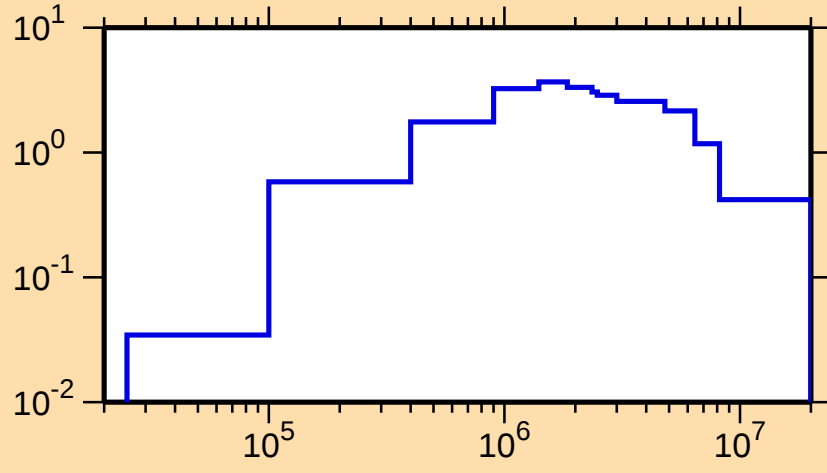
\sigma vs. E for ^{242}\text{Np}(n,\text{inel.})
