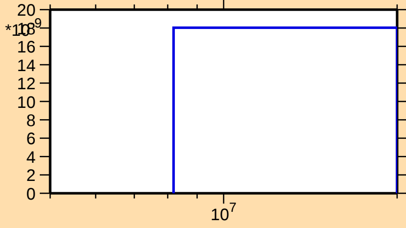
\sigma vs. E for ^{242}\text{Np}(n,2np)
