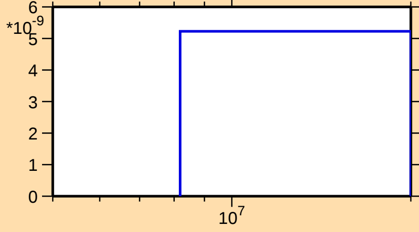
\sigma vs. E for ^{242}\text{Np}(n,2n\alpha)
