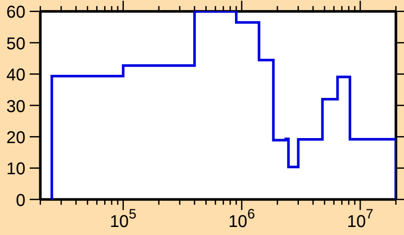
\Delta\sigma/\sigma vs. E for ^{242}\text{Np}(n,\text{el.})
