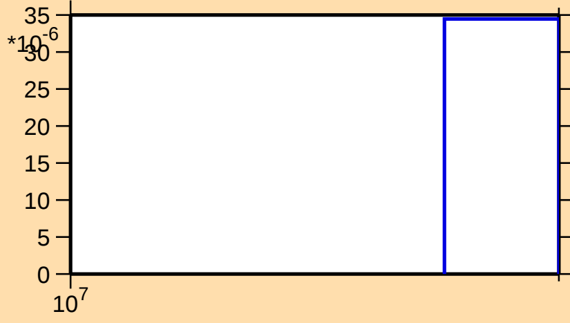
\sigma vs. E for ^{17}\text{O}(\text{n},2\text{np})
