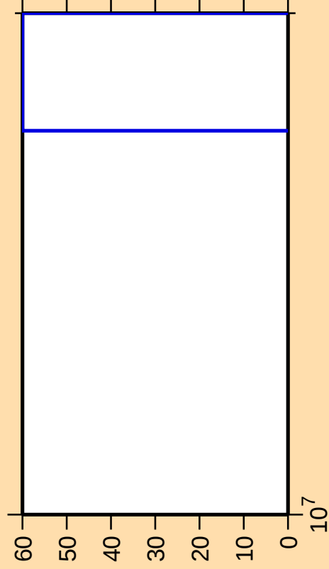
\Delta\sigma/\sigma vs. E for ^{17}\text{O}(\text{n},\text{He3})
