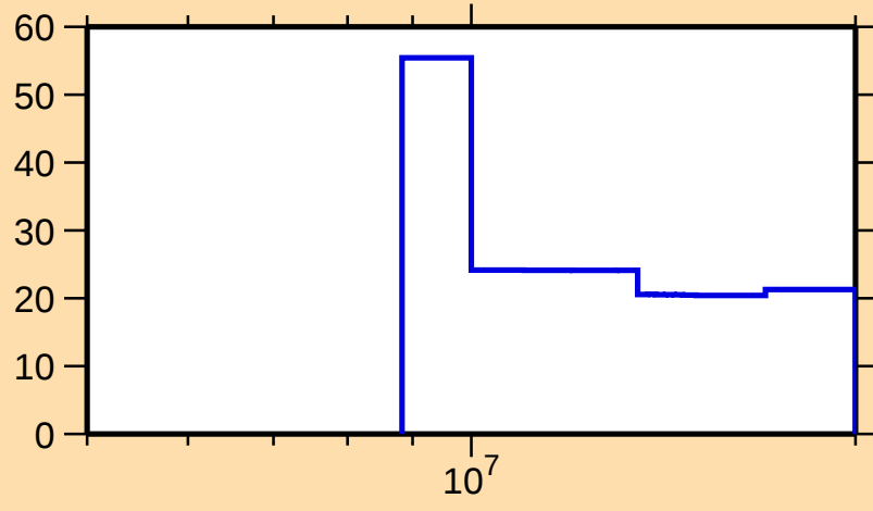
\Delta\sigma/\sigma vs. E for ^{17}\text{O}(\text{n},2\text{n})
