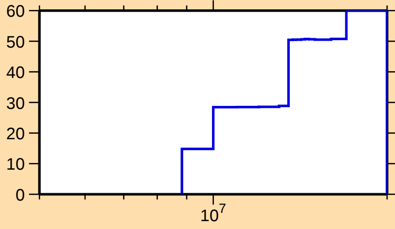
\Delta\sigma/\sigma vs. E for ^{17}\text{O}(\text{n},\text{n}_1)
