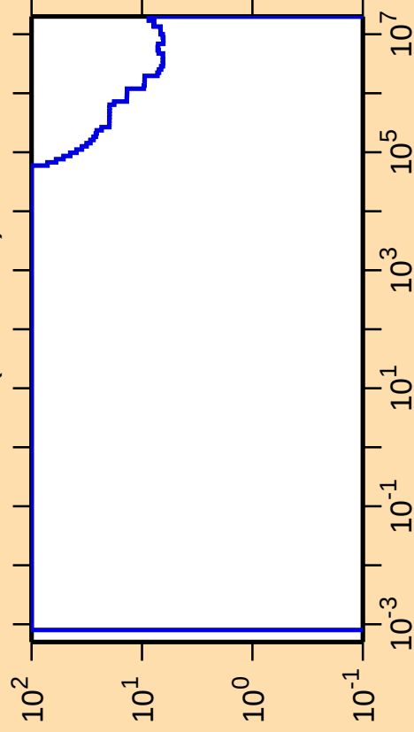
\Delta\sigma/\sigma vs. E for ^{17}\text{O}(\text{n,nonel.})
