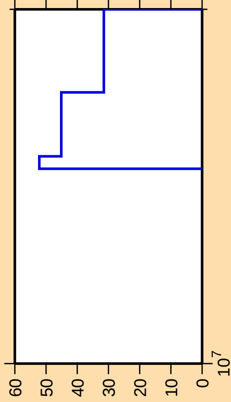
\Delta\sigma/\sigma vs. E for ^{17}\text{O}(\text{n,np})
