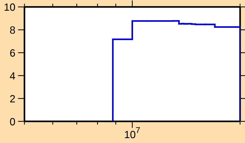
\Delta\sigma/\sigma vs. E for ^{17}\text{O}(\text{n},\text{el.})
