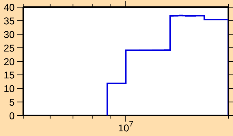
\Delta\sigma/\sigma vs. E for ^{17}\text{O}(\text{n,incl.})
