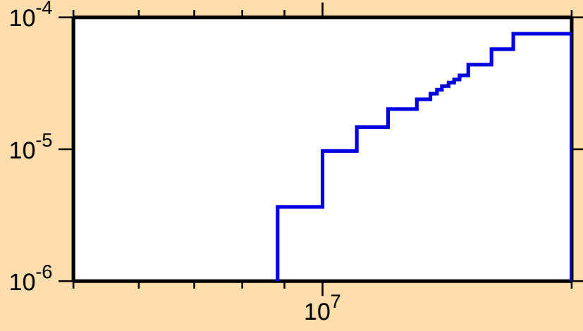
\sigma vs. E for ^{17}\text{O}(\text{n,ncont.})
