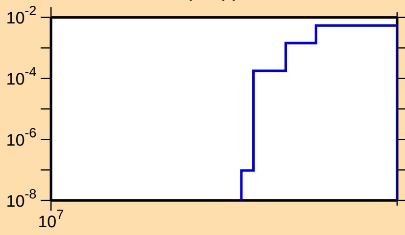
\sigma vs. E for ^{17}\text{O}(\text{n,np})
