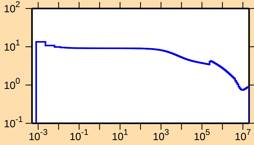
\sigma vs. E for ^{17}\text{O}(\text{n},\text{el.})
