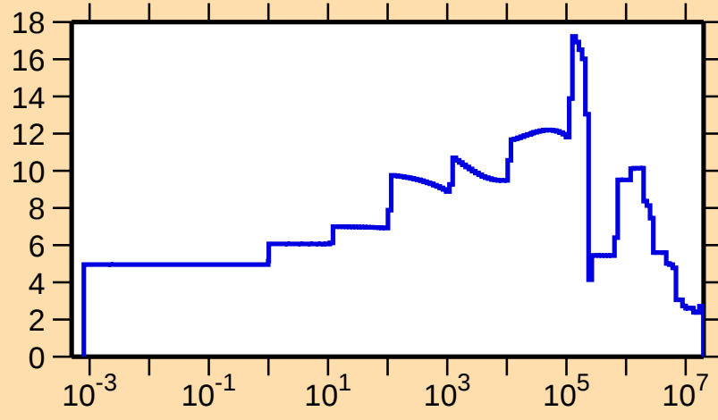
\Delta\sigma/\sigma vs. E for ^{17}\text{O}(\text{n,tot.})
