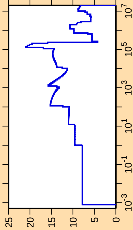
\Delta\sigma/\sigma vs. E for ^{17}\text{O}(\text{n,el.})
