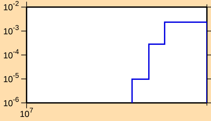
\sigma vs. E for ^{17}\text{O}(\text{n},\text{nd})
