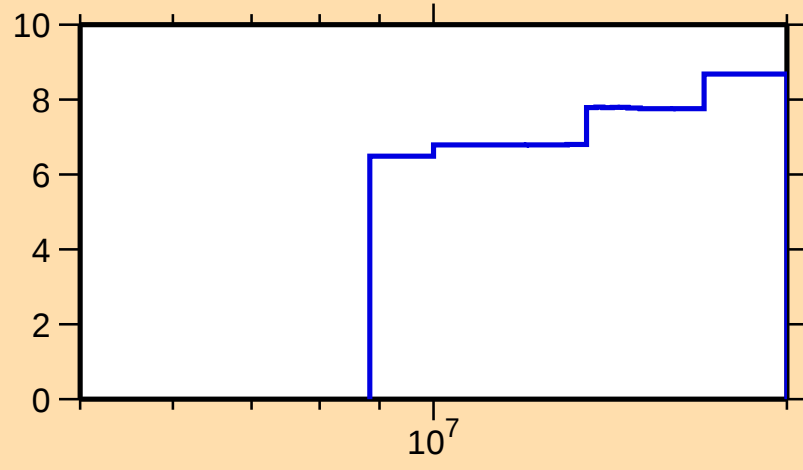
\Delta\sigma/\sigma vs. E for ^{17}\text{O}(\text{n},\text{nonel.})
