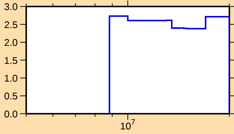
\Delta\sigma/\sigma vs. E for ^{17}\text{O}(\text{n},\text{tot.})
