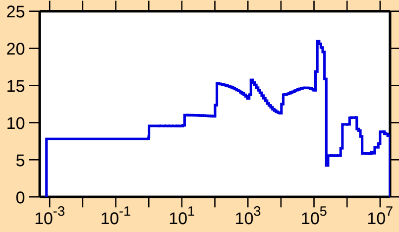
\Delta\sigma/\sigma vs. E for ^{17}\text{O}(\text{n,el.})
