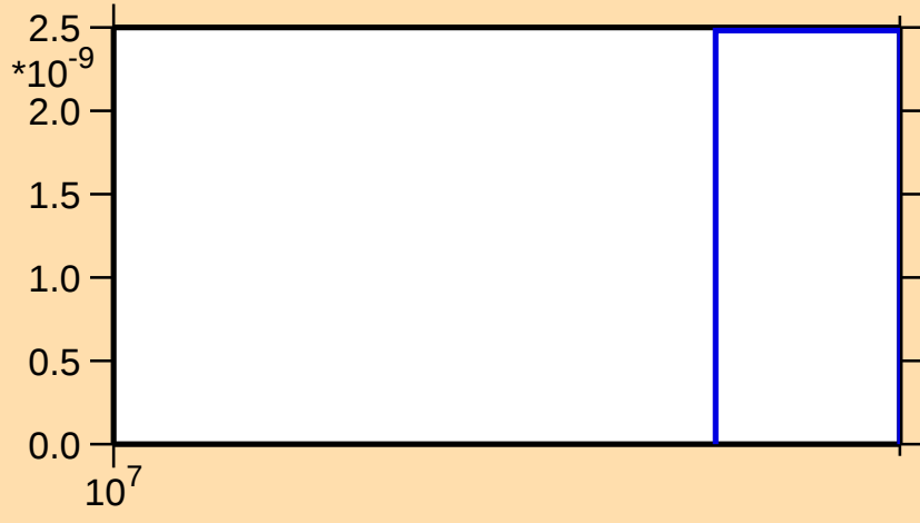
\sigma vs. E for ^{17}\text{O}(\text{n},\text{He3})
