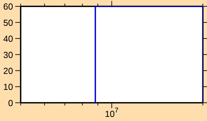
\Delta\sigma/\sigma vs. E for ^{17}\text{O}(\text{n,ncont.})
