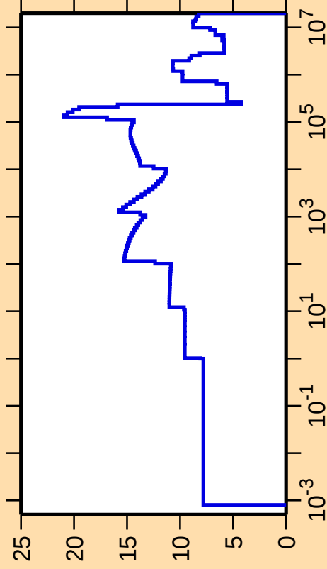
\Delta\sigma/\sigma vs. E for ^{17}\text{O}(\text{n},\text{el.})
