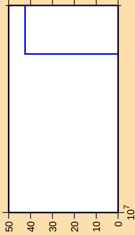
\Delta\sigma/\sigma vs. E for ^{17}\text{O}(\text{n},2\text{np})
