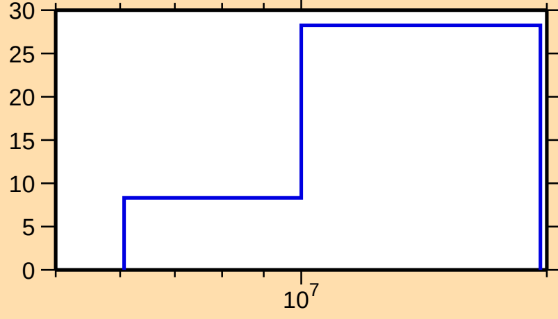
\Delta\sigma/\sigma vs. E for ^{17}\text{O}(\text{n,inel.})
