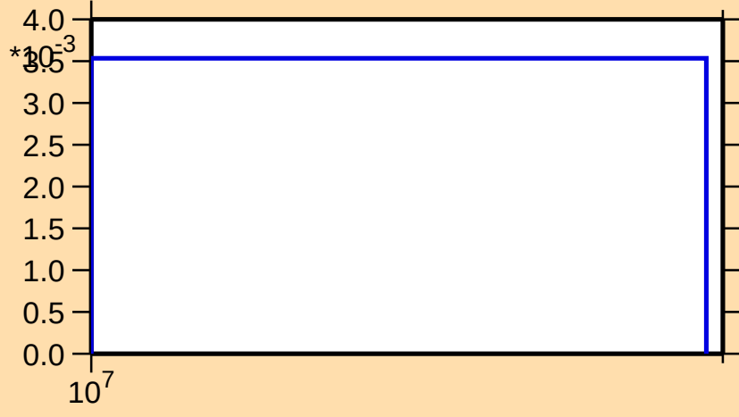
\sigma vs. E for ^{17}\text{O}(\text{n},\text{d})
