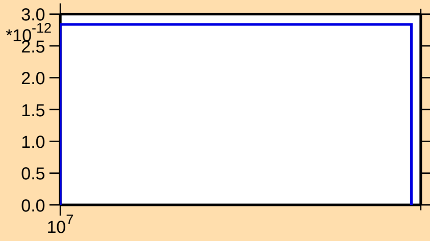
\sigma vs. E for ^{17}\text{O}(\text{n},\text{pt})
