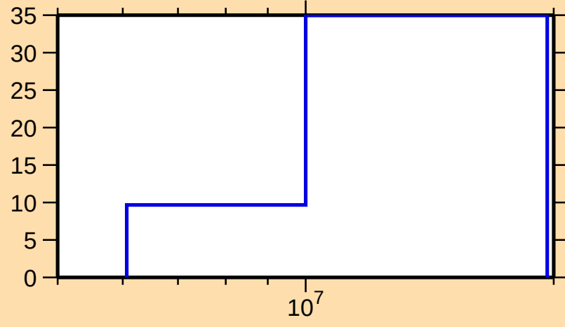
\Delta\sigma/\sigma vs. E for ^{17}\text{O}(\text{n,n}_1)
