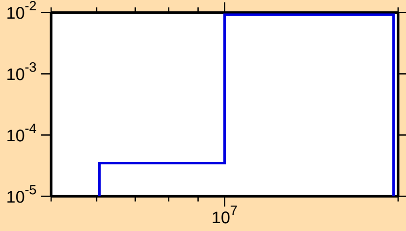
\sigma vs. E for ^{17}\text{O}(n,p)
