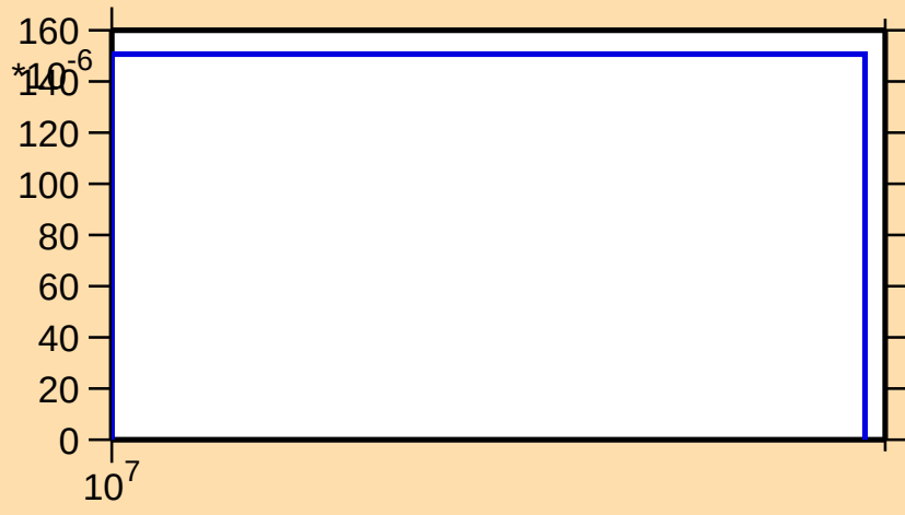
\sigma vs. E for ^{17}\text{O}(\text{n},\text{np})
