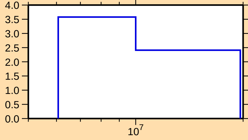
\Delta\sigma/\sigma vs. E for ^{17}\text{O}(\text{n,tot.})
