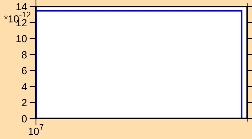
\sigma vs. E for ^{17}\text{O}(\text{n},\text{He3})
