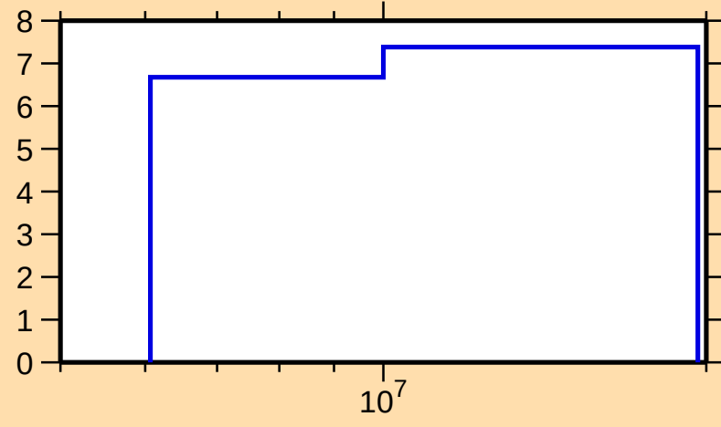
\Delta\sigma/\sigma vs. E for ^{17}\text{O}(\text{n,nonel.})
