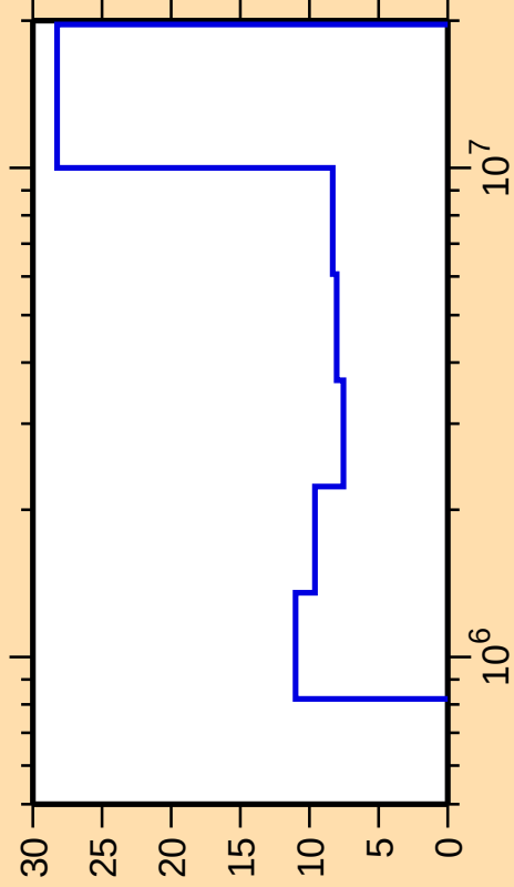
\Delta\sigma/\sigma vs. E for ^{17}\text{O}(\text{n,inel.})
