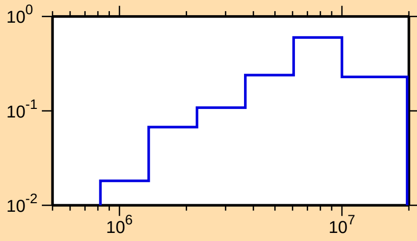
\sigma vs. E for ^{17}\text{O}(\text{n,inel.})
