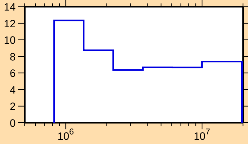
\Delta\sigma/\sigma vs. E for ^{17}\text{O}(\text{n,nonel.})
