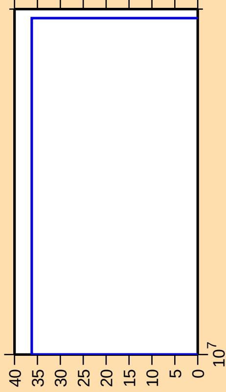
\Delta\sigma/\sigma vs. E for ^{17}\text{O}(\text{n},\text{np})
