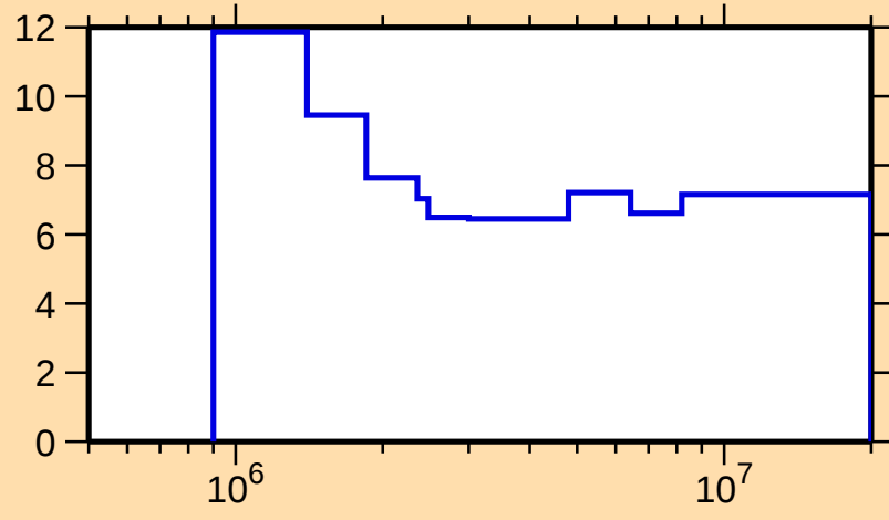
\Delta\sigma/\sigma vs. E for ^{17}\text{O}(\text{n,nonel.})
