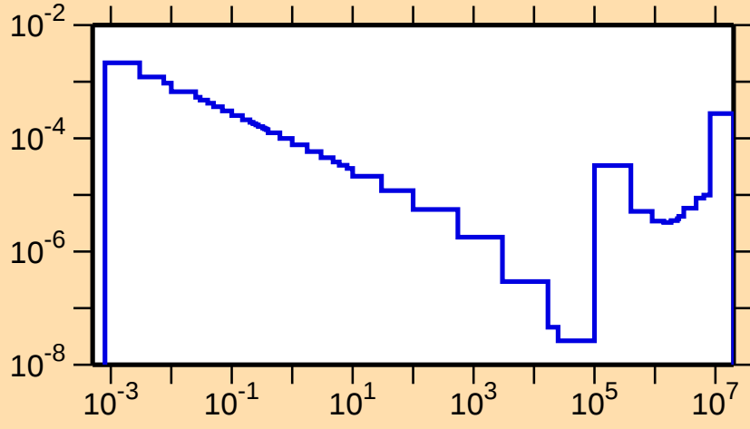
\sigma vs. E for ^{17}\text{O}(n,\gamma)
