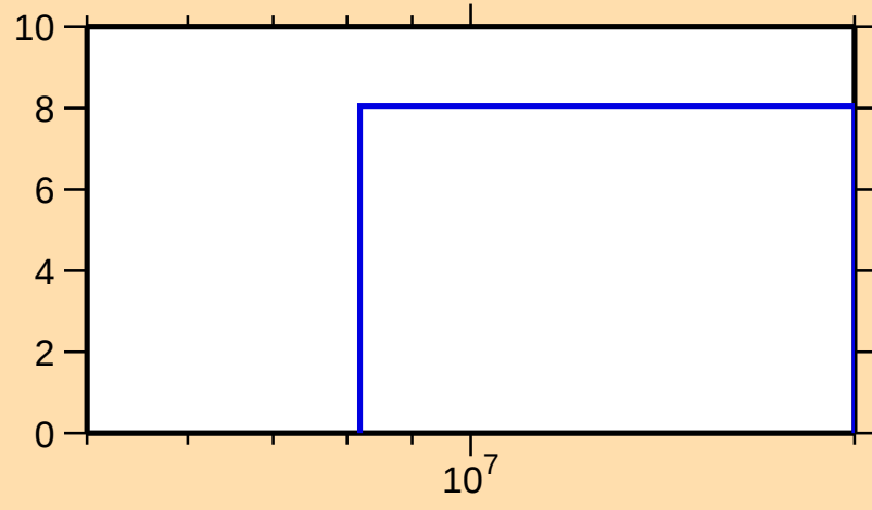
\Delta\sigma/\sigma vs. E for ^{17}\text{O}(\text{n,el.})
