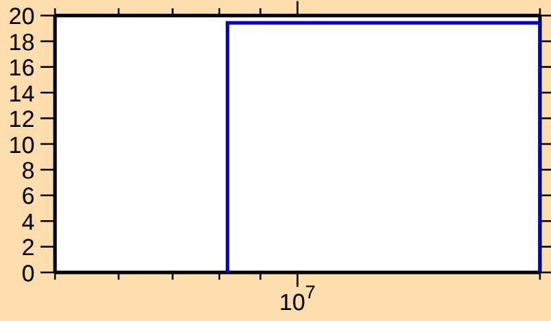
\Delta\sigma/\sigma vs. E for ^{17}\text{O}(\text{n,inel.})
