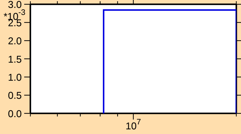
\sigma vs. E for ^{17}\text{O}(\text{n,d})
