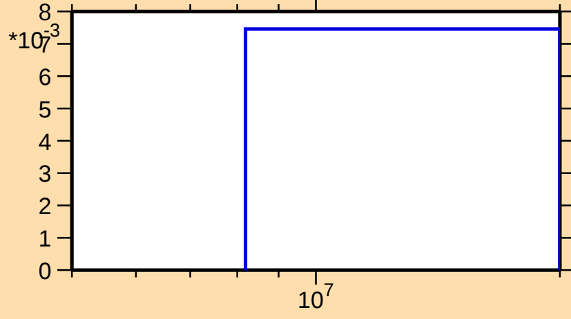
\sigma vs. E for ^{17}\text{O}(\text{n,p})
