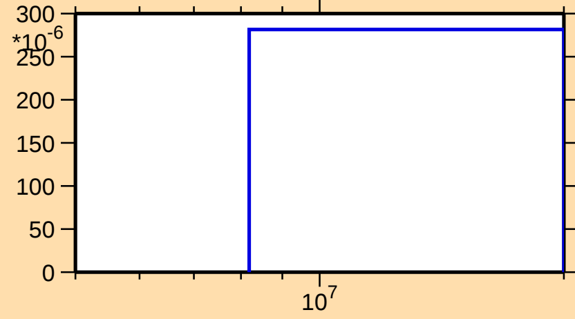
\sigma vs. E for ^{17}\text{O}(n,2n\alpha)
