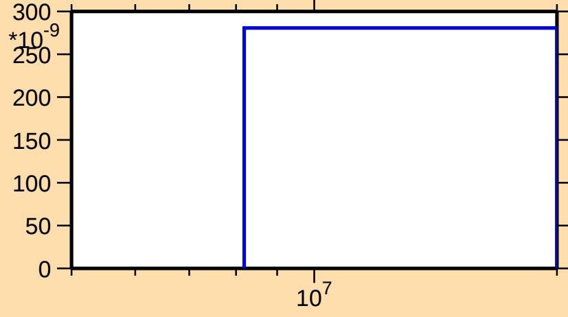
\sigma vs. E for ^{17}\text{O}(n,2np)
