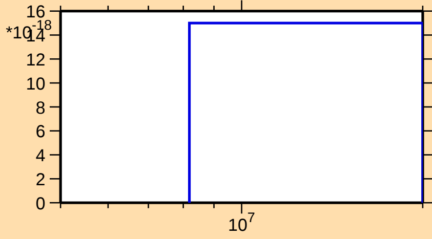
\sigma vs. E for ^{17}\text{O}(\text{n},\text{nt})
