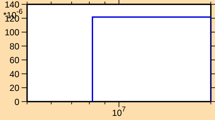
\sigma vs. E for ^{17}\text{O}(\text{n},\text{np})
