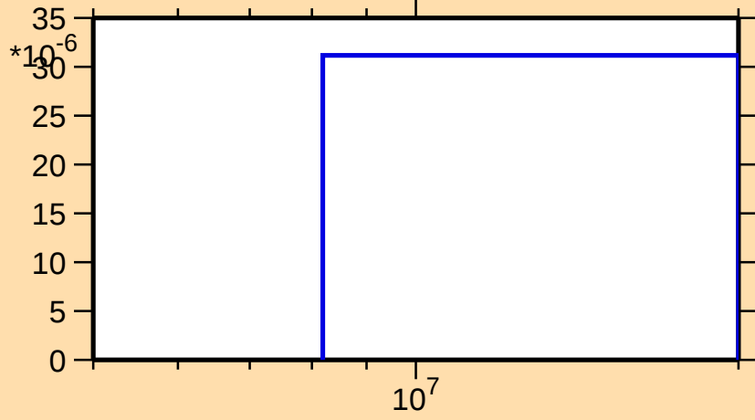
\sigma vs. E for ^{17}\text{O}(\text{n},\text{nd})
