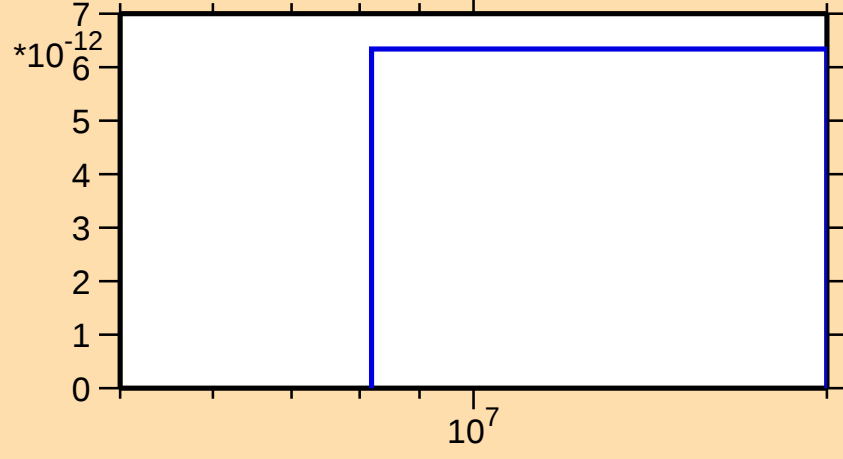
\sigma vs. E for ^{17}\text{O}(\text{n},\text{pt})
