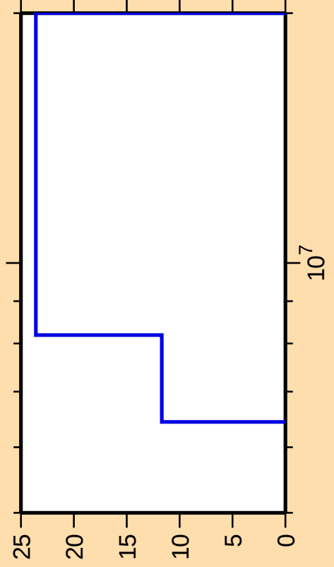
\Delta\sigma/\sigma vs. E for ^{17}\text{O}(n,\alpha)
