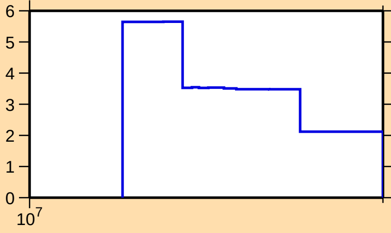
\Delta\sigma/\sigma vs. E for ^{19}\text{O}(\text{n,tot.})
