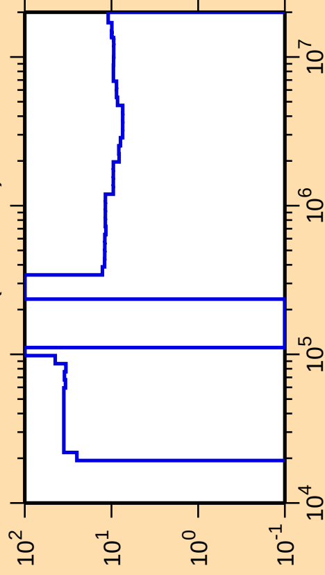
\Delta\sigma/\sigma vs. E for ^{19}\text{O}(\text{n,nonel.})
