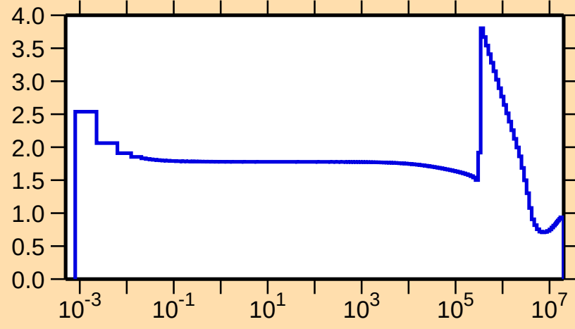
\sigma vs. E for ^{19}\text{O}(\text{n,el.})
