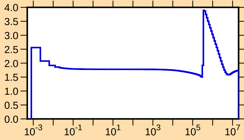
\sigma vs. E for ^{19}\text{O}(\text{n,tot.})
