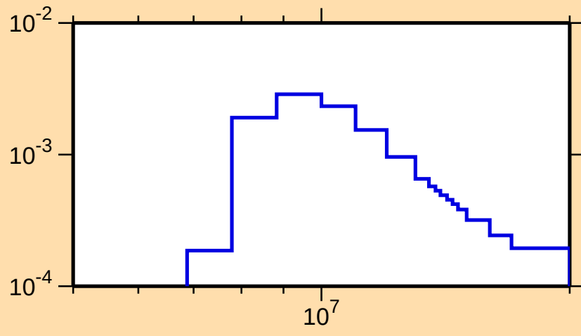
\sigma vs. E for ^{19}\text{O}(\text{n,ncont.})
