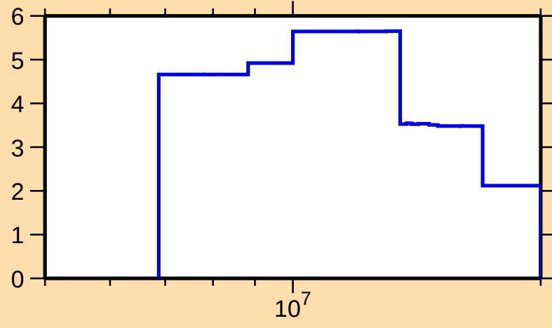
\Delta\sigma/\sigma vs. E for ^{19}\text{O}(\text{n},\text{tot.})
