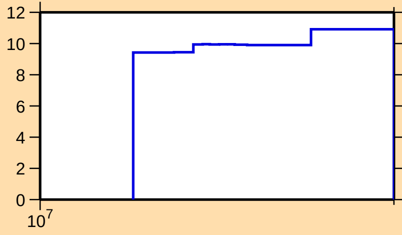
\Delta\sigma/\sigma vs. E for ^{19}\text{O}(\text{n,nonel.})
