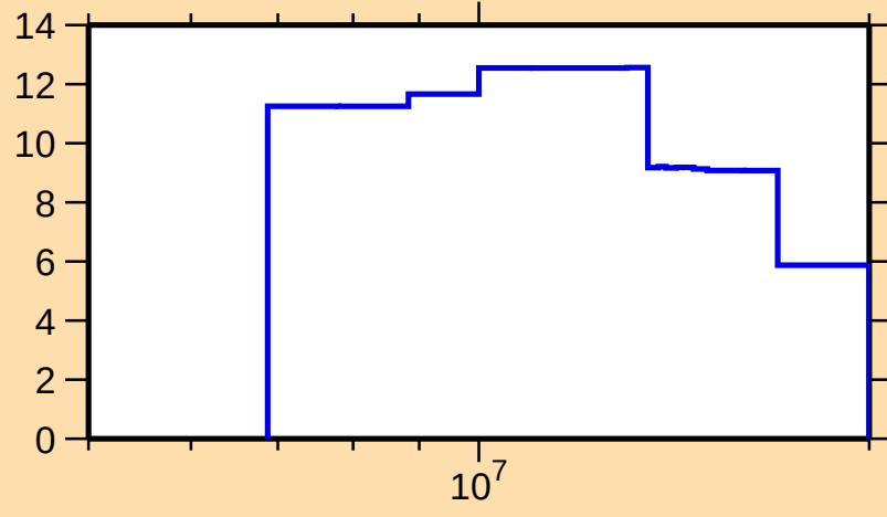
\Delta\sigma/\sigma vs. E for ^{19}\text{O}(\text{n},\text{el.})
