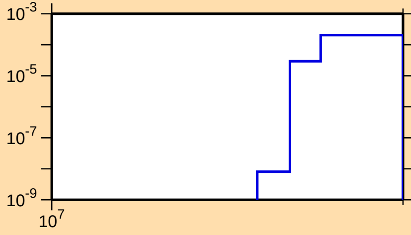
\sigma vs. E for ^{19}\text{O}(\text{n,d})
