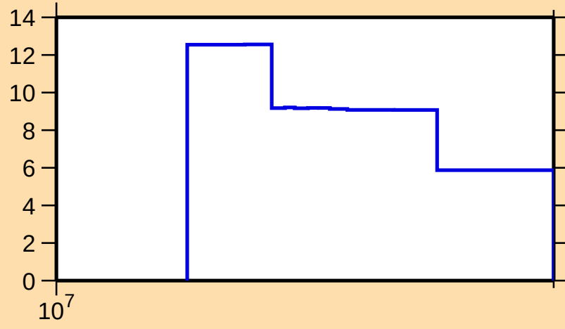
\Delta\sigma/\sigma vs. E for ^{19}\text{O}(\text{n,el.})
