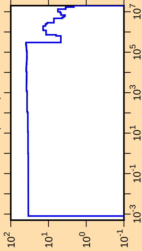
\Delta\sigma/\sigma vs. E for ^{19}\text{O}(\text{n,tot.})
