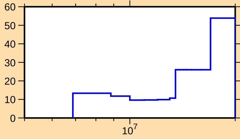
\Delta\sigma/\sigma vs. E for ^{19}\text{O}(\text{n,inel.})
