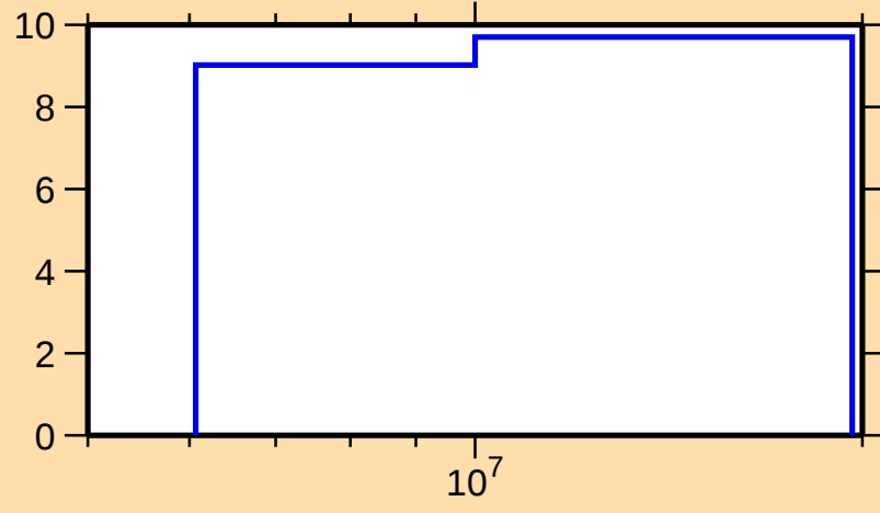
\Delta\sigma/\sigma vs. E for ^{19}\text{O}(\text{n},\text{nonel.})
