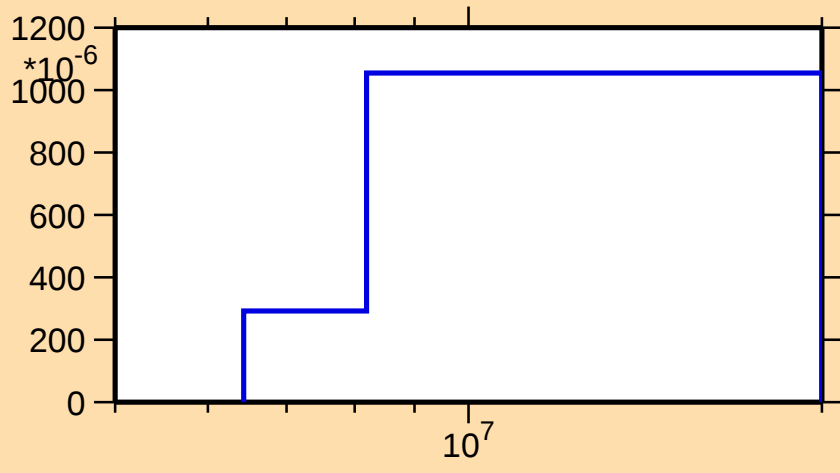
\sigma vs. E for ^{19}\text{O}(\text{n},\text{ncont.})
