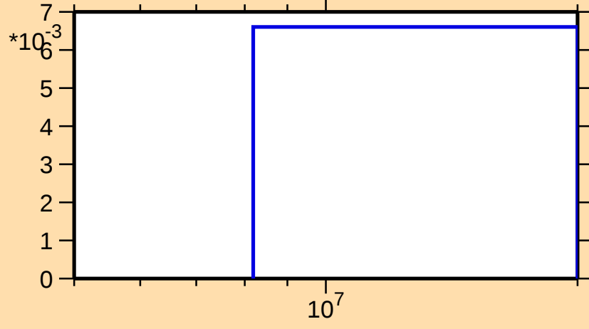
\sigma vs. E for ^{19}\text{O}(n,3n)
