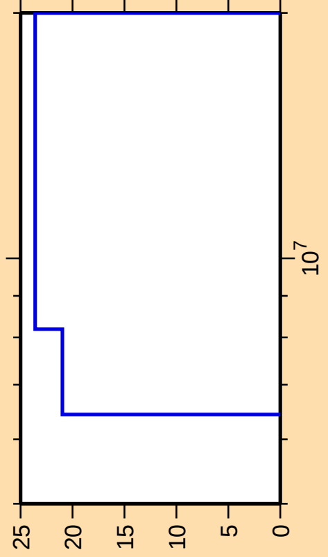
\Delta\sigma/\sigma vs. E for ^{19}\text{O}(n,\alpha)
