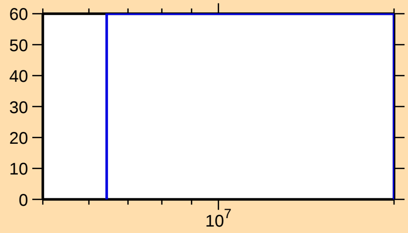
\Delta\sigma/\sigma vs. E for ^{19}\text{O}(n,\text{ncont.})
