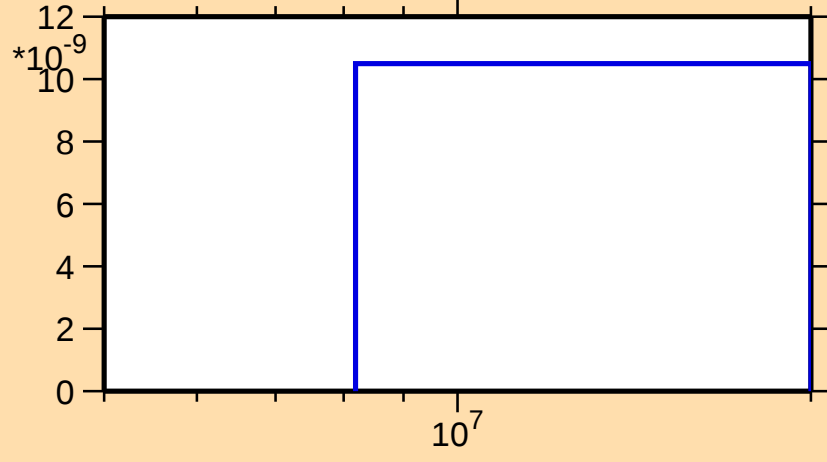
\sigma vs. E for ^{19}\text{O}(n,np)
