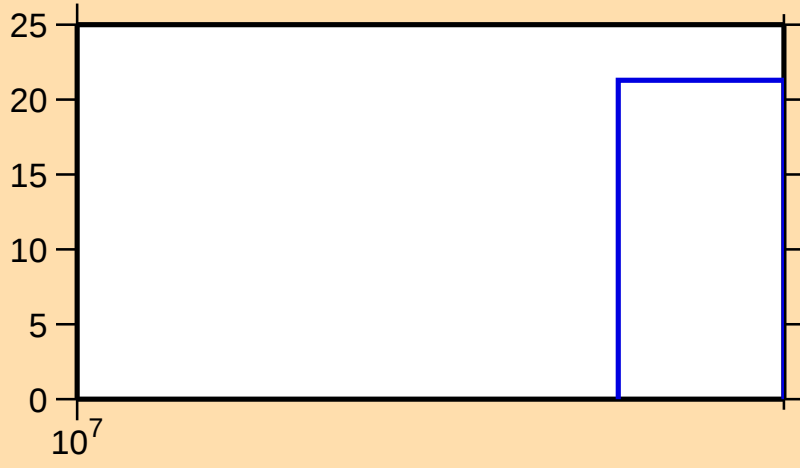
\Delta\sigma/\sigma vs. E for ^{21}\text{O}(\text{n},2\text{n})
