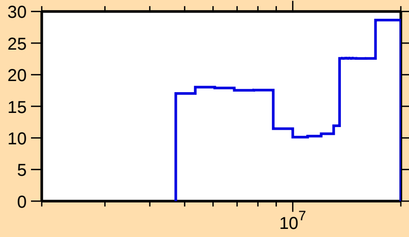
\Delta\sigma/\sigma vs. E for ^{21}\text{O}(\text{n,incl.})
