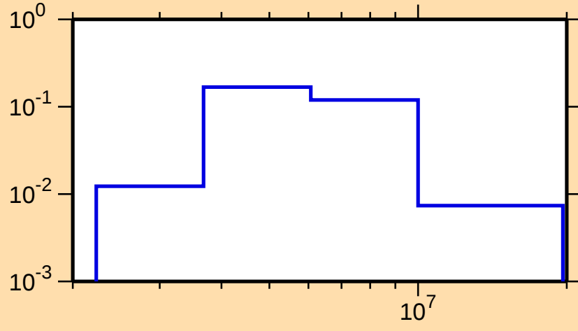
\sigma vs. E for ^{21}\text{O}(n,n_4)
