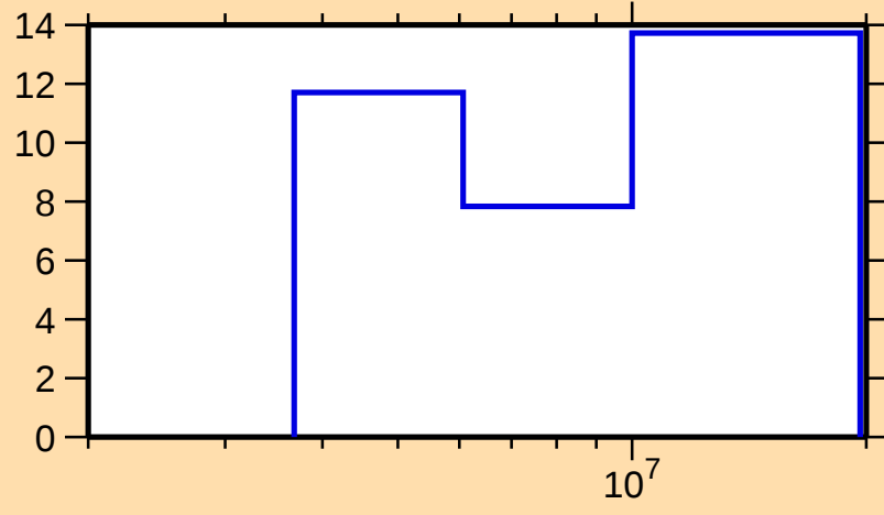
\Delta\sigma/\sigma vs. E for ^{21}\text{O}(\text{n},\text{el.})
