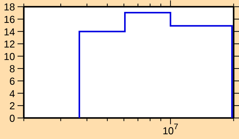
\Delta\sigma/\sigma vs. E for ^{21}\text{O}(\text{n,inel.})
