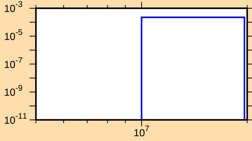
\sigma vs. E for ^{169}\text{Os}(n,2n\alpha)
