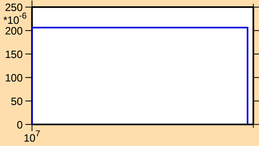
\sigma vs. E for ^{169}\text{Os}(n,2np)
