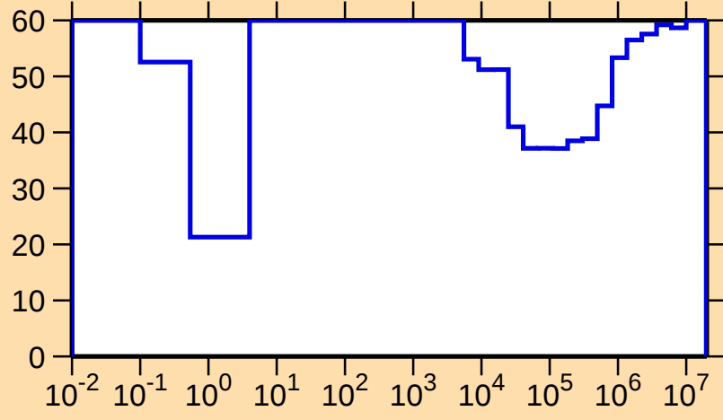
\Delta\sigma/\sigma vs. E for ^{169}\text{Os}(n,\gamma)
