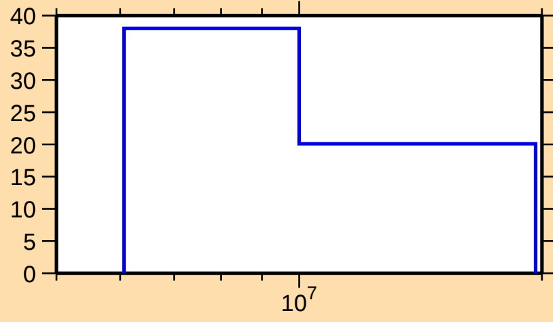
\Delta\sigma/\sigma vs. E for ^{169}\text{Os}(n,\text{inel.})
