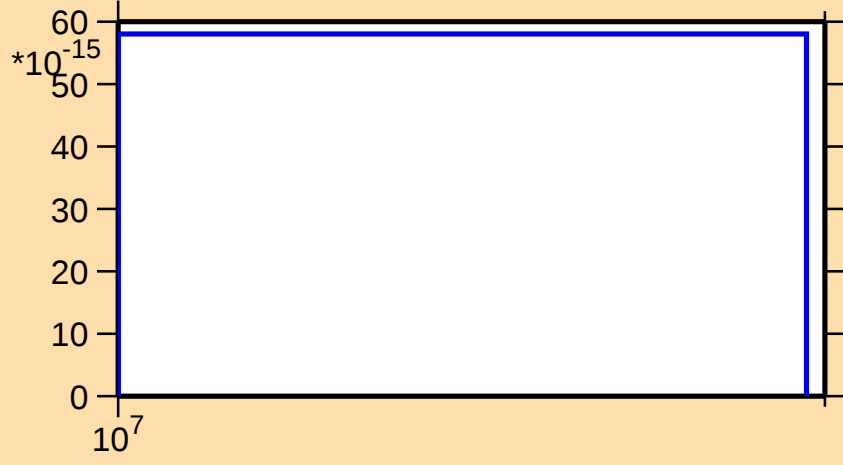
\sigma vs. E for ^{169}\text{Os}(n,nt)
