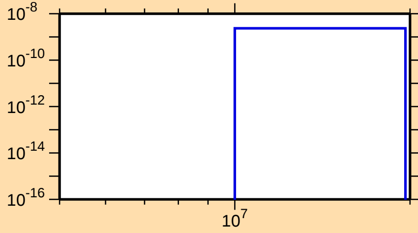
\sigma vs. E for ^{169}\text{Os} (mt 34)
