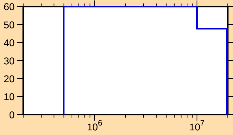
\Delta\sigma/\sigma vs. E for ^{169}\text{Os}(n,n\text{cont.})
