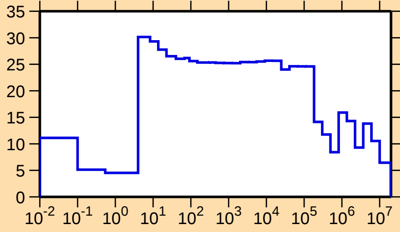
\Delta\sigma/\sigma vs. E for ^{169}\text{Os}(n,\text{el.})
