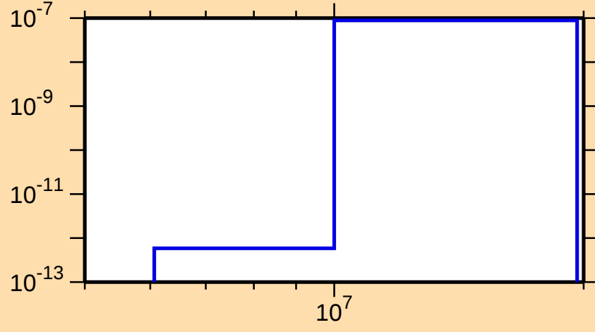
\sigma vs. E for ^{169}\text{Os}(\text{mt117})
