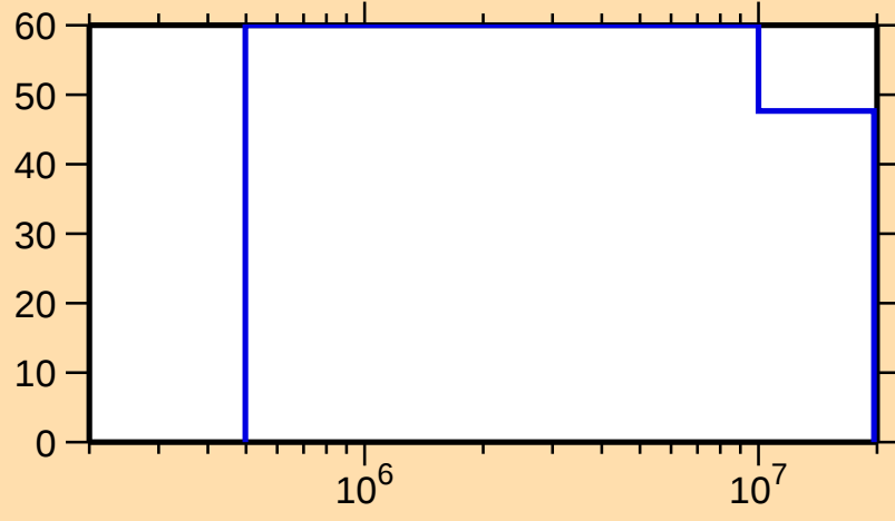
\Delta\sigma/\sigma vs. E for ^{169}\text{Os}(n,n\text{cont.})
