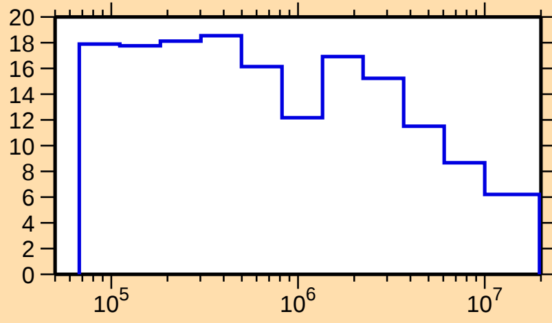
\Delta\sigma/\sigma vs. E for ^{169}\text{Os}(n,\text{nonel.})
