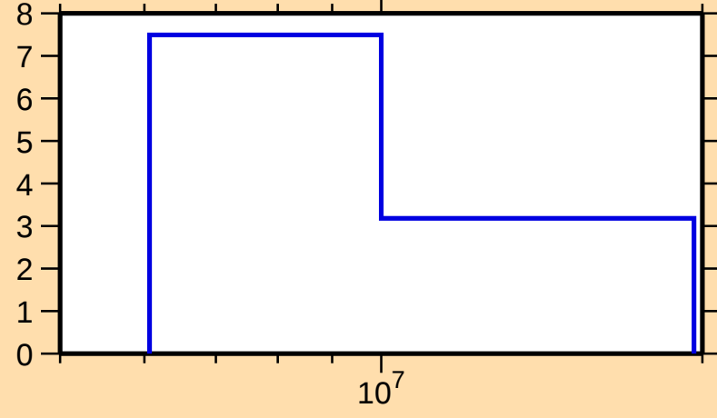
\Delta\sigma/\sigma vs. E for ^{169}\text{Os}(n,\text{tot.})
