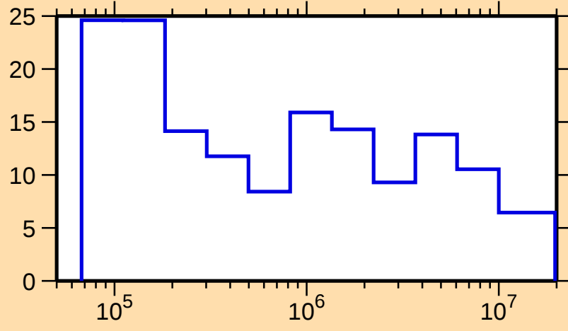
\Delta\sigma/\sigma vs. E for ^{169}\text{Os}(n,\text{el.})
