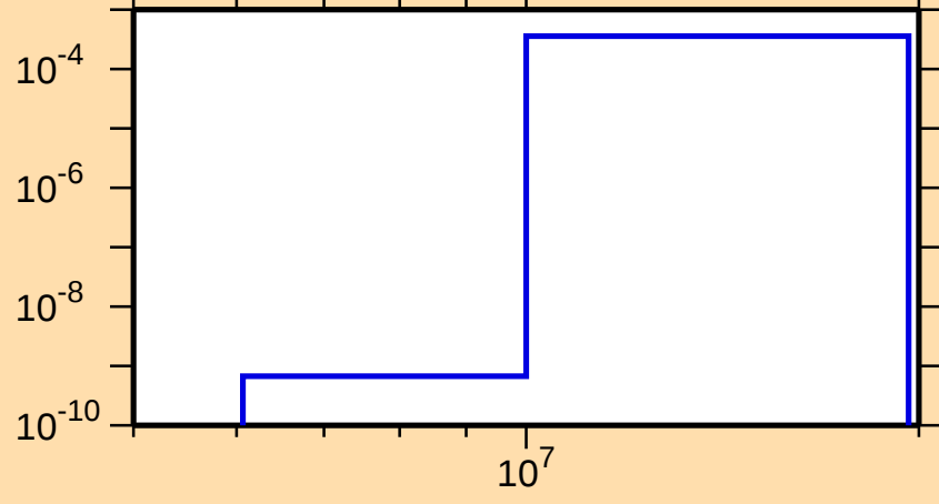
\sigma vs. E for ^{169}\text{Os}(n,t)
