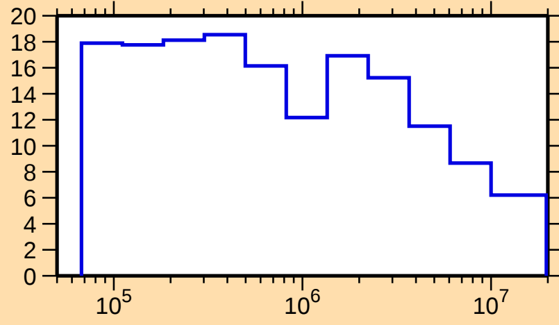
\Delta\sigma/\sigma vs. E for ^{169}\text{Os}(n,\text{nonel.})
