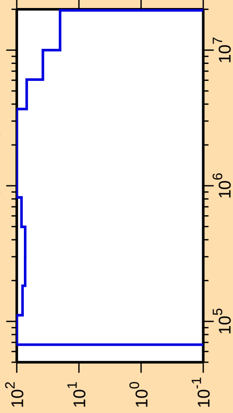
\Delta\sigma/\sigma vs. E for ^{169}\text{Os}(n,\text{inel.})
