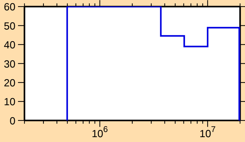
\Delta\sigma/\sigma vs. E for ^{169}\text{Os}(n, n_1)
