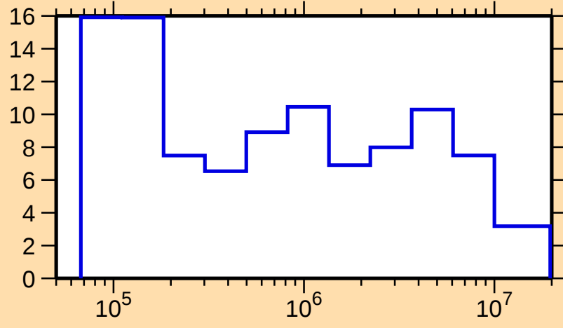
\Delta\sigma/\sigma vs. E for ^{169}\text{Os}(n,\text{tot.})
