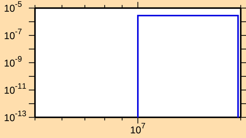
\sigma vs. E for ^{169}\text{Os}(n,\text{pt})
