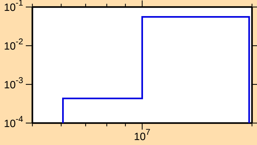
\sigma vs. E for ^{169}\text{Os}(n,2n)
