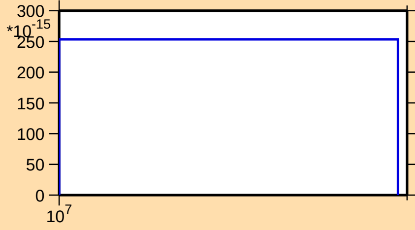
\sigma vs. E for ^{171}\text{Os}(n,nt)
