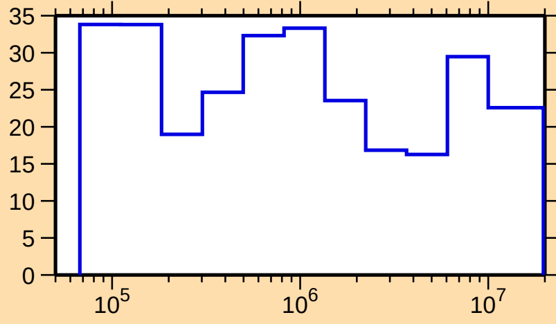
\Delta\sigma/\sigma vs. E for ^{171}\text{Os}(n,\text{el.})
