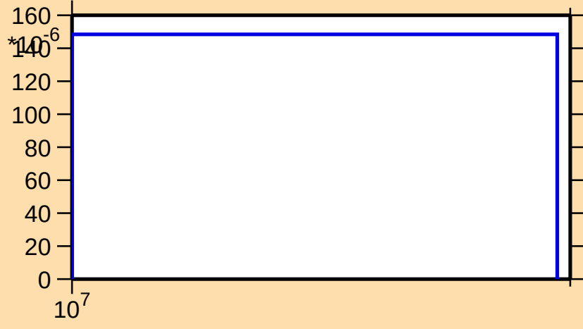
\sigma vs. E for ^{171}\text{Os}(n,2np)
