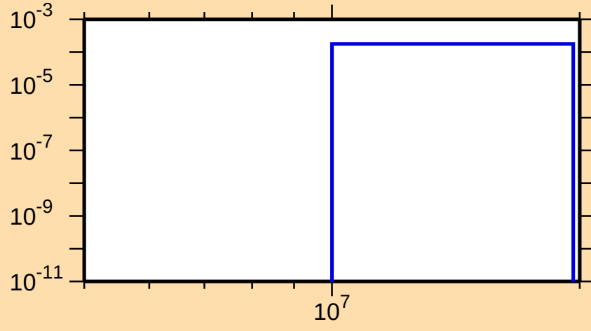
\sigma vs. E for ^{171}\text{Os}(n,2n\alpha)
