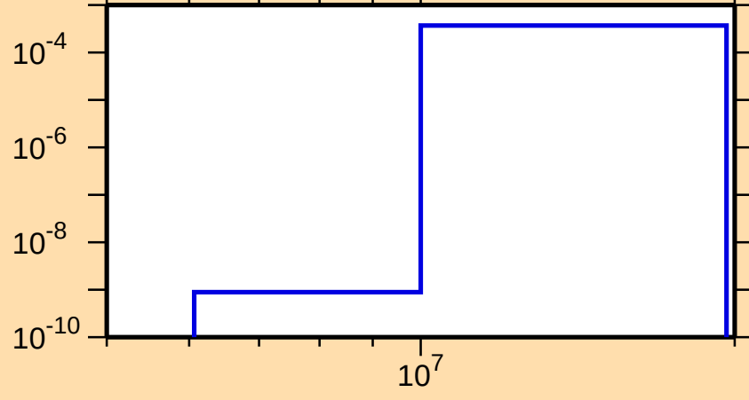
\sigma vs. E for ^{171}\text{Os}(n,t)
