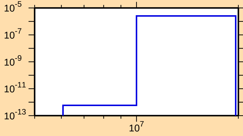
\sigma vs. E for ^{171}\text{Os}(n,\text{pd})
