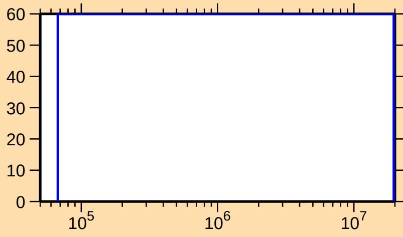
\Delta\sigma/\sigma vs. E for ^{171}\text{Os}(n,n_1)
