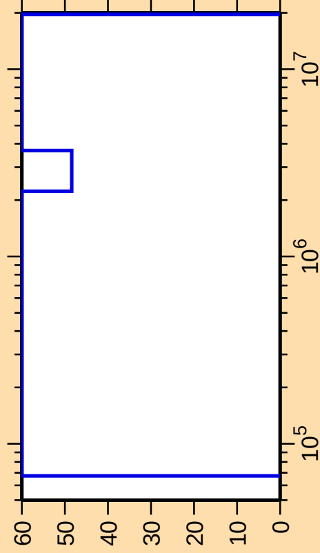
\Delta\sigma/\sigma vs. E for ^{171}\text{Os}(n,\text{inel.})
