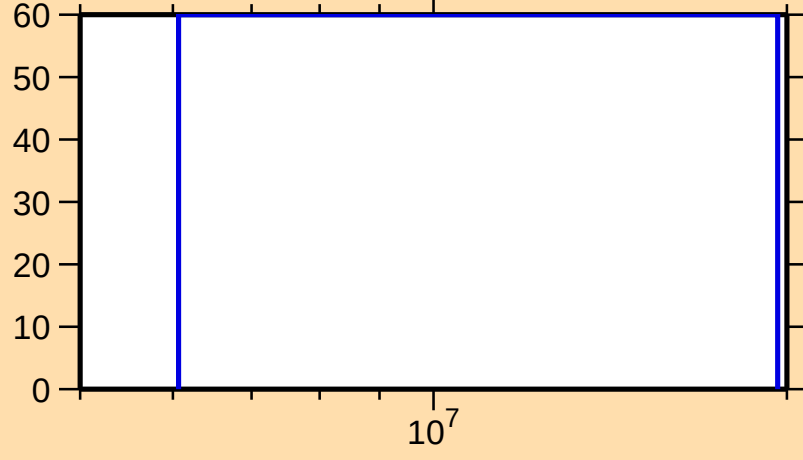
\Delta\sigma/\sigma vs. E for ^{171}\text{Os}(n,\text{inel.})
