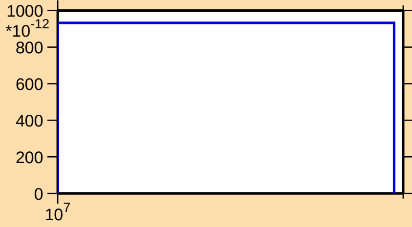
\sigma vs. E for ^{171}\text{Os} (mt 34)
