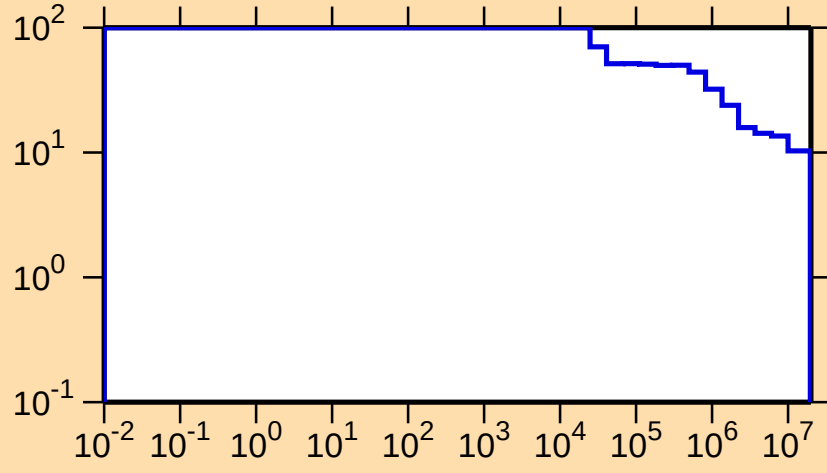
\Delta\sigma/\sigma vs. E for ^{171}\text{Os}(n,\text{nonel.})
