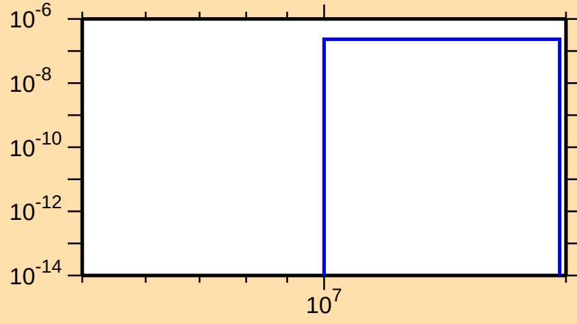
\sigma vs. E for ^{171}\text{Os}(n,\text{nd})
