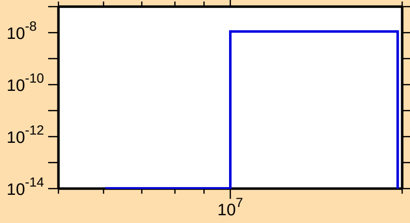
\sigma vs. E for ^{171}\text{Os}(\text{mt117})
