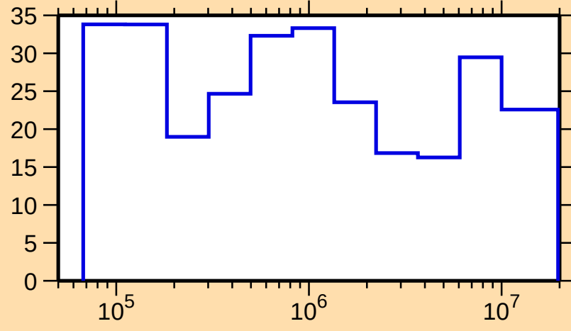
\Delta\sigma/\sigma vs. E for ^{171}\text{Os}(n,\text{el.})
