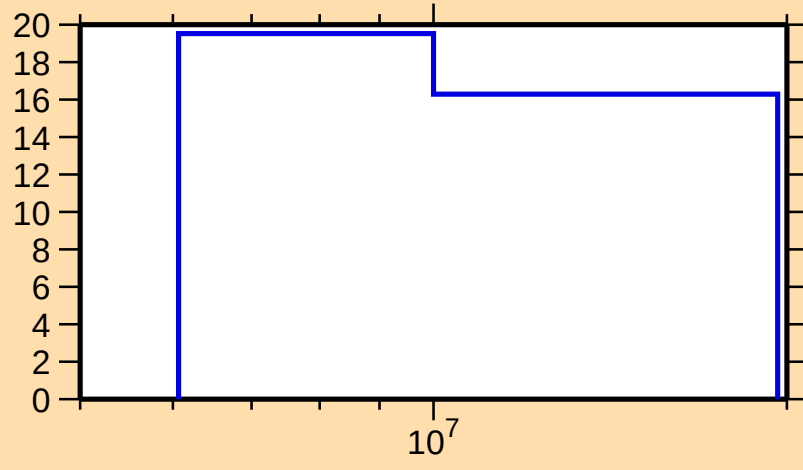
\Delta\sigma/\sigma vs. E for ^{171}\text{Os}(n,\text{tot.})
