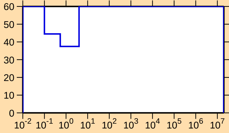
\Delta\sigma/\sigma vs. E for ^{171}\text{Os}(n,\gamma)
