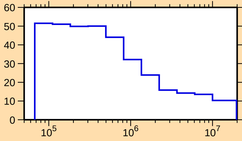
\Delta\sigma/\sigma vs. E for ^{171}\text{Os}(n,\text{nonel.})
