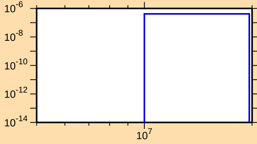
\sigma vs. E for ^{171}\text{Os}(n,\text{pt})
