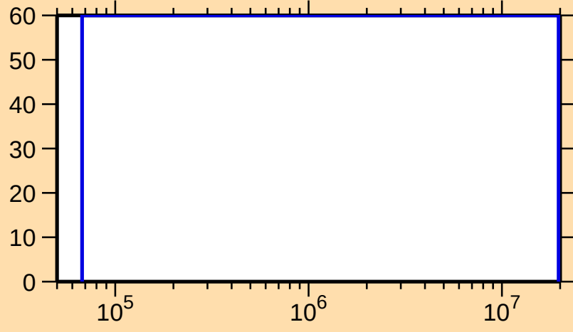
\Delta\sigma/\sigma vs. E for ^{171}\text{Os}(n,n_1)
