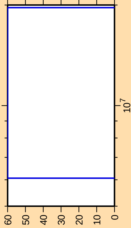
\Delta\sigma/\sigma vs. E for ^{171}\text{Os}(n,t)
