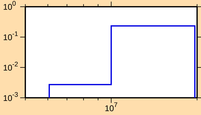
\sigma vs. E for ^{171}\text{Os}(n,2n)
