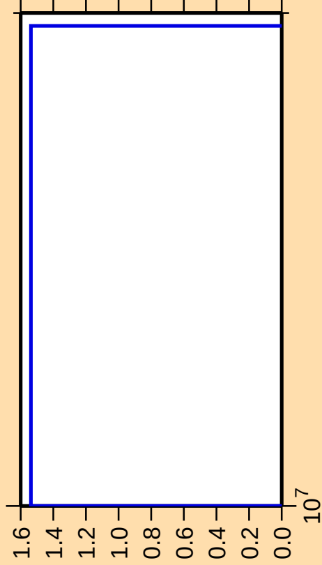
\Delta\sigma/\sigma vs. E for ^{171}\text{Os}(n,nt)
