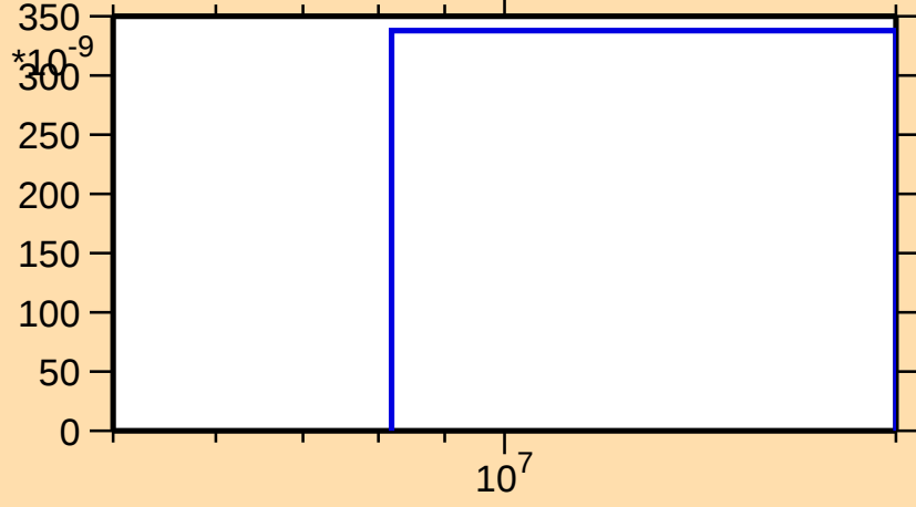
\sigma vs. E for ^{171}\text{Os}(n,\text{pt})
