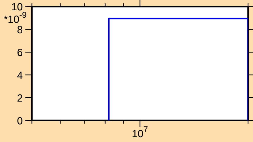
\sigma vs. E for ^{171}\text{Os}(\text{mt117})
