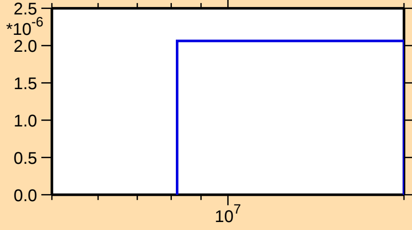
\sigma vs. E for ^{171}\text{Os}(n,\text{pd})
