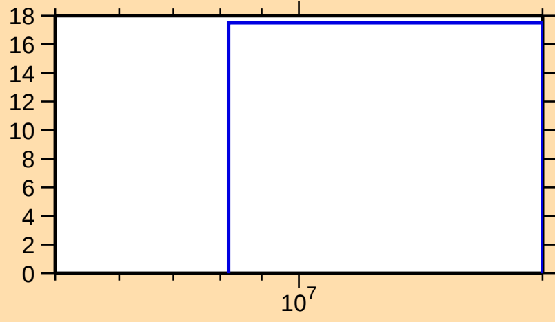
\Delta\sigma/\sigma vs. E for ^{171}\text{Os}(n,\text{tot.})
