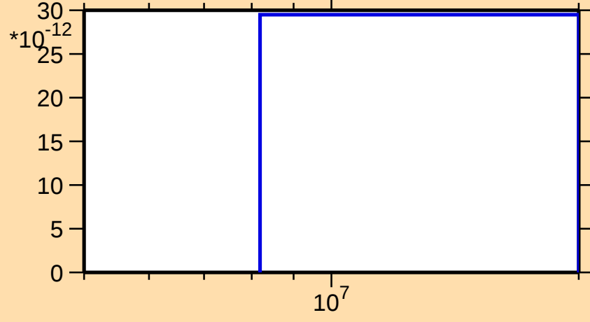
\sigma vs. E for ^{171}\text{Os}(n,3n)
