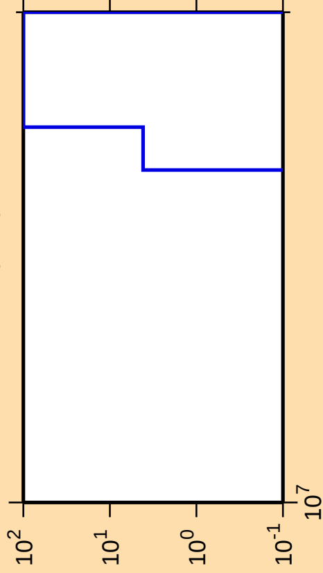
\Delta\sigma/\sigma vs. E for ^{181}\text{Os}(n,\text{nt})
