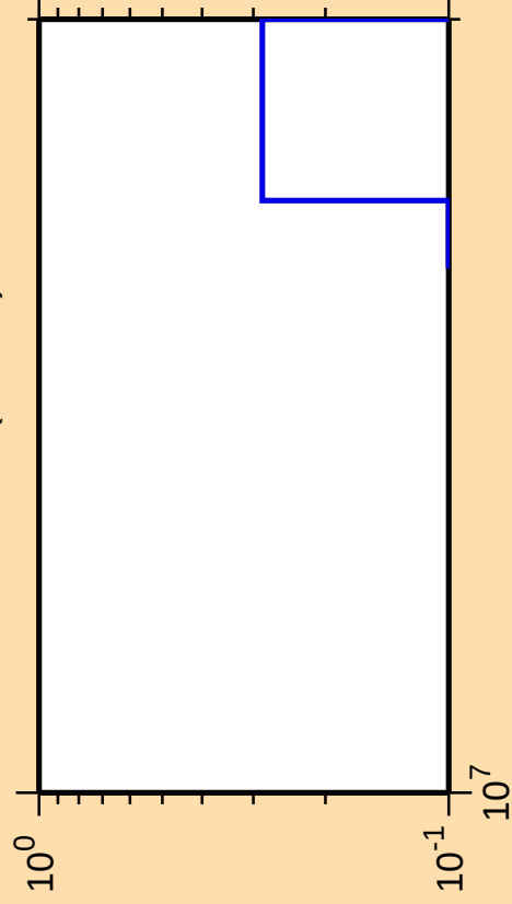
\Delta\sigma/\sigma vs. E for ^{181}\text{Os}(n,3n\alpha)
