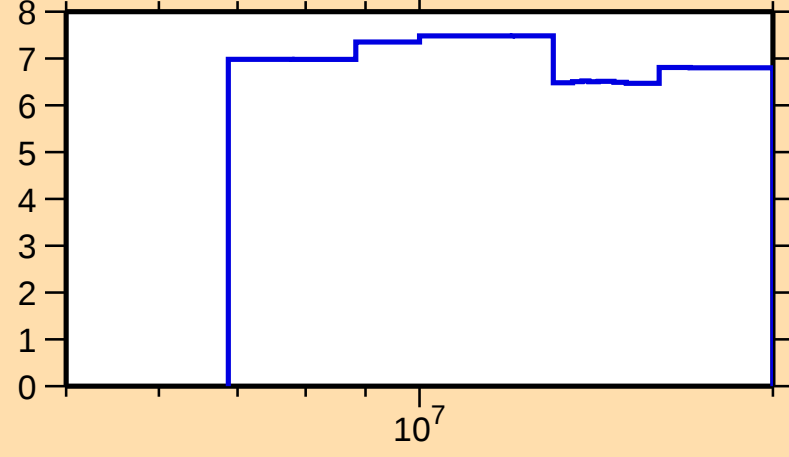
\Delta\sigma/\sigma vs. E for ^{181}\text{Os}(n,\text{nonel.})
