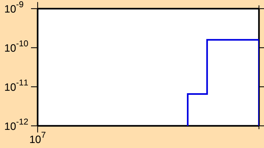
\sigma vs. E for ^{181}\text{Os}(n,\text{pd})
