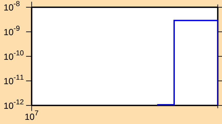
\sigma vs. E for ^{181}\text{Os}(n,\text{nt})
