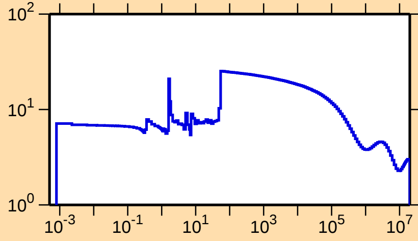
\sigma vs. E for ^{181}\text{Os}(n,\text{el.})
