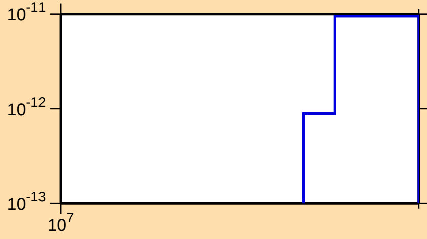
\sigma vs. E for ^{181}\text{Os}(\text{mt117})
