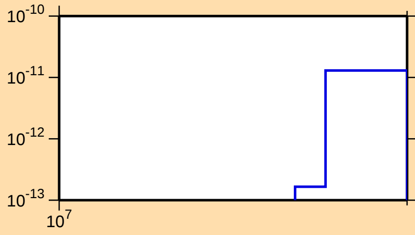
\sigma vs. E for ^{181}\text{Os}(n,\text{pt})
