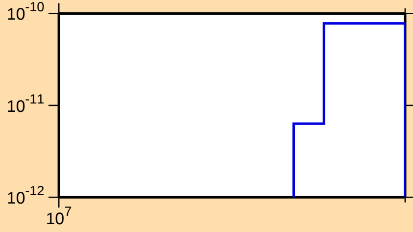
\sigma vs. E for ^{181}\text{Os} (mt 45)
