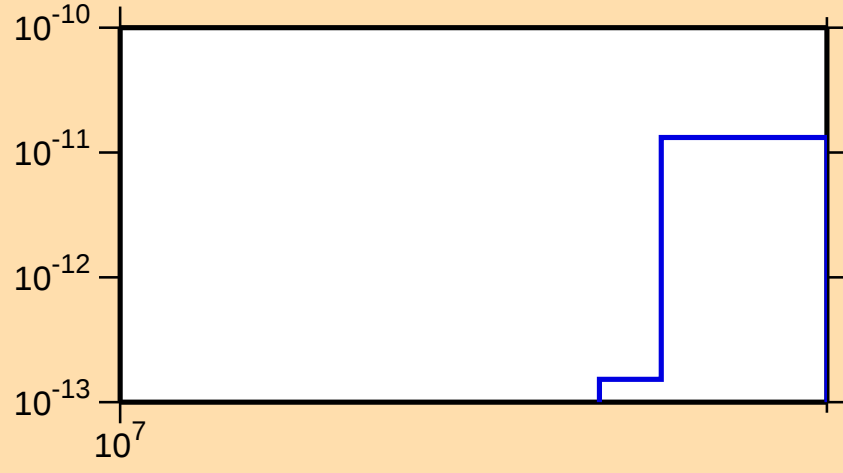
\sigma vs. E for ^{181}\text{Os} (mt 34)
