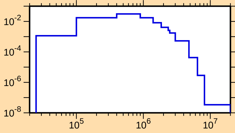
\sigma vs. E for ^{181}\text{Os}(n,n_2)
