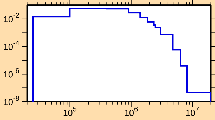
\sigma vs. E for ^{181}\text{Os}(n,n_3)
