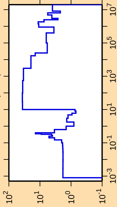
\Delta\sigma/\sigma vs. E for ^{181}\text{Os}(n,\text{el.})
