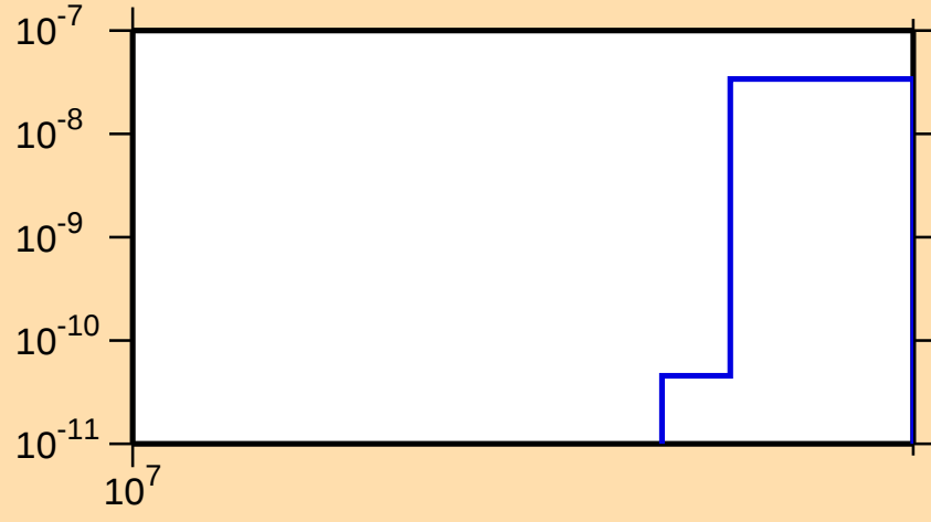
\sigma vs. E for ^{188}\text{Os}(n,nt)
