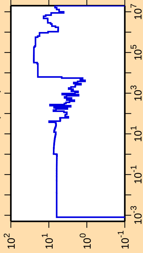
\Delta\sigma/\sigma vs. E for ^{188}\text{Os}(n,\text{el.})
