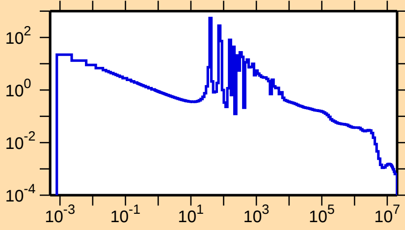
\sigma vs. E for ^{188}\text{Os}(n,\gamma)
