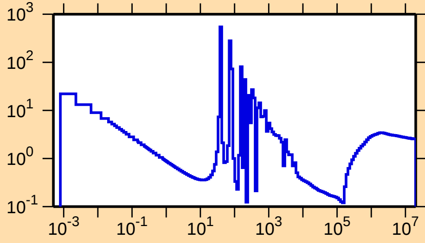
\sigma vs. E for ^{188}\text{Os}(n,\text{nonel.})
