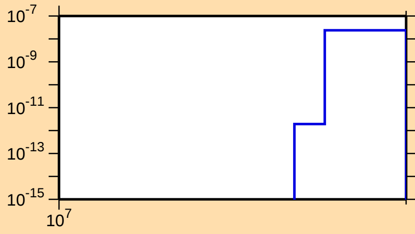
\sigma vs. E for ^{188}\text{Os}(n,2np)
