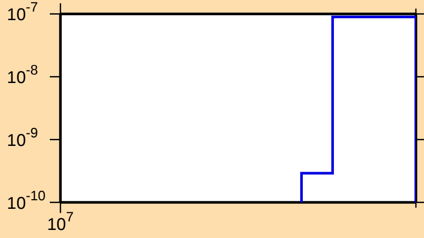
\sigma vs. E for ^{188}\text{Os}(n,\text{nd})
