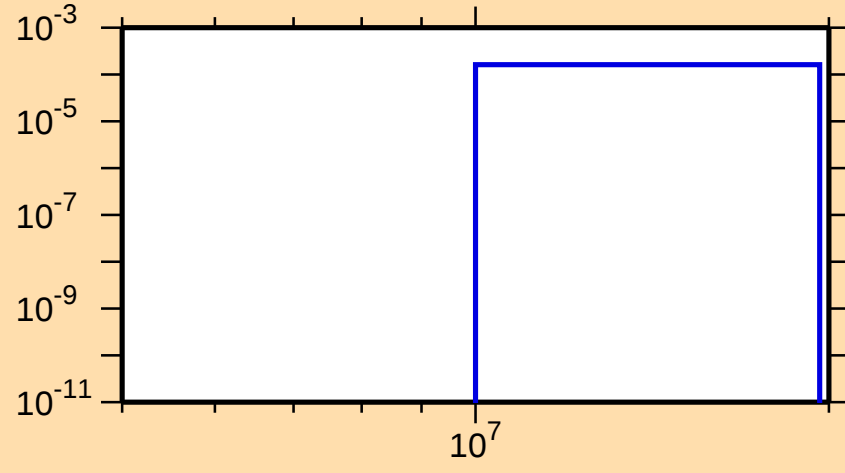
\sigma vs. E for ^{188}\text{Os}(n,np)
