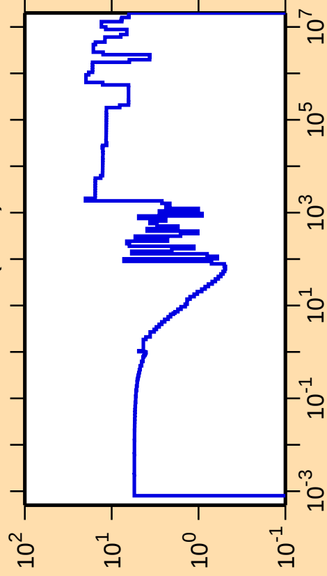
\Delta\sigma/\sigma vs. E for ^{190}\text{Os}(n,\text{el.})
