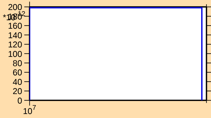
\sigma vs. E for ^{190}\text{Os}(n,\text{nd})
