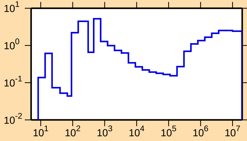
\sigma vs. E for ^{192}\text{Os}(n,\text{nonel.})
