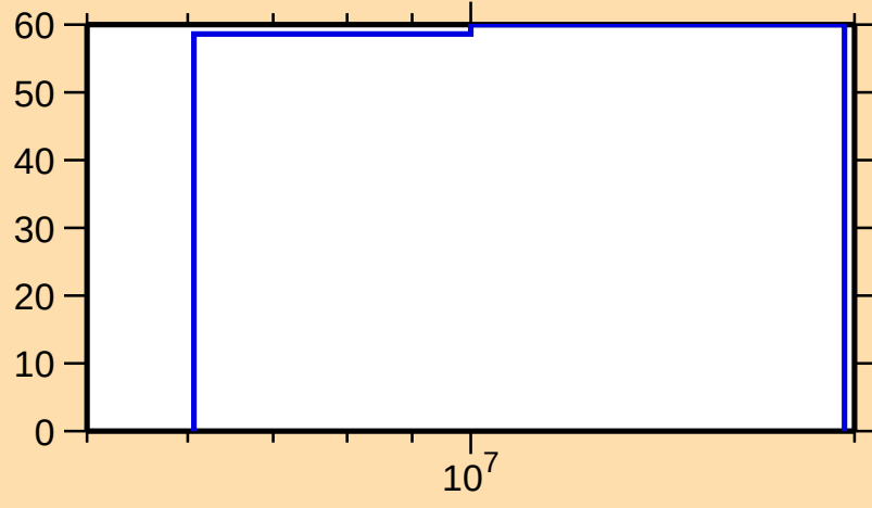
\Delta\sigma/\sigma vs. E for ^{192}\text{Os}(n,\gamma)
