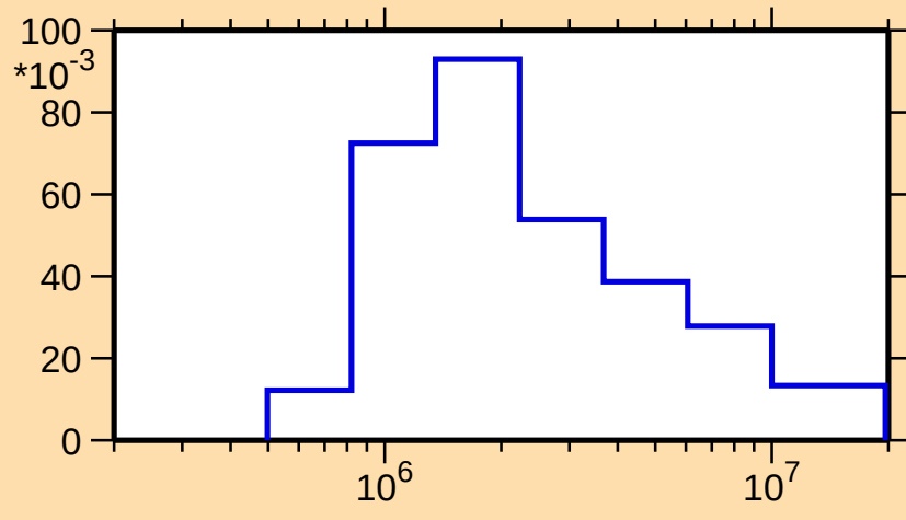
\sigma vs. E for ^{192}\text{Os}(n,n_3)
