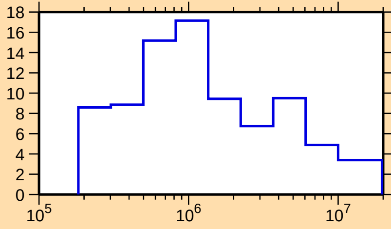
\Delta\sigma/\sigma vs. E for ^{192}\text{Os}(n,\text{tot.})
