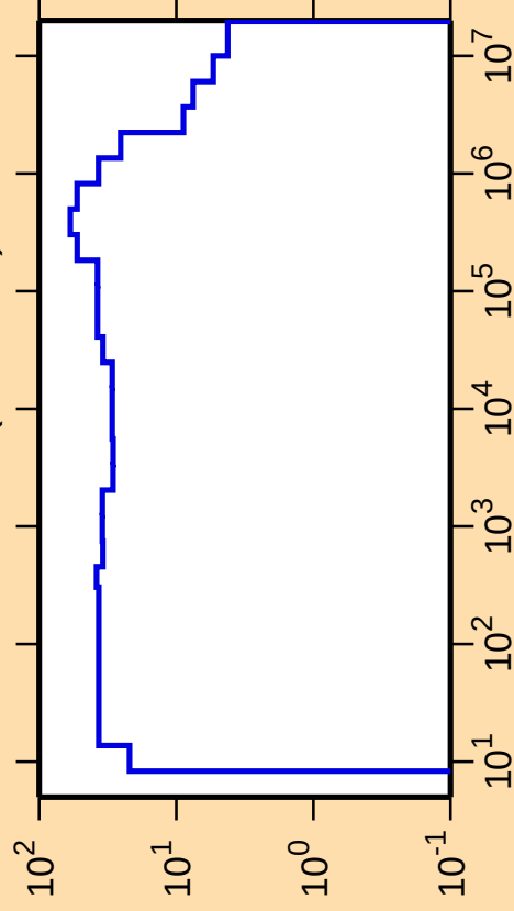
\Delta\sigma/\sigma vs. E for ^{192}\text{Os}(n,\text{nonel.})
