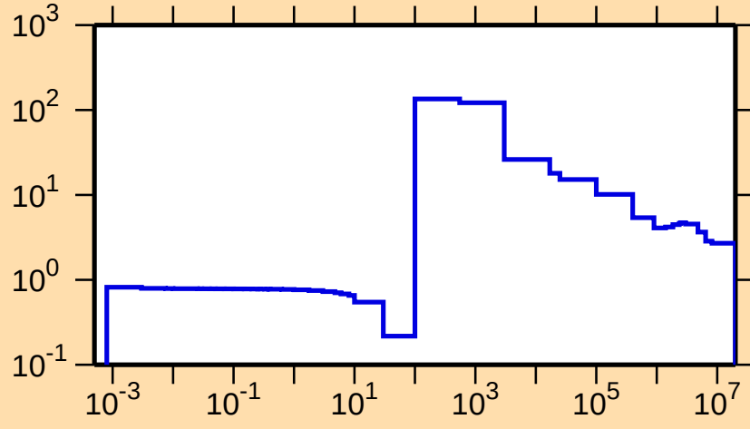
\sigma vs. E for ^{192}\text{Os}(n,\text{el.})
