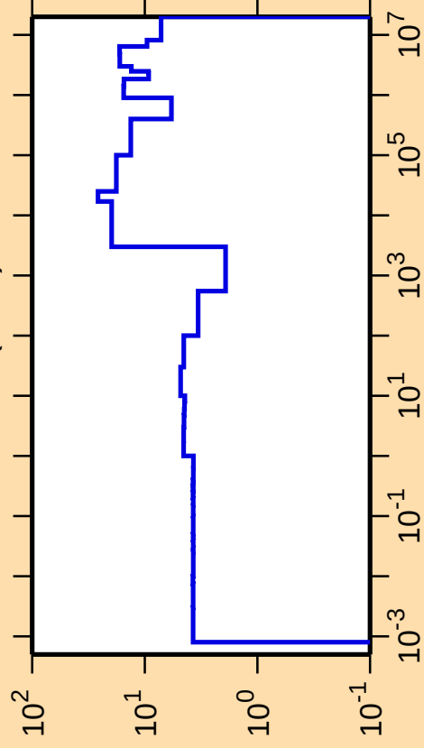
\Delta\sigma/\sigma vs. E for ^{192}\text{Os}(n,\text{el.})
