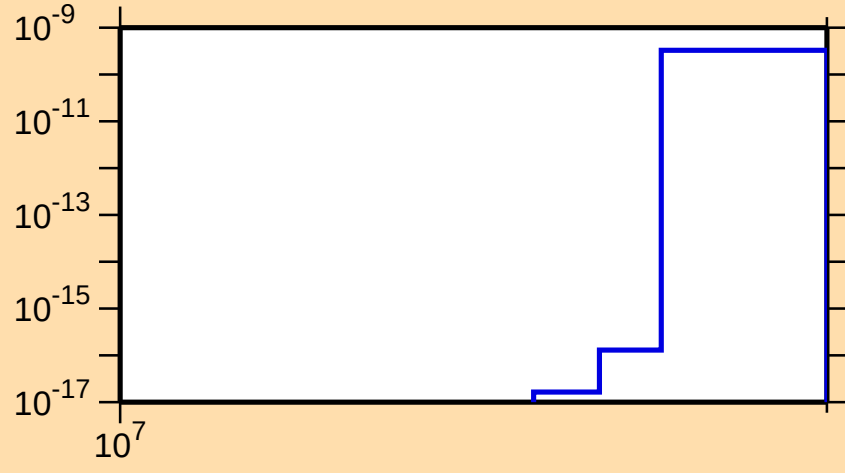
\sigma vs. E for ^{199}\text{Os}(n,2np)
