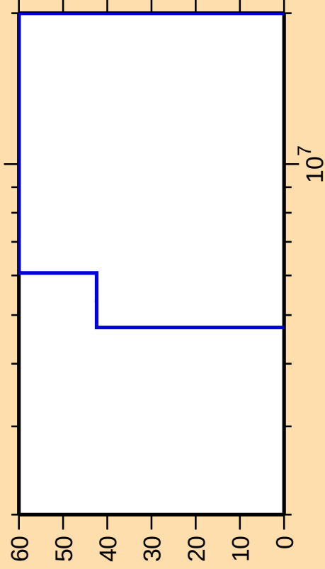
\Delta\sigma/\sigma vs. E for ^{199}\text{Os}(n,n\text{cont.})
