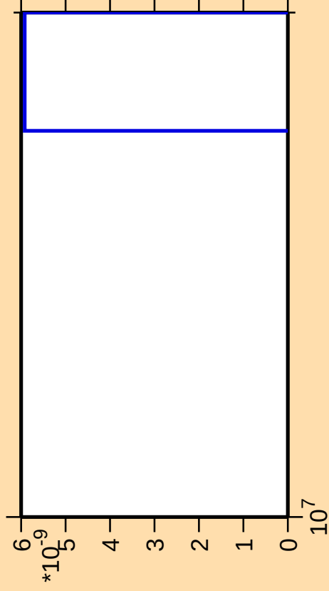
\Delta\sigma/\sigma vs. E for ^{199}\text{Os} (mt 11)
