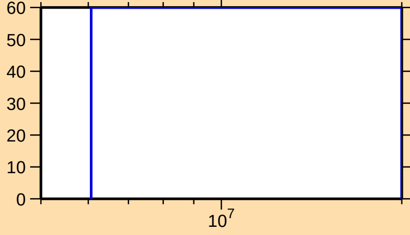
\Delta\sigma/\sigma vs. E for ^{199}\text{Os}(n,n\text{cont.})
