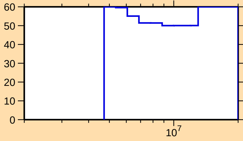
\Delta\sigma/\sigma vs. E for ^{199}\text{Os}(n,2n)
