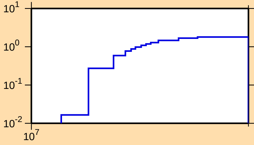
\sigma vs. E for ^{199}\text{Os}(n,3n)
