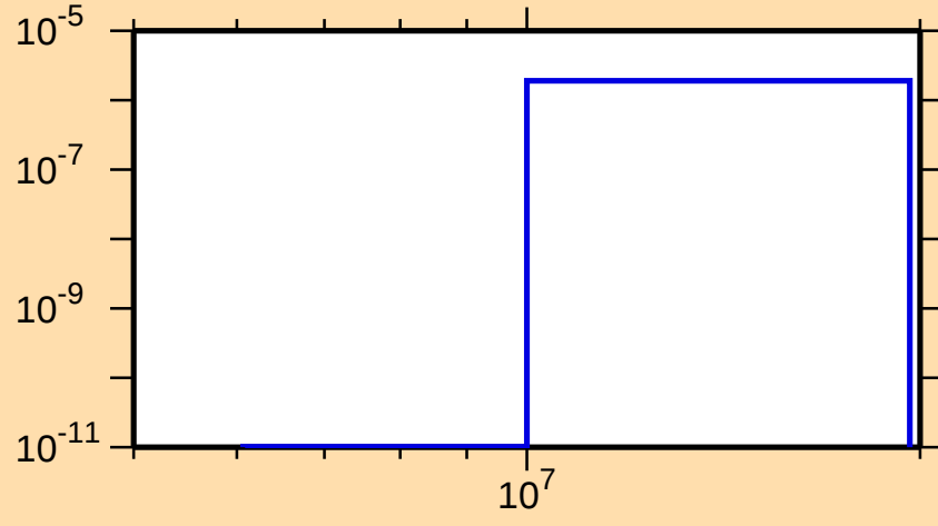
\sigma vs. E for ^{199}\text{Os}(n,\alpha)
