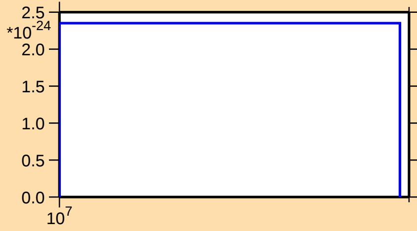
\sigma vs. E for ^{199}\text{Os} (mt 11)
