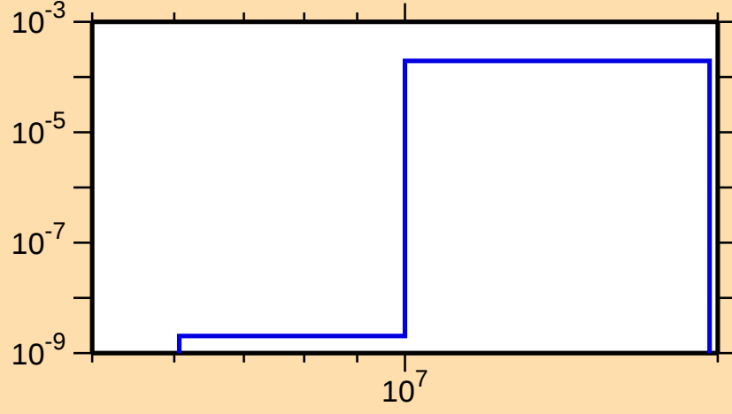
\sigma vs. E for ^{199}\text{Os}(n,p)
