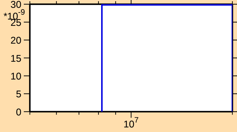
\sigma vs. E for ^{199}\text{Os}(n,n\alpha)
