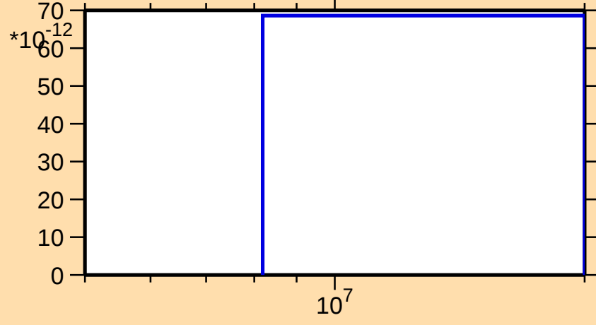
\sigma vs. E for ^{199}\text{Os}(n,\text{nd})
