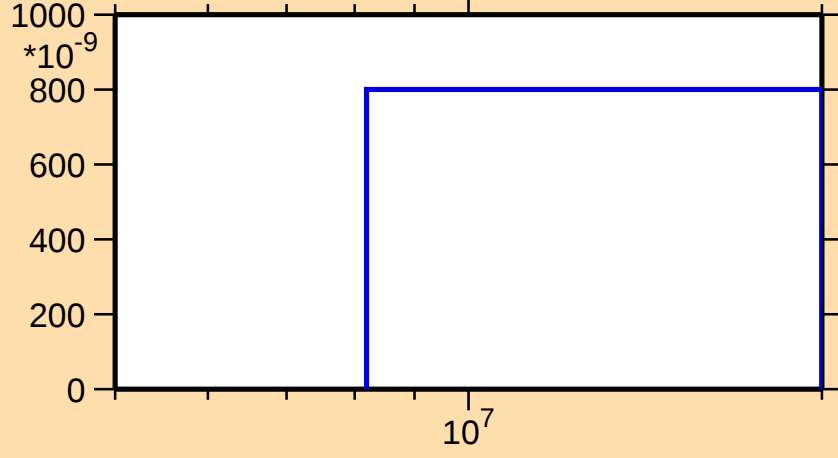
\sigma vs. E for ^{199}\text{Os}(n,t)
