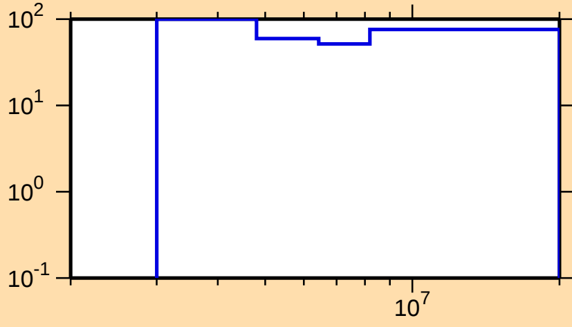
\Delta\sigma/\sigma vs. E for ^{199}\text{Os}(n,2n)
