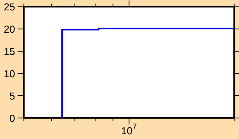
\Delta\sigma/\sigma vs. E for ^{199}\text{Os}(n,\text{nonel.})
