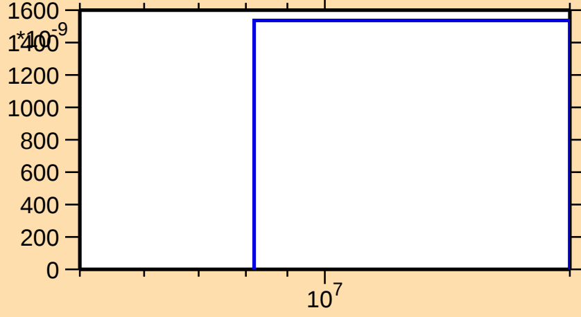
\sigma vs. E for ^{199}\text{Os}(n,d)
