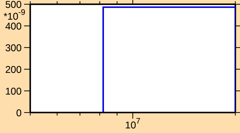
\sigma vs. E for ^{199}\text{Os}(n,np)
