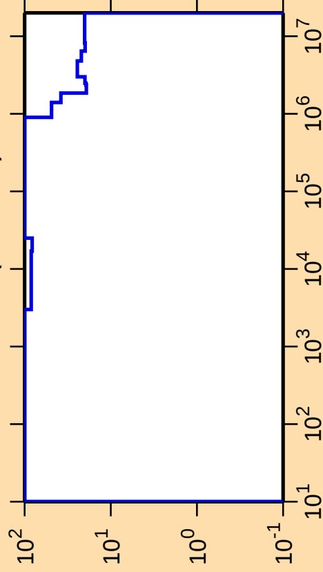
\Delta\sigma/\sigma vs. E for ^{199}\text{Os}(n,\text{nonel.})
