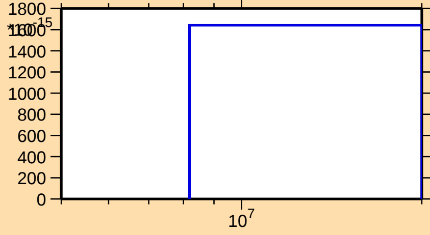
\sigma vs. E for ^{199}\text{Os}(n,2n\alpha)
