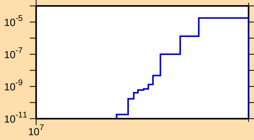
\sigma vs. E for ^{201}\text{Os}(n,d)
