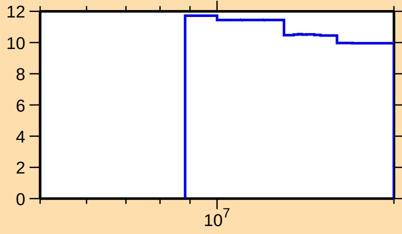
\Delta\sigma/\sigma vs. E for ^{201}\text{Os}(n,\text{nonel.})
