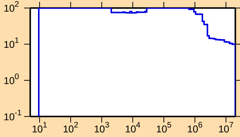
\Delta\sigma/\sigma vs. E for ^{201}\text{Os}(n,\text{nonel.})
