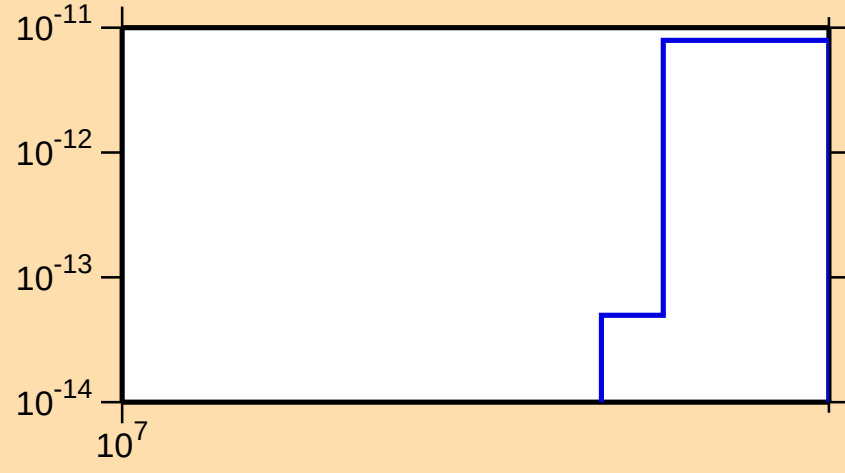
\sigma vs. E for ^{201}\text{Os}(n,2n\alpha)
