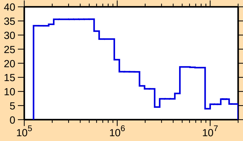
\Delta\sigma/\sigma vs. E for ^{201}\text{Os}(n,\text{el.})
