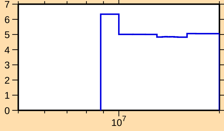
\Delta\sigma/\sigma vs. E for ^{201}\text{Os}(n,\text{tot.})
