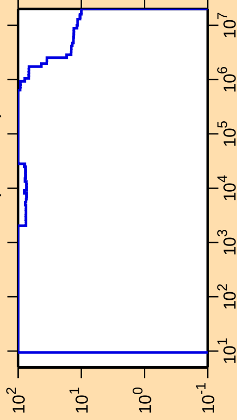
\Delta\sigma/\sigma vs. E for ^{201}\text{Os}(n,\text{nonel.})
