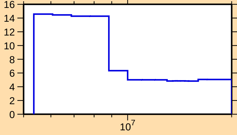
\Delta\sigma/\sigma vs. E for ^{201}\text{Os}(n,\text{tot.})
