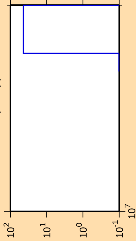
\Delta\sigma/\sigma vs. E for ^{201}\text{Os}(n,2np)
