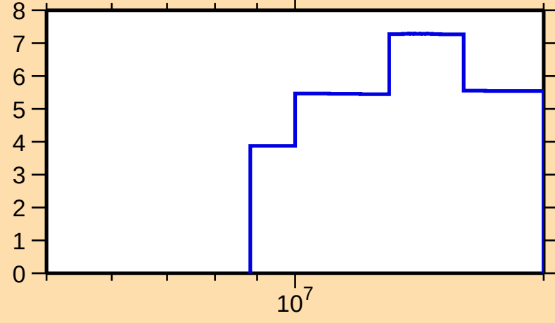
\Delta\sigma/\sigma vs. E for ^{201}\text{Os}(n,\text{el.})
