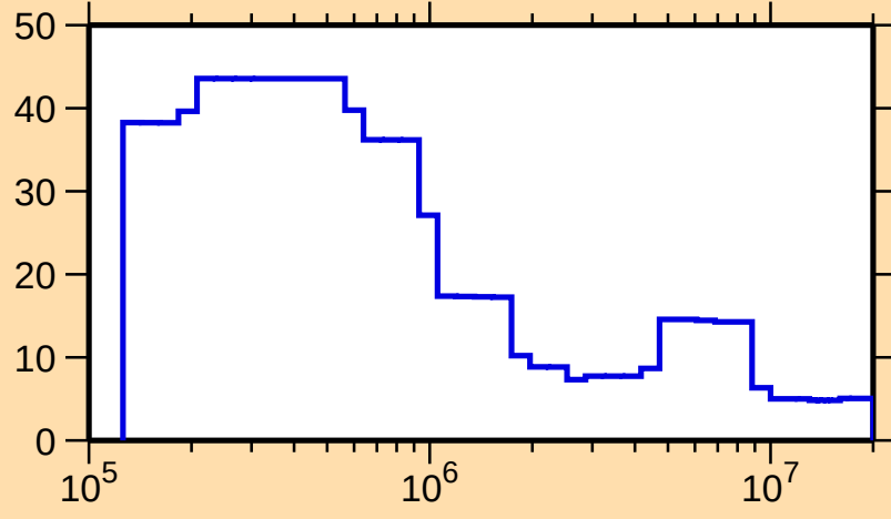
\Delta\sigma/\sigma vs. E for ^{201}\text{Os}(n,\text{tot.})
