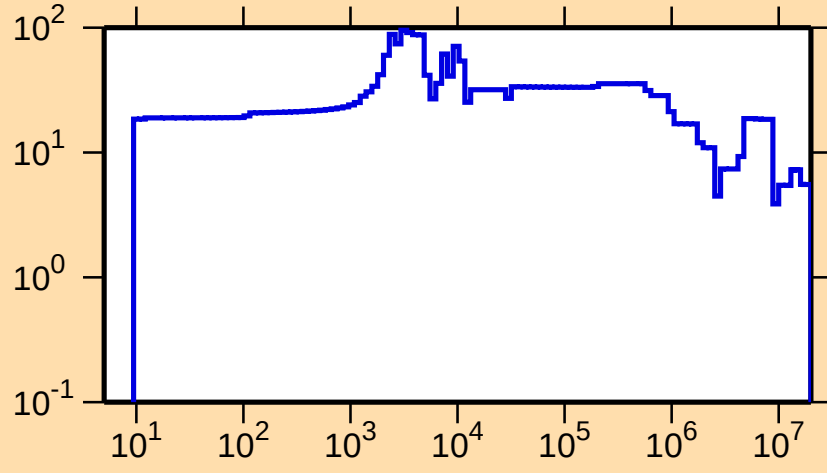
\Delta\sigma/\sigma vs. E for ^{201}\text{Os}(n,\text{el.})
