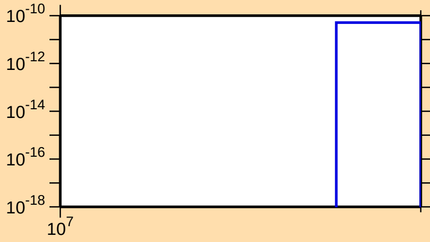
\sigma vs. E for ^{201}\text{Os}(n,2np)
