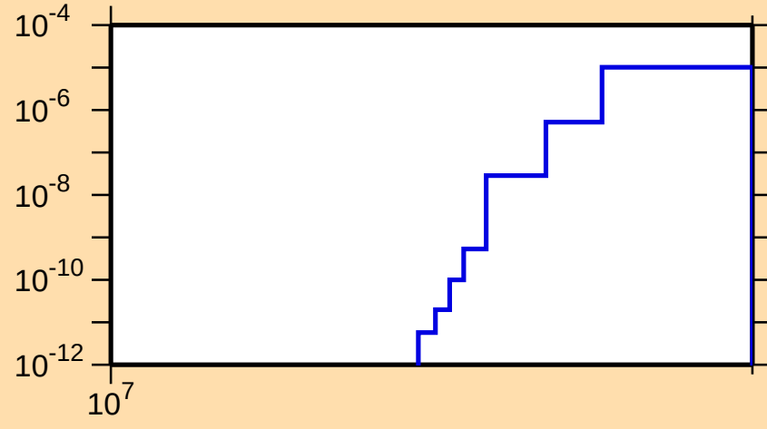
\sigma vs. E for ^{201}\text{Os}(n,np)
