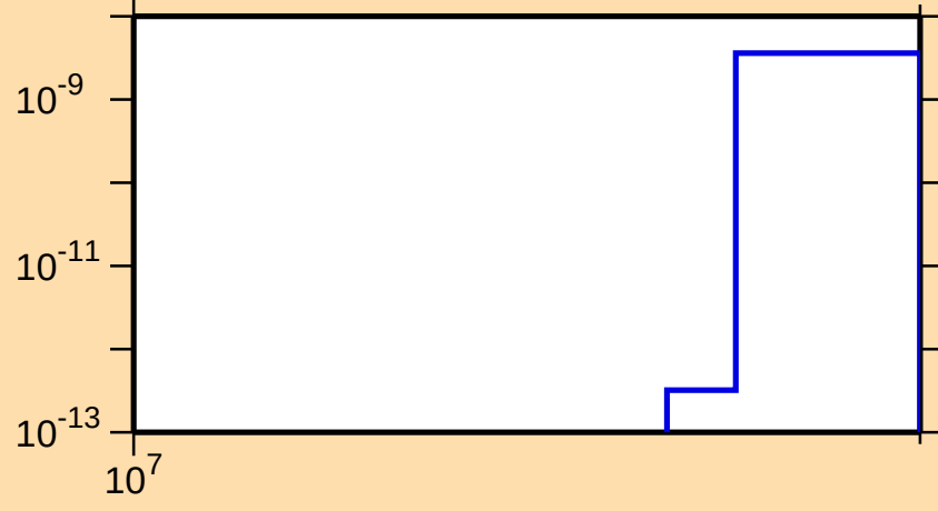
\sigma vs. E for ^{201}\text{Os}(n,nt)
