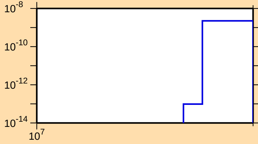
\sigma vs. E for ^{201}\text{Os}(n,\text{nd})
