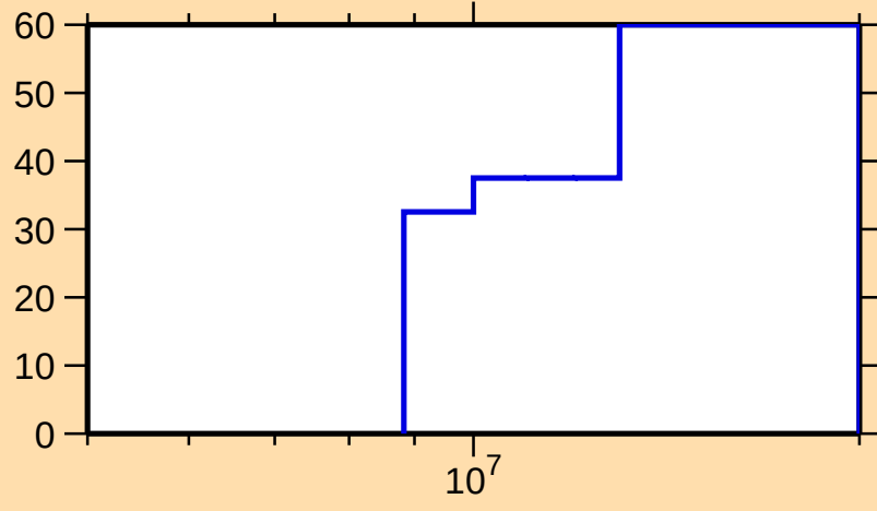
\Delta\sigma/\sigma vs. E for ^{201}\text{Os}(n,2n)
