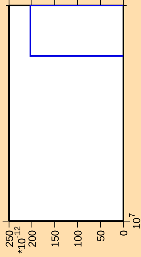
\Delta\sigma/\sigma vs. E for ^{201}\text{Os}(\text{mt } 11)
