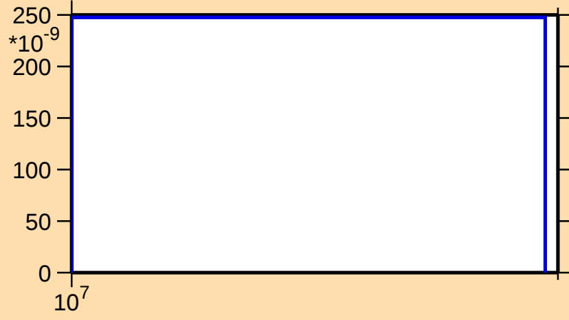
\sigma vs. E for ^{201}\text{Os}(n,d)
