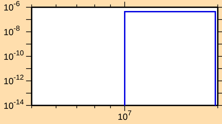
\sigma vs. E for ^{201}\text{Os}(n,t)
