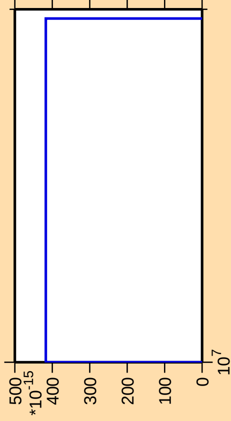
\Delta\sigma/\sigma vs. E for ^{201}\text{Os} (mt 11)
