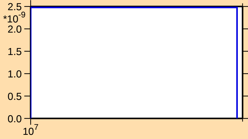
\sigma vs. E for ^{201}\text{Os}(n,n\alpha)
