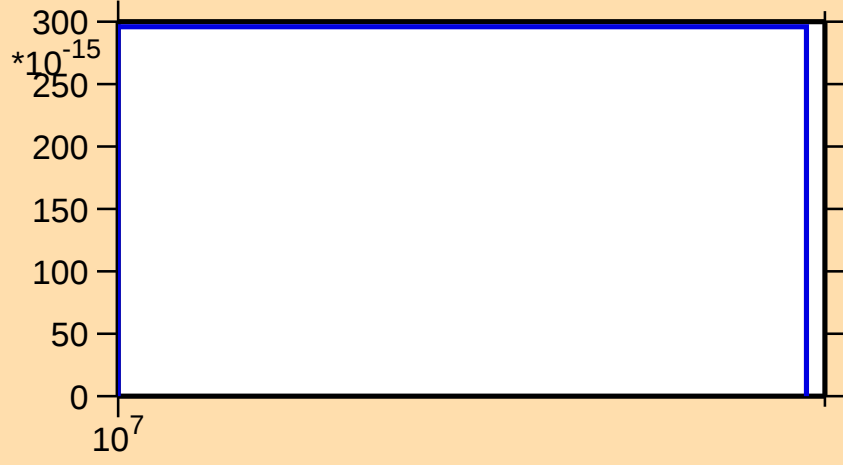
\sigma vs. E for ^{201}\text{Os}(n,2np)
