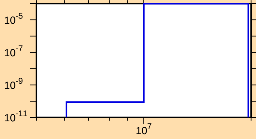
\sigma vs. E for ^{201}\text{Os}(n,p)
