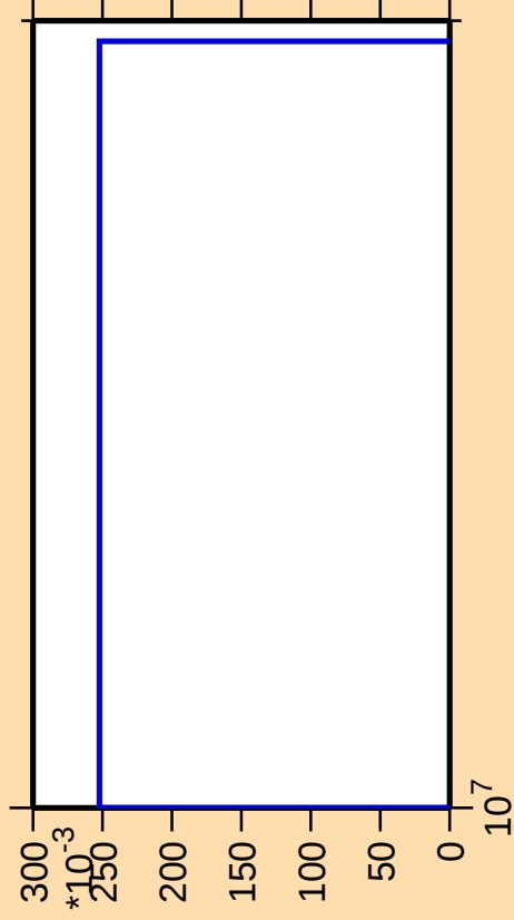
\Delta\sigma/\sigma vs. E for ^{201}\text{Os}(n,2np)
