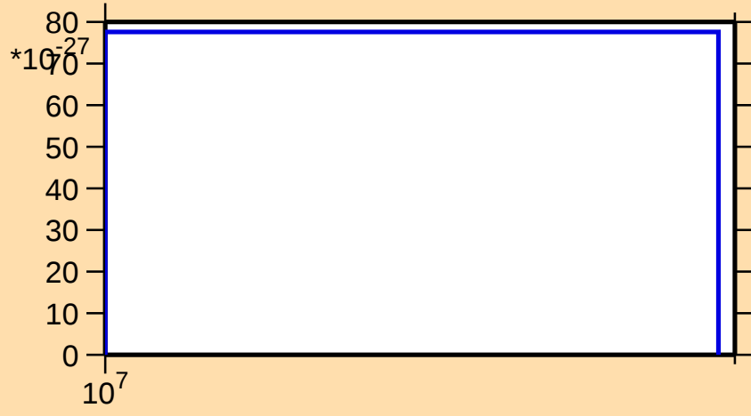
\sigma vs. E for ^{201}\text{Os} (mt 11)
