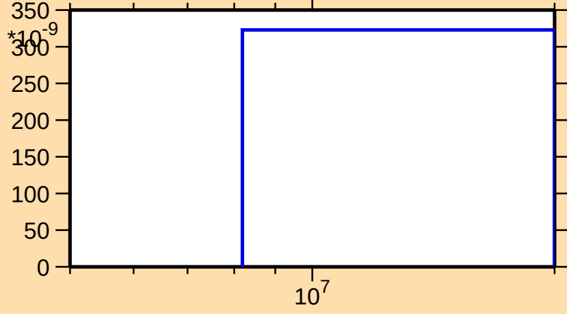
\sigma vs. E for ^{201}\text{Os}(n,\alpha)
