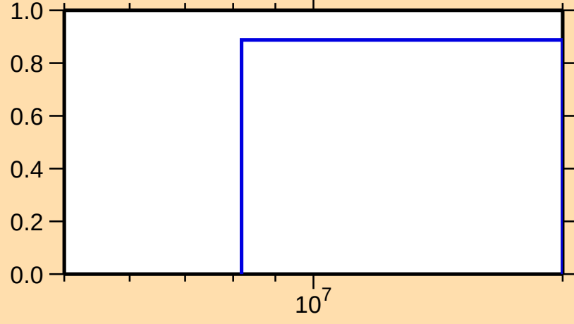
\sigma vs. E for ^{201}\text{Os}(n,3n)
