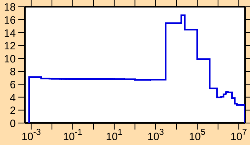
\sigma vs. E for ^{201}\text{Os}(n,\text{el.})
