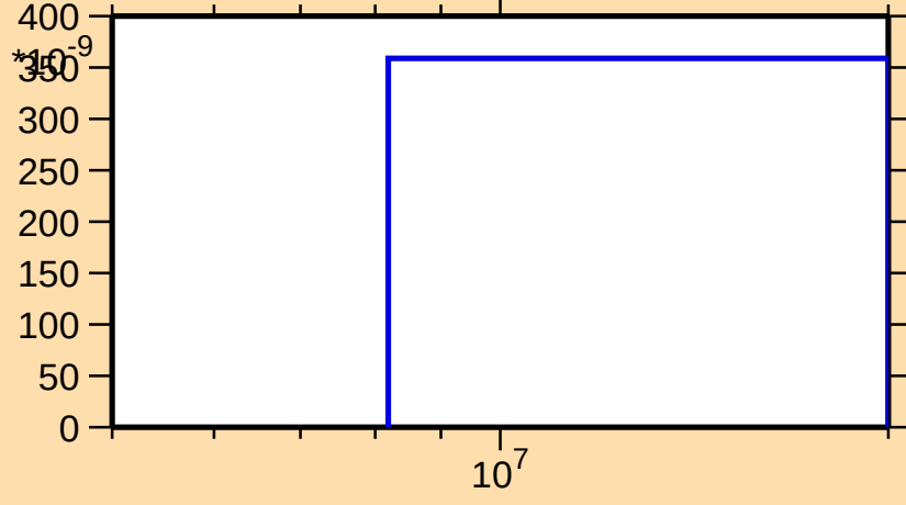
\sigma vs. E for ^{201}\text{Os}(n,t)
