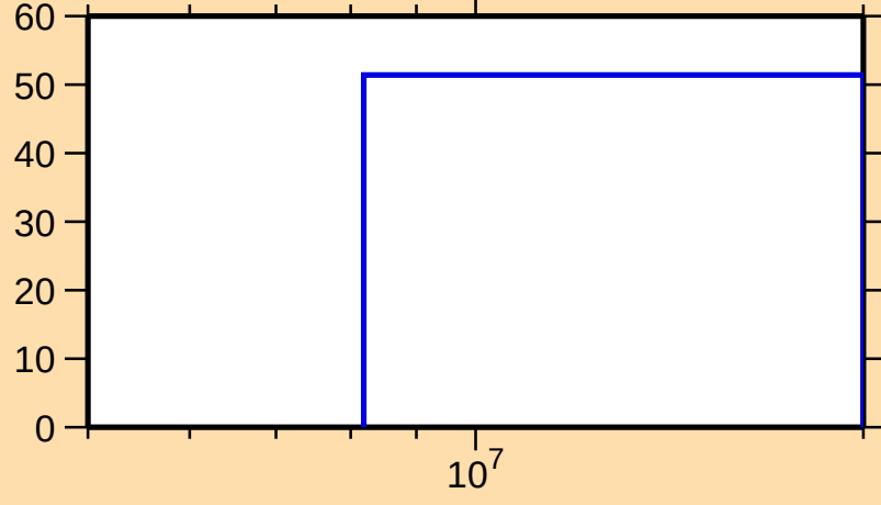
\Delta\sigma/\sigma vs. E for ^{201}\text{Os}(n,2n)
