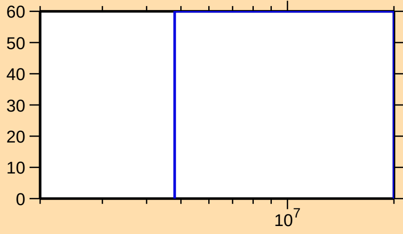
\Delta\sigma/\sigma vs. E for ^{201}\text{Os}(n,n\text{cont.})
