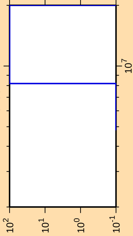
\Delta\sigma/\sigma vs. E for ^{201}\text{Os}(n,p)
