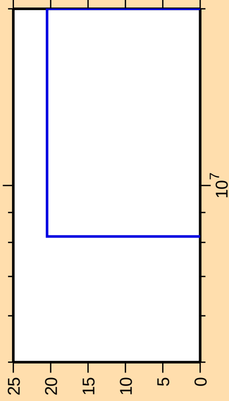
\Delta\sigma/\sigma vs. E for ^{201}\text{Os}(n,3n)
