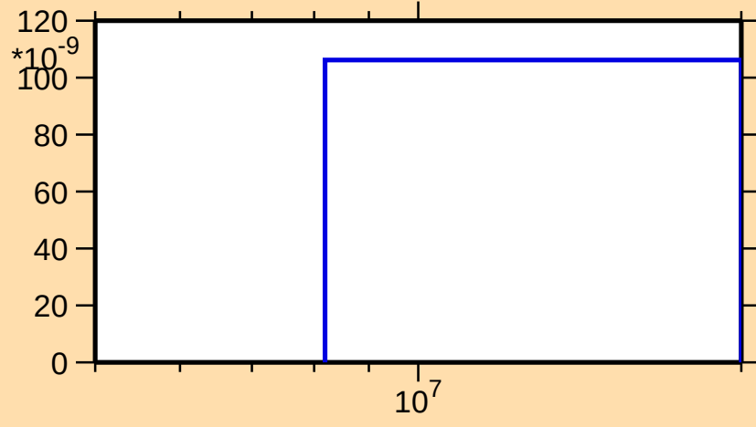
\sigma vs. E for ^{201}\text{Os}(n,np)
