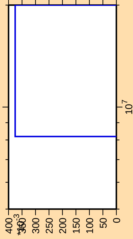
\Delta\sigma/\sigma vs. E for ^{201}\text{Os}(n,2n\alpha)
