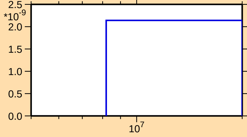
\sigma vs. E for ^{201}\text{Os}(n,n\alpha)
