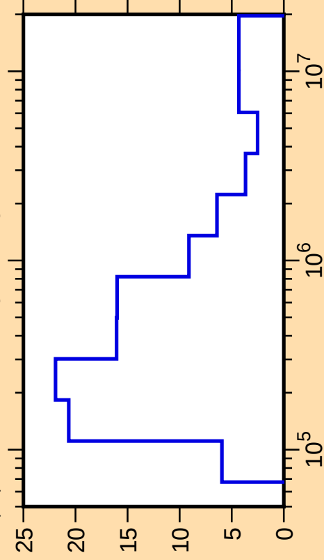
\Delta\mu/\mu vs. E for ^{31}\text{P}(\text{mt251})
