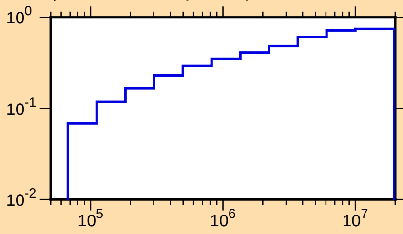
\mu vs. E for ^{31}\text{P}(\text{mt251})
