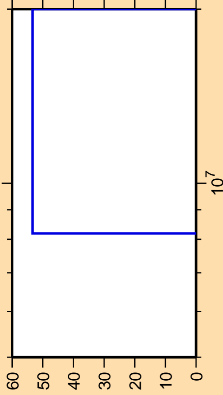
\Delta\sigma/\sigma vs. E for ^{33}\text{P}(n,t)
