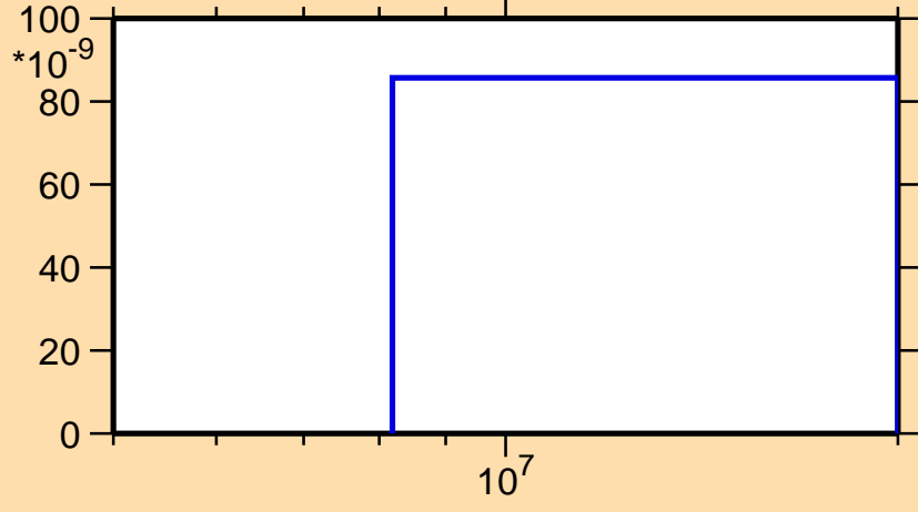
\sigma vs. E for ^{33}\text{P}(n,\text{nd})
