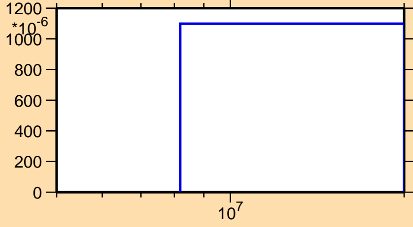
\sigma vs. E for ^{33}\text{P}(n,n\alpha)
