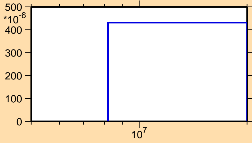
\sigma vs. E for ^{33}\text{P}(n,t)
