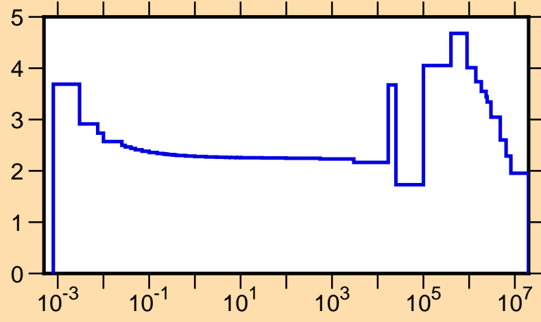
\sigma vs. E for ^{33}\text{P}(n,\text{tot.})
