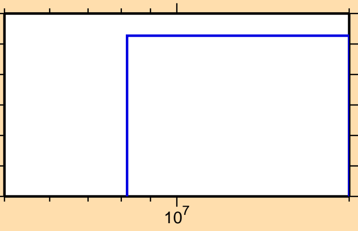
\sigma vs. E for ^{33}\text{P}(n,np)
