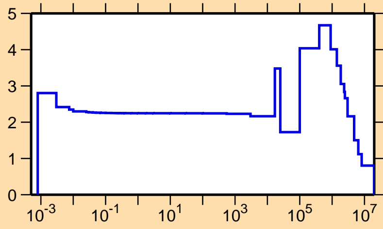
\sigma vs. E for ^{33}\text{P}(n,\text{el.})
