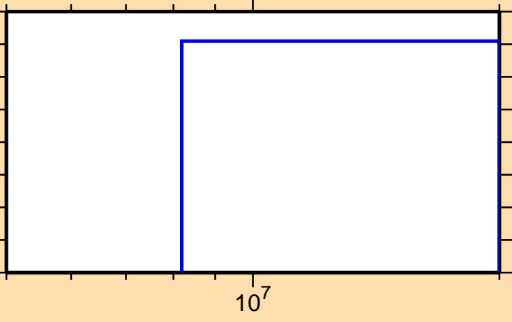
\sigma vs. E for ^{33}\text{P}(n,nt)
