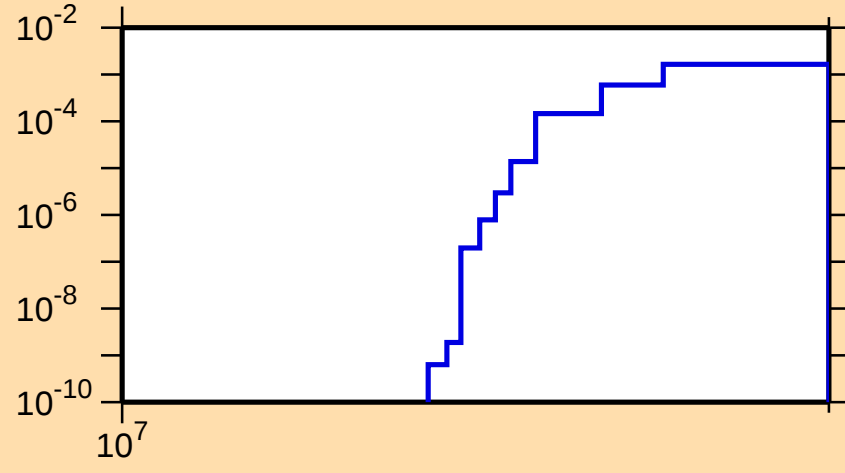
\sigma vs. E for ^{36}\text{P}(n,np)
