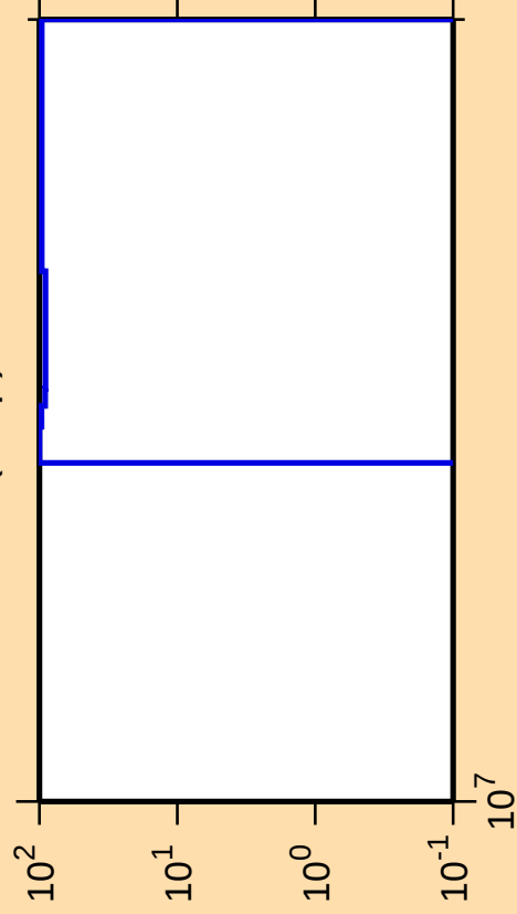
\Delta\sigma/\sigma vs. E for ^{36}\text{P}(n,np)
