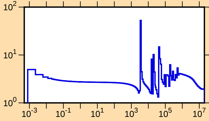
\sigma vs. E for ^{36}\text{P}(n,\text{tot.})
