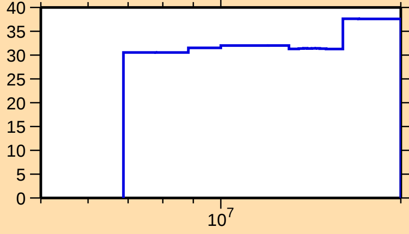
\Delta\sigma/\sigma vs. E for ^{36}\text{P}(n,2n)
