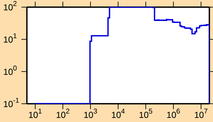
\Delta\sigma/\sigma vs. E for ^{36}\text{P}(n,\text{nonel.})
