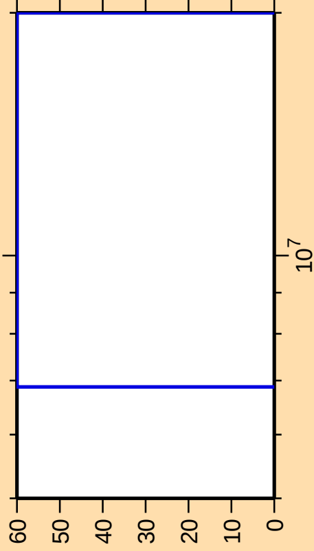
\Delta\sigma/\sigma vs. E for ^{36}\text{P}(\text{n,p})
