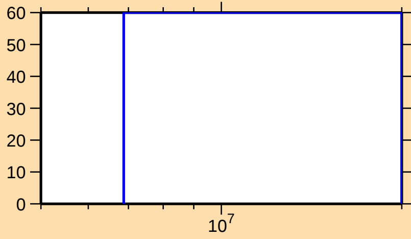
\Delta\sigma/\sigma vs. E for ^{36}\text{P}(\text{n,ncont.})
