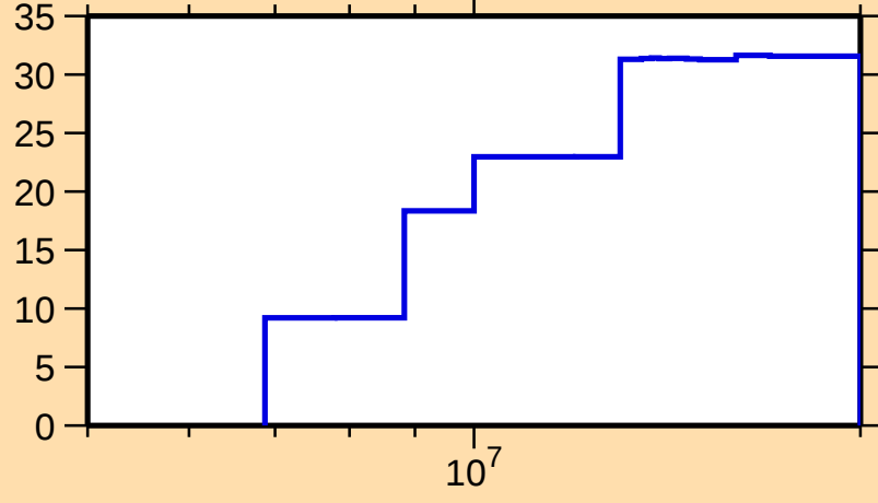
\Delta\sigma/\sigma vs. E for ^{36}\text{P}(\text{n,el.})
