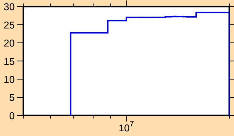
\Delta\sigma/\sigma vs. E for ^{36}\text{P}(n,\text{nonel.})
