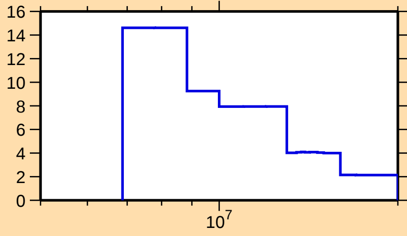
\Delta\sigma/\sigma vs. E for ^{36}\text{P}(n,\text{tot.})
