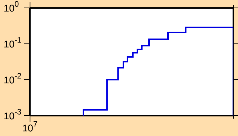
\sigma vs. E for ^{36}\text{P}(n,3n)
