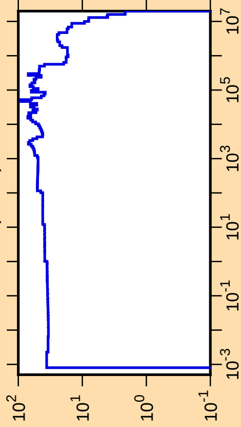
\Delta\sigma/\sigma vs. E for ^{36}\text{P}(n,\text{tot.})
