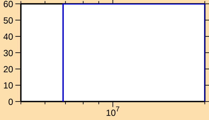
\Delta\sigma/\sigma vs. E for ^{36}\text{P}(n,\gamma)
