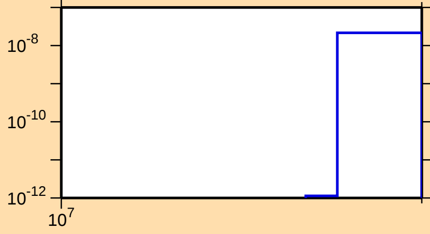
\sigma vs. E for ^{36}\text{P}(n,2n\alpha)
