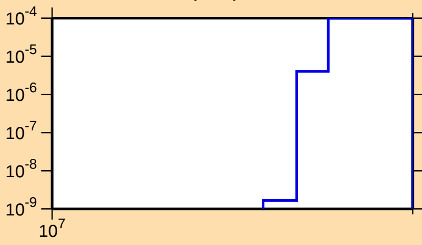
\sigma vs. E for ^{36}\text{P}(\text{n},\text{nt})
