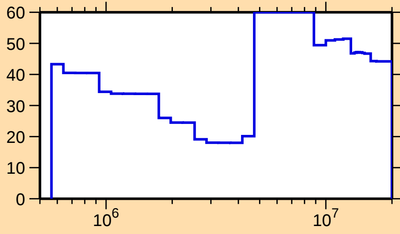
\Delta\sigma/\sigma vs. E for ^{36}\text{P}(n,\text{inel.})
