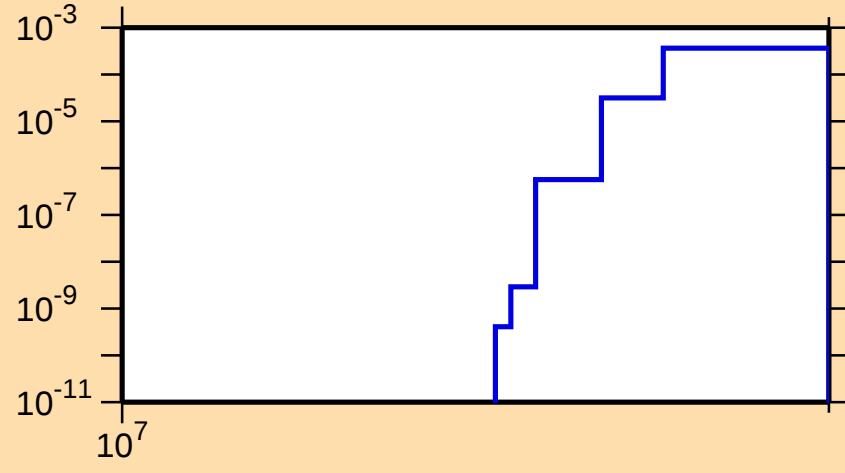
\sigma vs. E for ^{36}\text{P}(\text{n},\text{nd})
