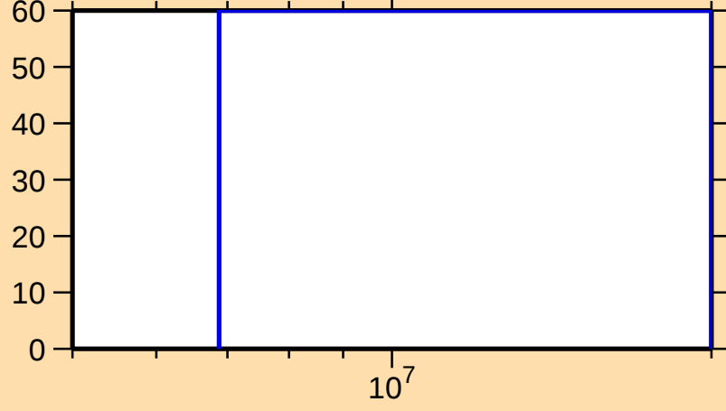
\Delta\sigma/\sigma vs. E for ^{36}\text{P}(n,n_1)
