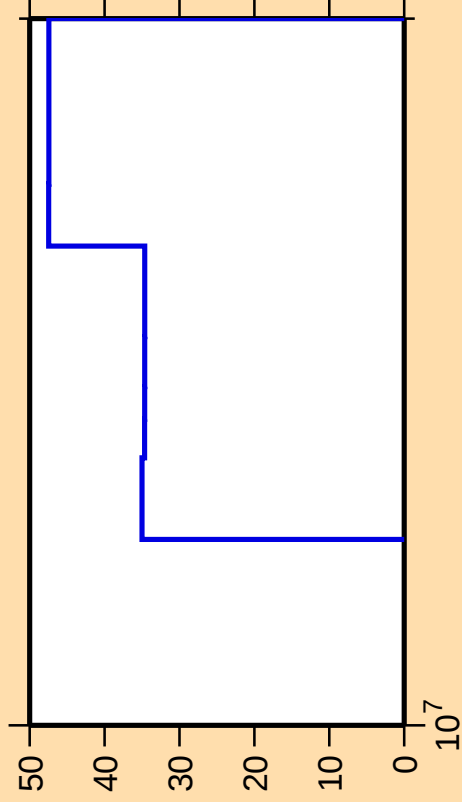
\Delta\sigma/\sigma vs. E for ^{36}\text{P}(n,3n)
