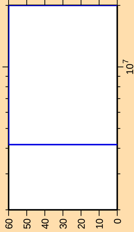
\Delta\sigma/\sigma vs. E for ^{36}\text{P}(n,\gamma)
