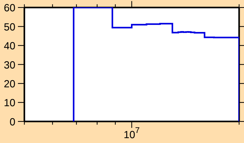
\Delta\sigma/\sigma vs. E for ^{36}\text{P}(\text{n,inel.})
