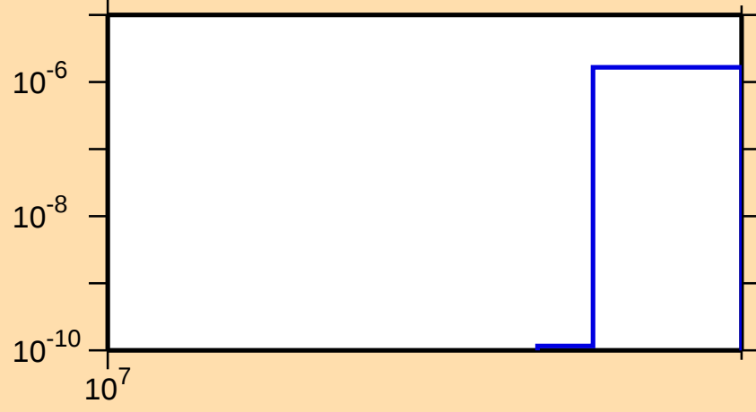
\sigma vs. E for ^{36}\text{P}(n,2np)
