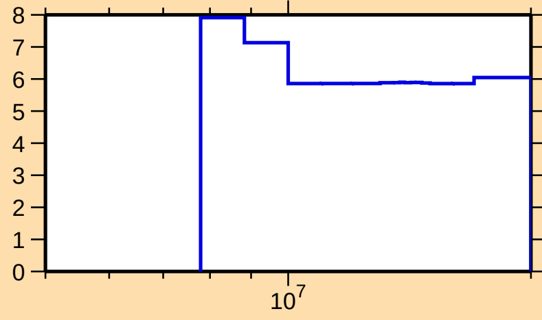
\Delta\sigma/\sigma vs. E for ^{37}\text{P}(\text{n},\text{nonel.})
