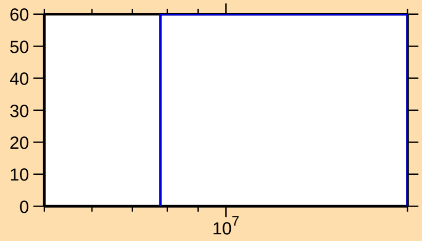
\Delta\sigma/\sigma vs. E for ^{37}\text{P}(n,n\text{cont.})
