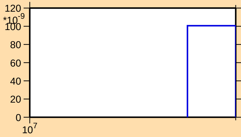
\sigma vs. E for ^{37}\text{P}(\text{n},\text{nd})
