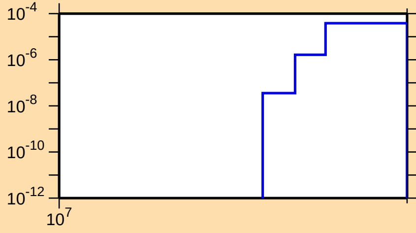
\sigma vs. E for ^{37}\text{P}(\text{n},\text{nt})
