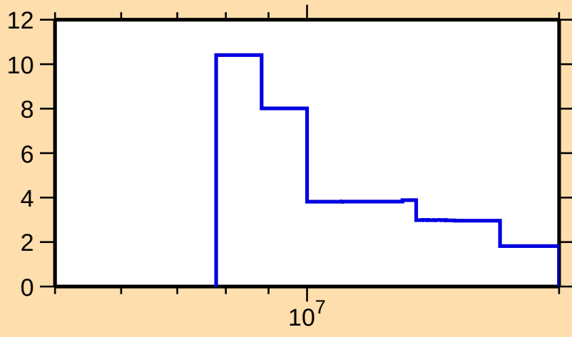
\Delta\sigma/\sigma vs. E for ^{37}\text{P}(\text{n,tot.})
