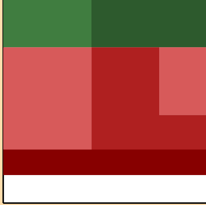
\Delta\sigma/\sigma vs. E for ^{37}\text{P}(n,\text{el.})
