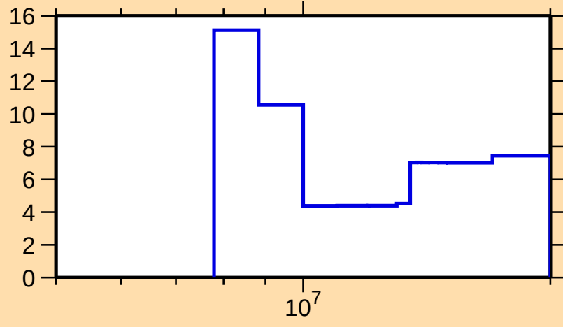
\Delta\sigma/\sigma vs. E for ^{37}\text{P}(\text{n},\text{el.})
