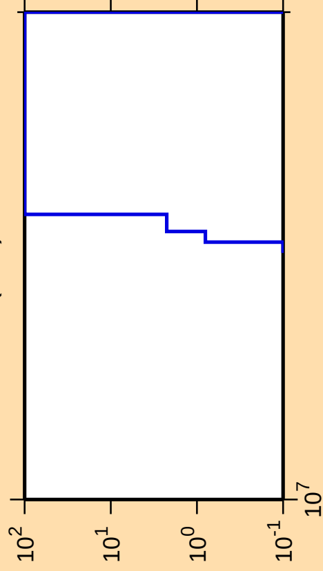
\Delta\sigma/\sigma vs. E for ^{37}\text{P}(\text{n},\text{nt})
