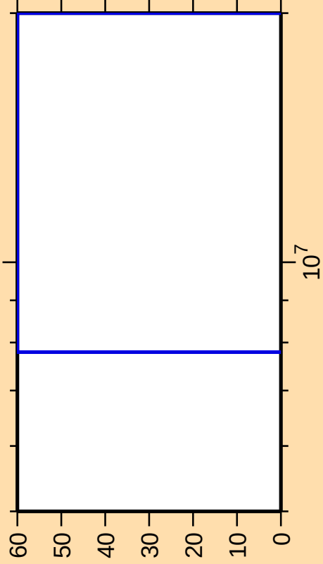
\Delta\sigma/\sigma vs. E for ^{37}\text{P}(\text{n},\text{ncont.})
