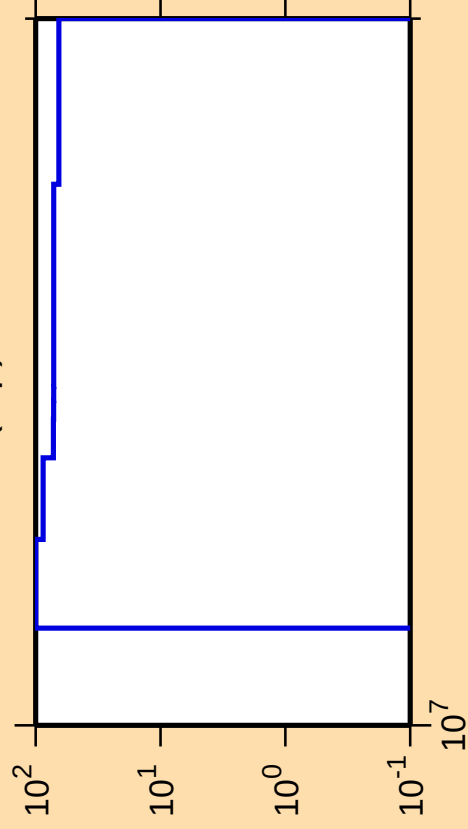
\Delta\sigma/\sigma vs. E for ^{37}\text{P}(\text{n,p})
