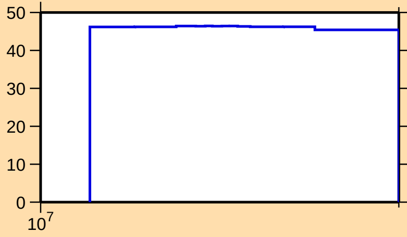
\Delta\sigma/\sigma vs. E for ^{37}\text{P}(\text{n,inel.})
