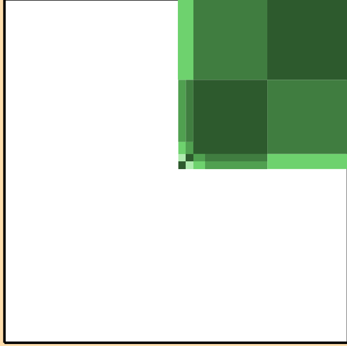
\sigma vs. E for ^{37}\text{P}(n,np)
