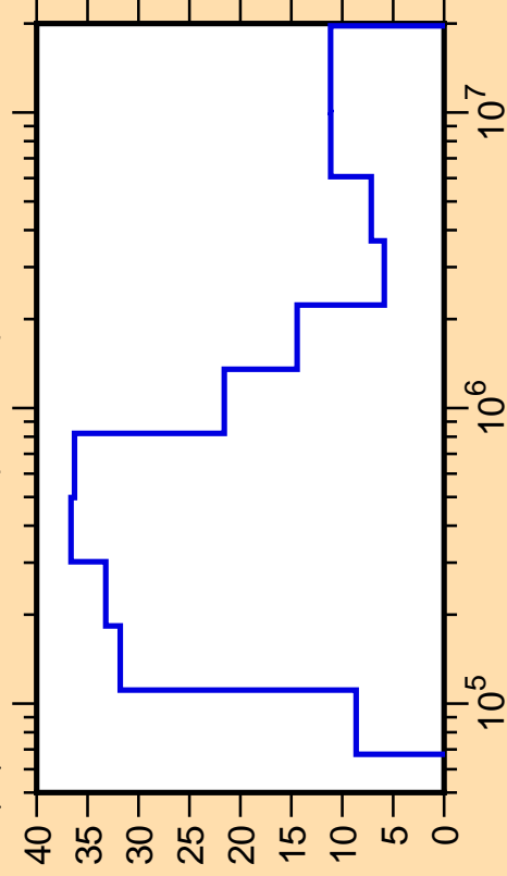
\Delta\mu/\mu vs. E for ^{37}\text{P}(\text{mt251})
