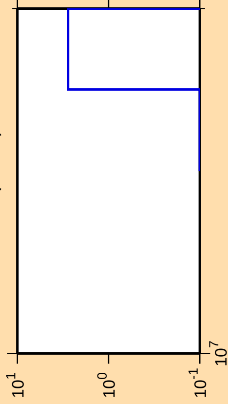
\Delta\sigma/\sigma vs. E for ^{229}\text{Pa}(\text{mt } 11)
