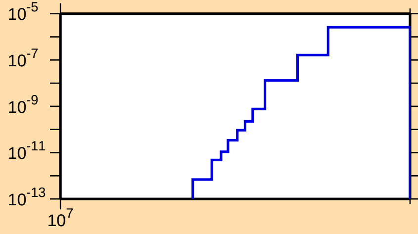
\sigma vs. E for ^{229}\text{Pa}(n,\text{nd})
