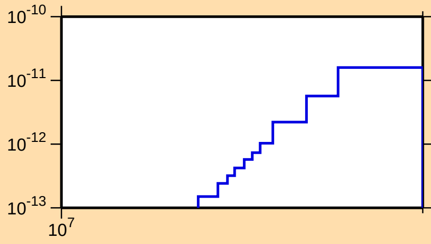
\sigma vs. E for ^{229}\text{Pa}(n,p\alpha)
