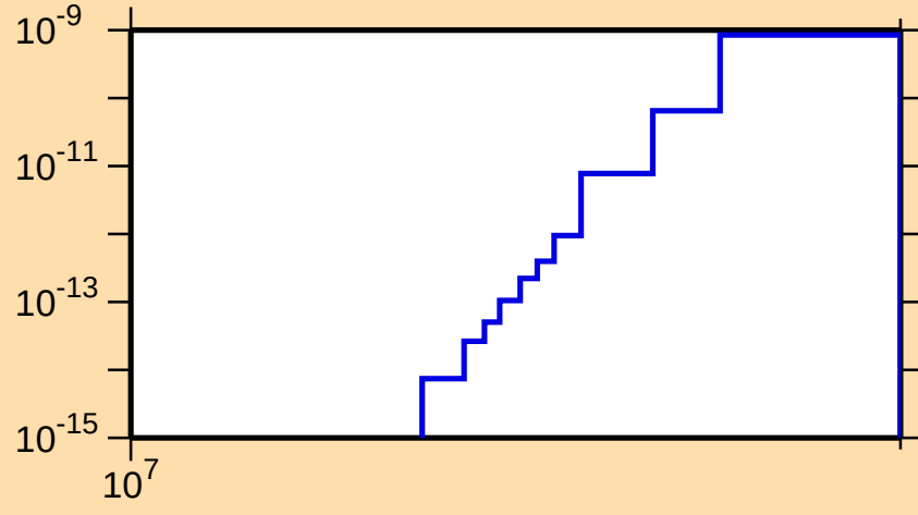
\sigma vs. E for ^{229}\text{Pa}(n,\text{He}3)
