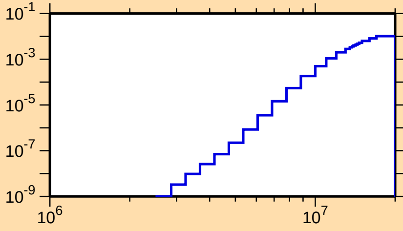
\sigma vs. E for ^{229}\text{Pa}(n,p)
