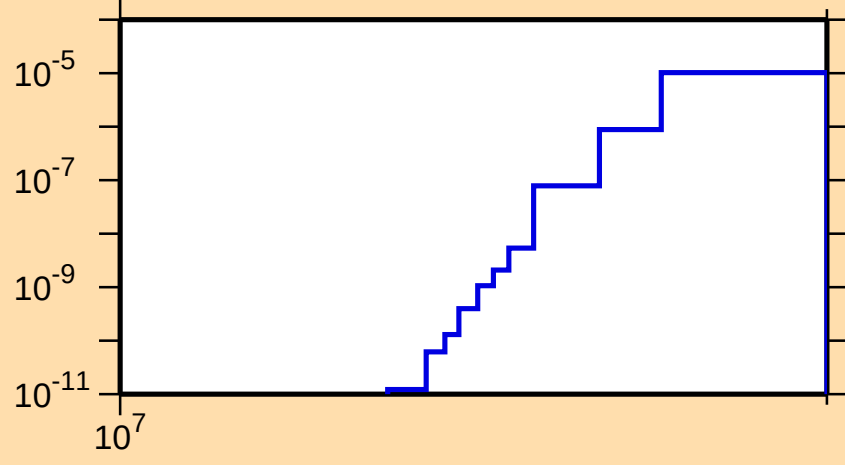
\sigma vs. E for ^{229}\text{Pa}(n,nt)
