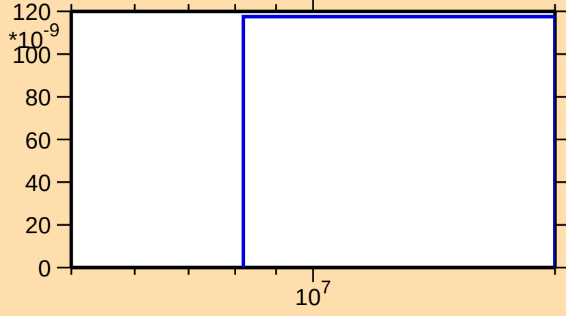
\sigma vs. E for ^{229}\text{Pa}(n,2n\alpha)
