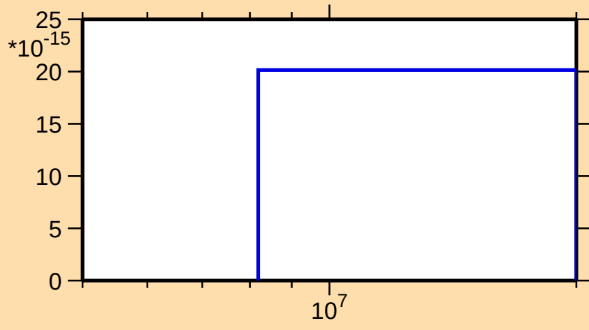
\sigma vs. E for ^{229}\text{Pa}(\text{mt 11})
