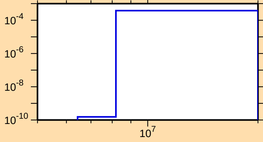
\sigma vs. E for ^{229}\text{Pa}(n,np)
