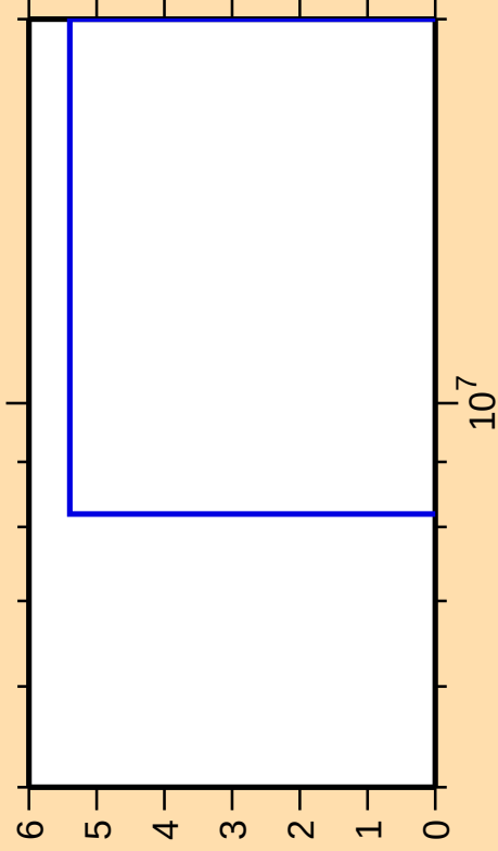
\Delta\sigma/\sigma vs. E for ^{229}\text{Pa}(\text{mt } 45)
