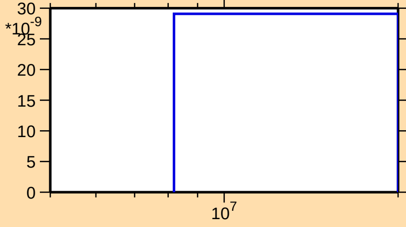
\sigma vs. E for ^{229}\text{Pa}(n,\text{nd})
