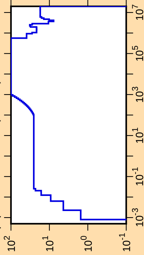
\Delta\mu/\mu vs. E for ^{234}\text{Pa}(\text{mt251})
