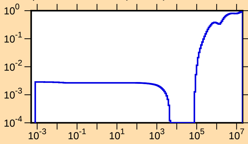
\mu vs. E for ^{234}\text{Pa}(\text{mt251})
